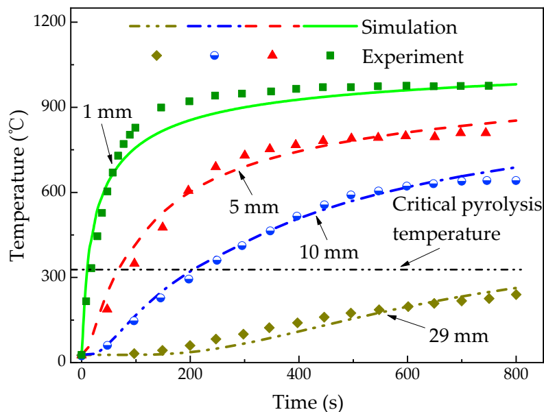
Figure 4. Temperature profiles of the glass fiber/phenolic resin composites under one-sided heating.
