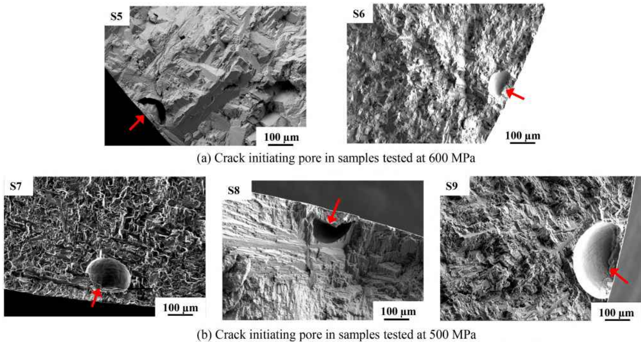
Fig. 8. SEM images of fracture surfaces showing the crack initiating defect (indicated with an arrow) for samples tested at 600 and 500 MPa.
