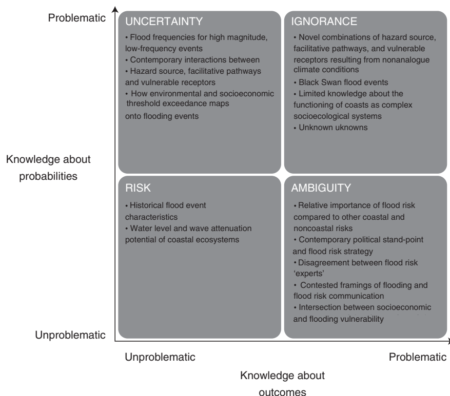
FIGURE 3 Flood events in the context of incertitude. This figure applies Stirling's (2007) categorization of incomplete knowledge states to flooding
