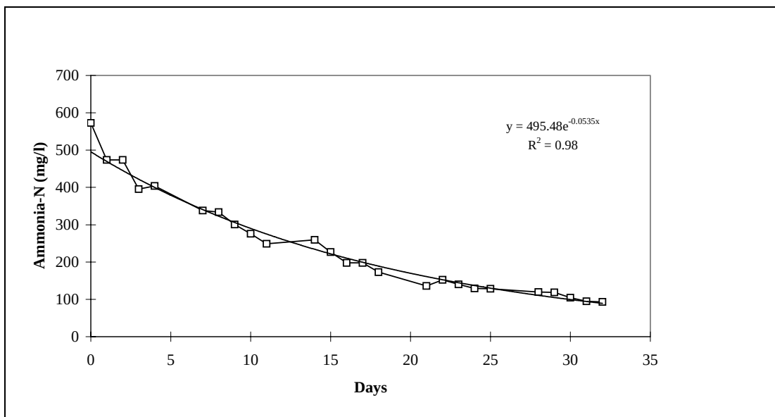
Figure 4 A typical example of \text{NH}_3\text{-N} removal from a batch of leachate (experiment A, small-scale trough 1)
