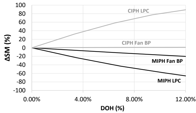
Figure 14: MCR Surge Margin change for different DoH
