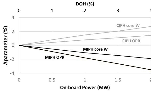
Figure 7: T/O OPR and core mass flow for different DoH
