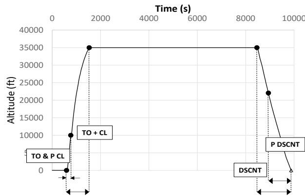
Figure 18: Mission density altitude and PMS
