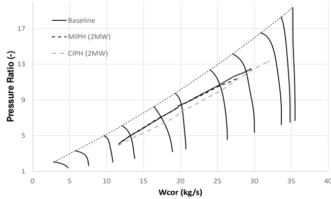
Figure 16 HPC operating line during slam acceleration
