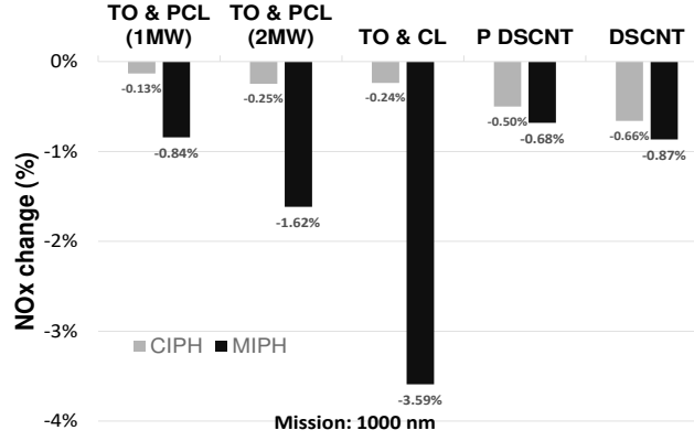
Figure 22: NOx emissions reduction for different PMS, 1000nm
