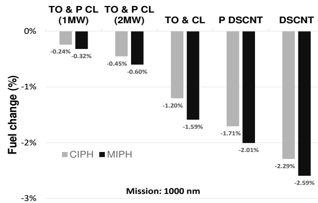
Figure 20: Fuel reduction for different PMS, 1000nm
