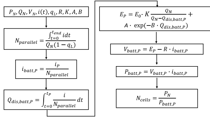
Figure 3: Battery sizing workflow adapted from [24]
