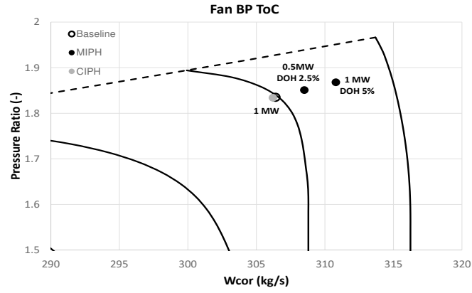
Figure 11: ToC Fan BP operating points for different DoH
