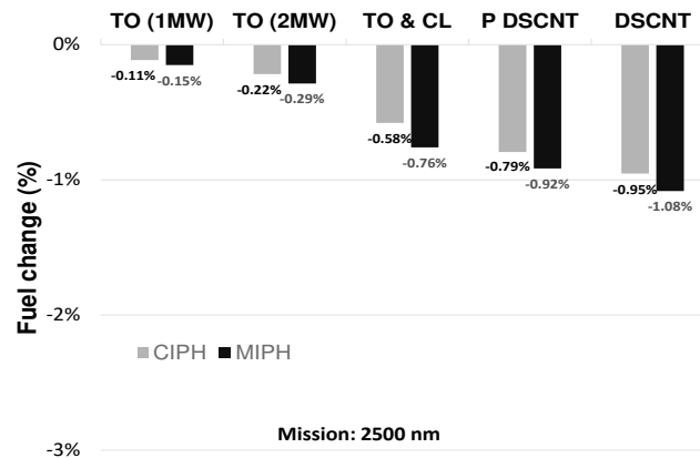
Figure 21: Fuel reduction for different PMS, 2500nm
