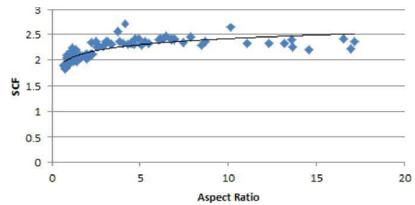
Fig. 5. SCF vs Aspect Ratio for single pit
