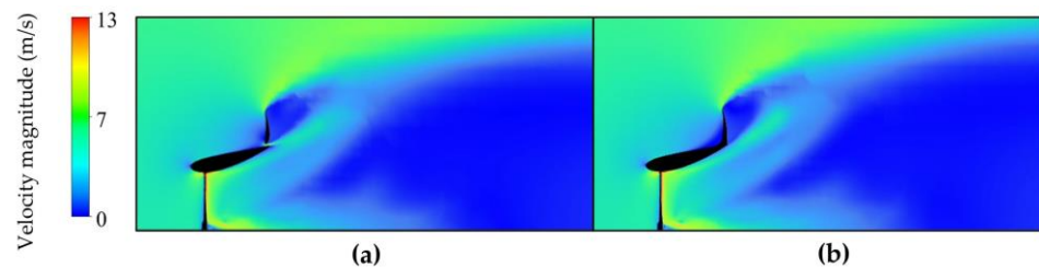
Figure 19. Velocity contours for (a) the multi-slot and (b) the flanged ducts with a Selig S1223 flap/flange at 90^\circ at V_0 = 5 m/s and \lambda = 5 .
