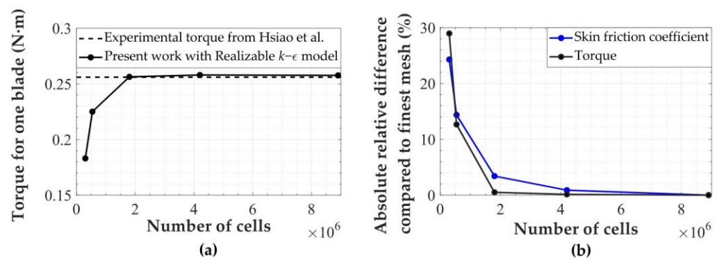
Figure 7. Result of the mesh independence study for the bare turbine conducted with the Realizable k-\epsilon model: (a) Torque obtained and comparison against the experimental value by [27], (b) relative difference of the torque and skin friction coefficient compared to the finest mesh tested.
