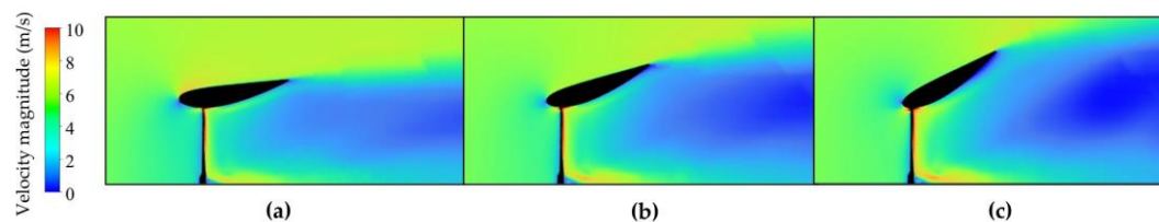
Figure 12. Contours of velocity magnitude in a plane perpendicular to the rotor for different duct angles: (a) 10^\circ , (b) 20^\circ and (c) 30^\circ , at V_0 = 5 m/s and \lambda = 5 .
