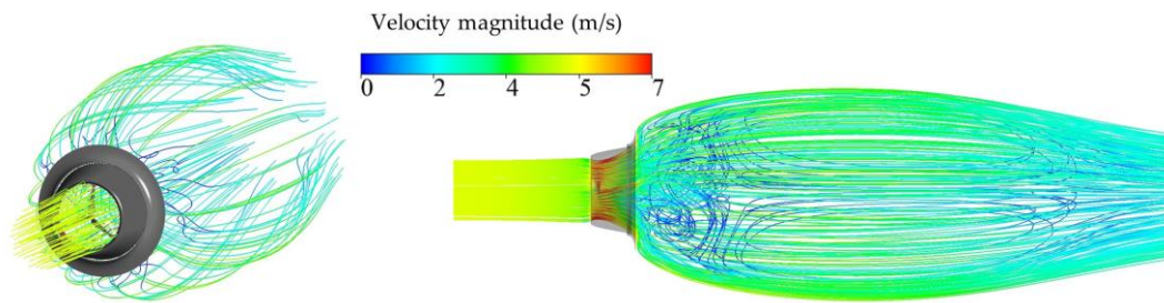
Figure 16. Three-dimensional streamlines around the turbine with a multi-slot duct with a gas turbine blade flap at a 90^\circ for V_0 = 5 m/s and \lambda = 5 .
