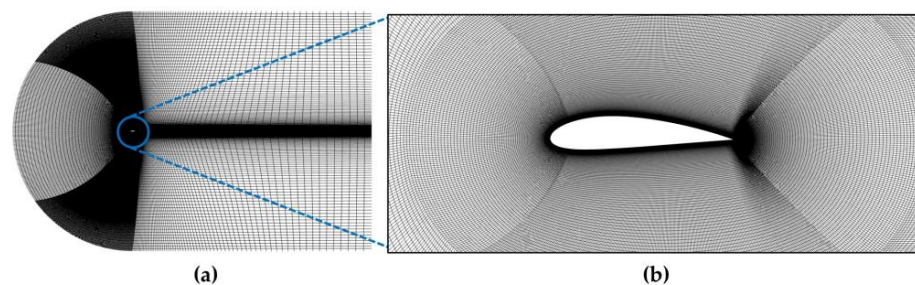
Figure 9. (a) Domain considered to study the lift and drag coefficients of the NACA4418 airfoil and (b) detail of the mesh around the airfoil.
