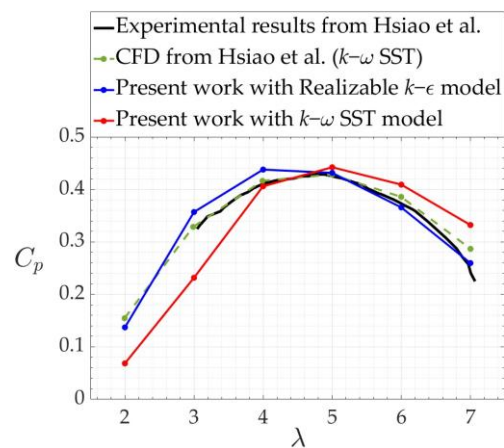
Figure 8. Comparison of the C_p values obtained numerically in the present study with the experimental and numerical results from Hsiao et al. [27].
