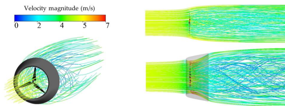
Figure 13. Three-dimensional streamlines around the bare turbine (top right) and the ducted turbine with a 15^\circ angle duct (bottom) for V_0 = 5 m/s and \lambda = 5 .
