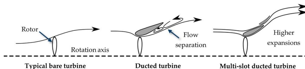
Figure 1. Illustration of the flow behaviour in a bare, ducted and a multi-slot ducted wind turbine.
