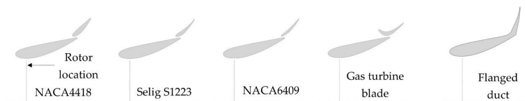
Figure 5. Two-dimensional schematic of the flap geometries studied in the present work.
