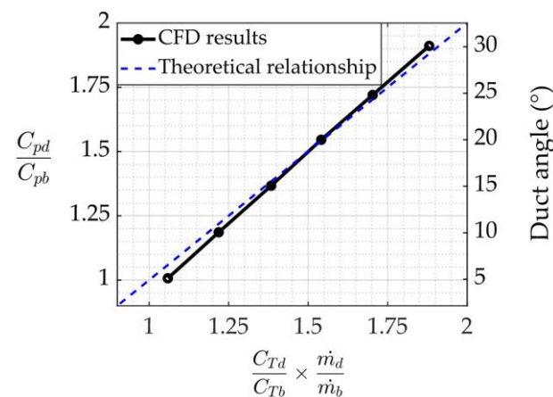
Figure 11. Comparison between CFD-based results obtained for the ducted turbine and the theoretical relationship in Equation (6).
