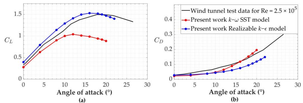
Figure 10. (a) Lift and (b) drag coefficients on a NACA 4418 airfoil obtained in the present work with Fluent using two different turbulence models at Re = 10^5 , and comparison against experimental data for Re = 2.5 \times 10^5 from [35].
