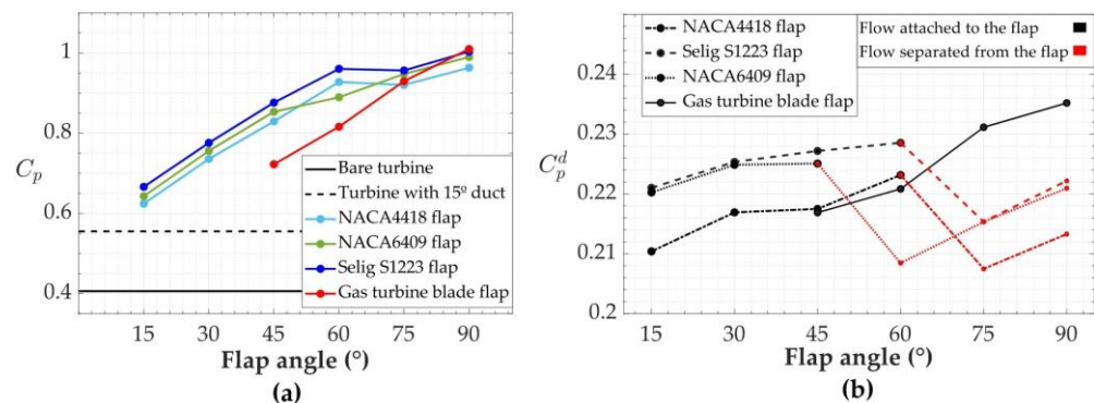
Figure 14. Results for the different flap geometries studied in terms of (a) power coefficient, (b) power coefficient considering the duct exit area. Results for V_0 = 5 m/s and \lambda = 5 .
