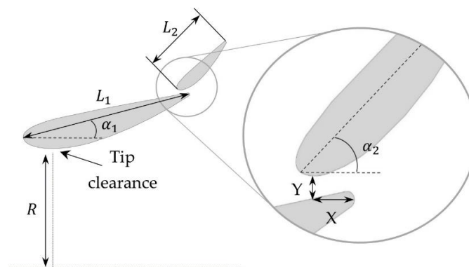
Figure 4. Main parameters of the multi-slot diffuser studied in the present work.
