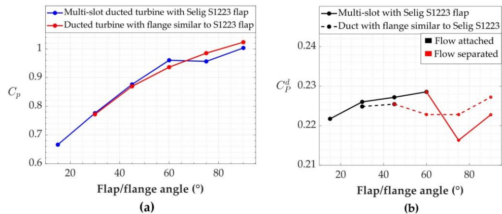
Figure 18. Comparison of the results between the multi-slot and the flanged ducts in terms of power coefficient considering (a) the rotor area and (b) the diffuser exit area at V_0 = 5 m/s and \lambda = 5 .
