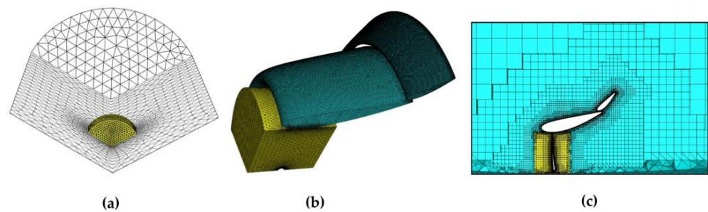
Figure 6. Examples of surface meshes for (a) the bare turbine, (b) the multi-slot case, and (c) volumetric mesh in a section perpendicular to the turbine plane for the multi-slot case.
