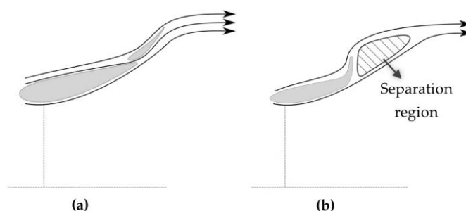
Figure 20. Illustration of the comparison of flow behaviour between (a) a multi-slot and (b) a compact flanged duct.
