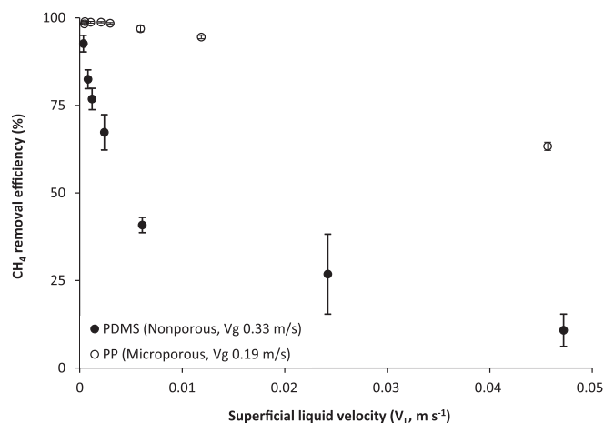
Fig. 2. Impact of superficial liquid velocity ( V_L ) on dissolved methane removal efficiency for the dense (PDMS) and microporous (polypropylene) membrane contactors. Gas velocity ( V_G ) fixed at 0.33 and 0.19 \text{m s}^{-1} for the nonporous and microporous membranes respectively.
