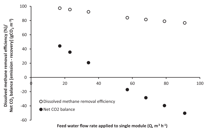
Fig. 11. Modelled dissolved methane removal efficiency estimated for a module with fibre length 0.546 \text{ m} and membrane area 220 \text{ m}^2 . Assumed feed water saturation concentration of 20 \text{ gCH}_4 \text{ m}^{-3} (approximate equilibrium concentration to 15^\circ \text{C} , y_{\text{CH}_4} 70%). Net \text{CO}_2 balance is the difference between non-recovered dissolved \text{CH}_4 at the HFMC outlet ( 20 \text{ gCO}_2 \text{ gCH}_4^{-1} ) and the use of the recovered fraction to offset grid electricity ( 0.47 \text{ kg kWh}^{-1} ).
