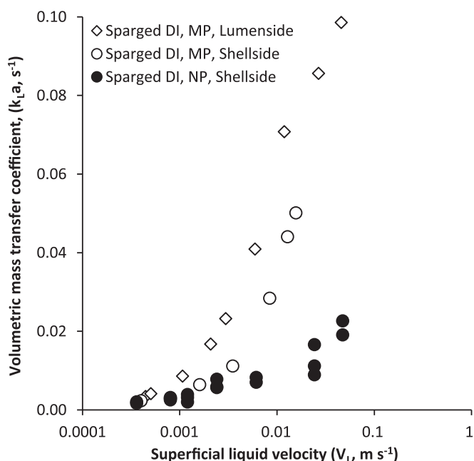
Fig. 10. Comparison of the determined volumetric mass transfer coefficients ( K_{La} ) for the non-porous and microporous membranes respectively. Data for the microporous membrane operated in both shell-side and lumen-side is presented.
