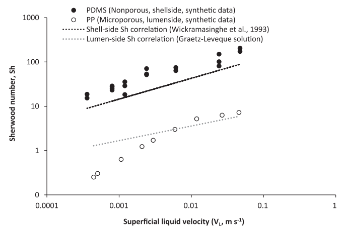
Fig. 6. Sherwood correlation for the dense (PDMS) and microporous (polypropylene) membrane contactors compared to established Sh correlations for lumen-side (Graetz-L  v  que solution, microporous) and shell-side flow [20].
