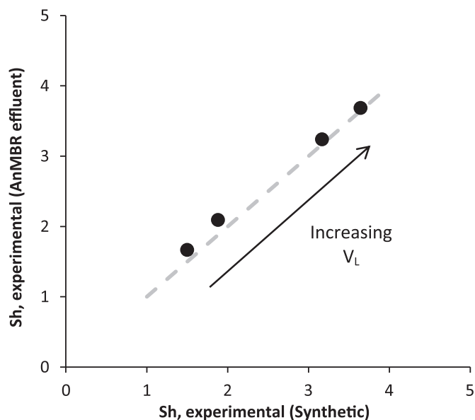
Fig. 8. Comparison of the Sherwood number ( Sh ) derived experimentally using synthetic effluent in the microporous contactor to the Sh number determined experimentally when using real effluent from an AnMBR. Dashed line represents a 1:1 relationship.
