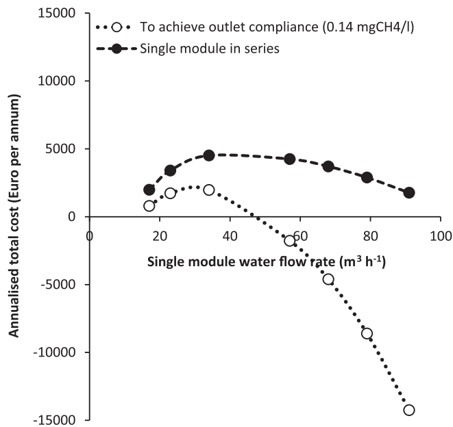
Fig. 13. Cost indices presented for dissolved methane recovery based on those of based on [27] with inclusion of a revenue component to account for methane utilisation (€0.094 kWh -1 ; 40% electrical conversion efficiency). Cost based on a water flow of around 10,000 PE. Total number of modules in series required (total length/module length) was determined by rounding. Membrane cost used € 40 m -2 ; 7 year life expectancy. Values above zero indicate a positive financial return.
