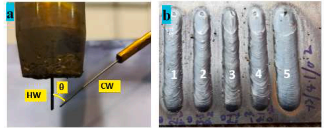
Fig. 1. Alloy mixing procedure: (a) Positioning of the HW & CW, (b) beads on plate.
