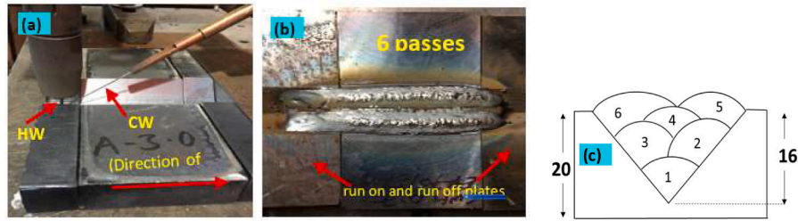
Fig. 2. (a) Welding set up: (b) 6-pass welded sample, (c) schematic of the 6-pass bead sequence.
