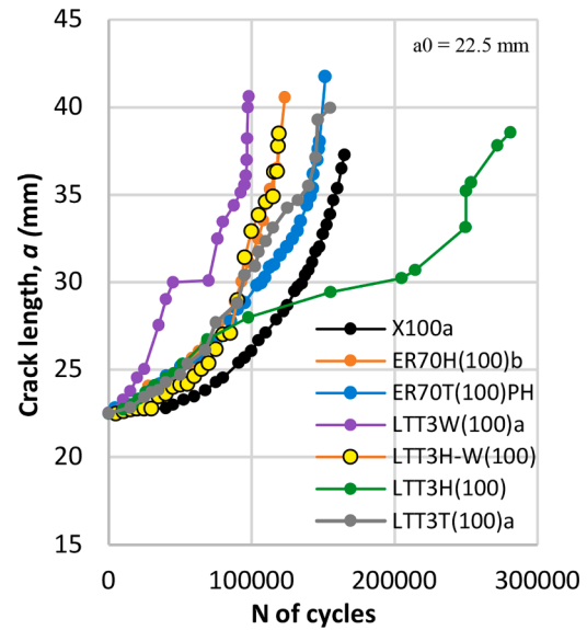
Fig. 22. The a vs. N for the LTT alloy.
