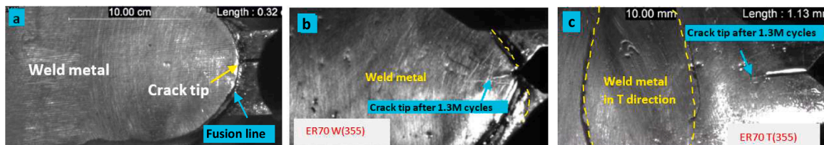
Fig. 19. Crack tip positioning during ER70 testing; (a) crack tip outside the weld metal, (b) crack tip inside the weld metal, (c) weld metal in perpendicular direction to the FCG front.
