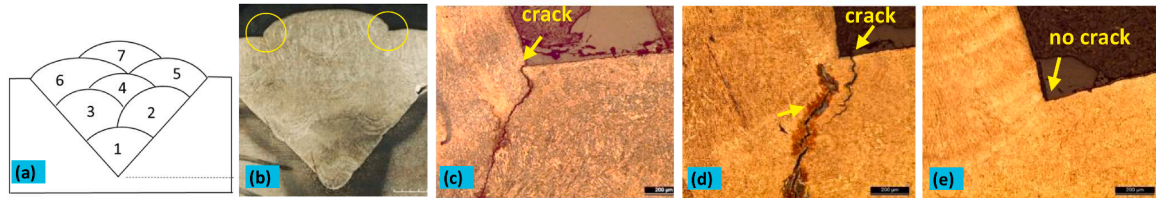
Fig. 3. Weld metals: (a) schematic of 7-pass weld, (b) 7-pass weldment showing toe or notch area examined, (c & d) typical cracking observed in the LTT alloy, (e) LTT alloy composition with no cracking.
