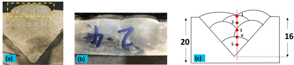
Fig. 4. Composition and hardness measurements: (a) location of compositional measurement (b) cut section for hardness test, (c) hardness measurement scheme.
