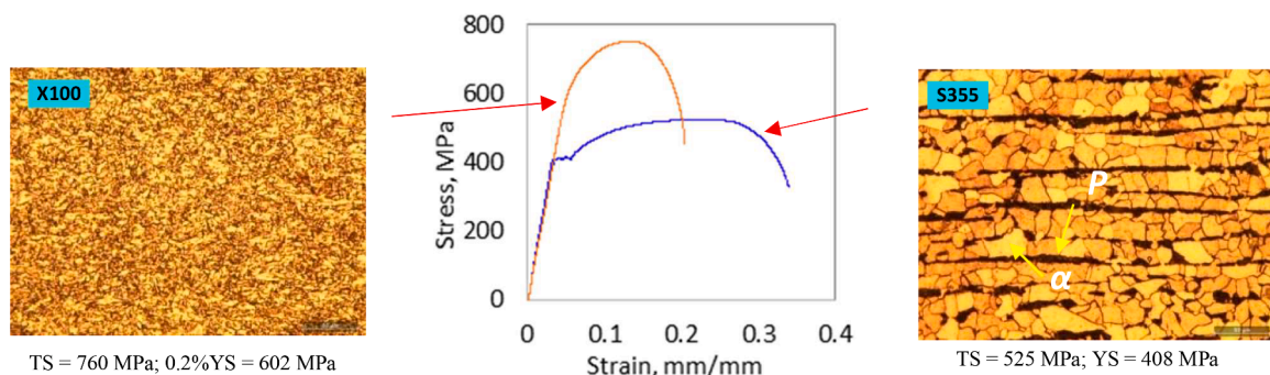
Fig. 6. Microstructure and mechanical properties of the baseplates.
