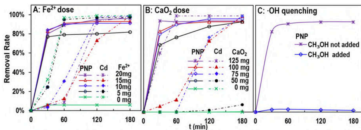
Figure 4. Effect of \text{Fe}^{2+} dosage (A), \text{CaO}_2 dosage (B) and \text{CH}_3\text{OH} quencher addition (C). The solid line represented the PNP data and the dashed line represents the Cd data. Experimental conditions: solution volume = 200 mL, initial PNP = 40 mg/L, initial Cd = 10 mg/L, \text{Fe}^{2+} = 75 mg/L, nano- \text{CaO}_2 = 500 mg/L, initial pH = 2.8, oscillation frequency = 160 rpm, T = 298\text{ K} .
