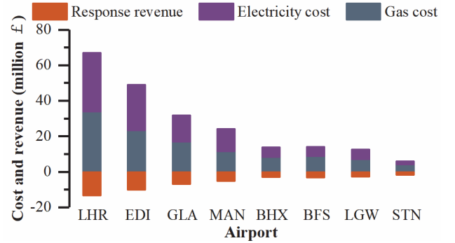
Fig. 5. Annual EA charging costs and A2G frequency response revenue for 8 UK airports
