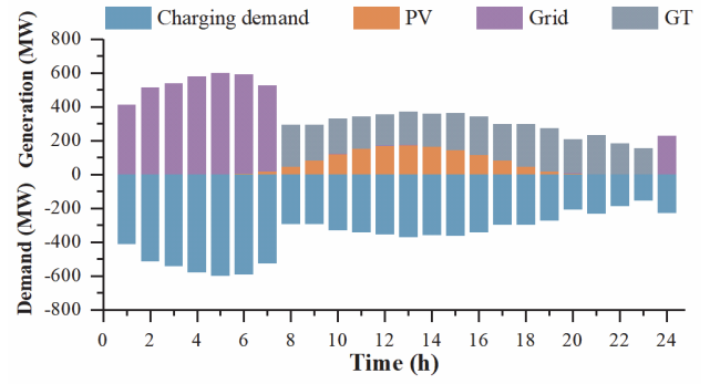
Fig. 3. Energy dispatch results of the 8 UK airports
