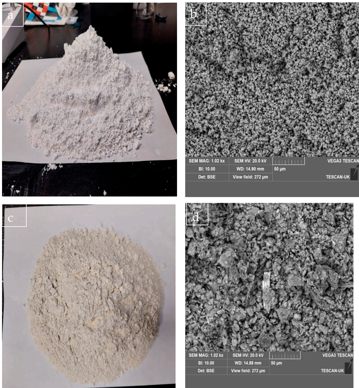
Figure 2. (a,b) Photographic and SEM image of limestone powder. (c,d) Photographic and SEM image of metakaolin powder.
