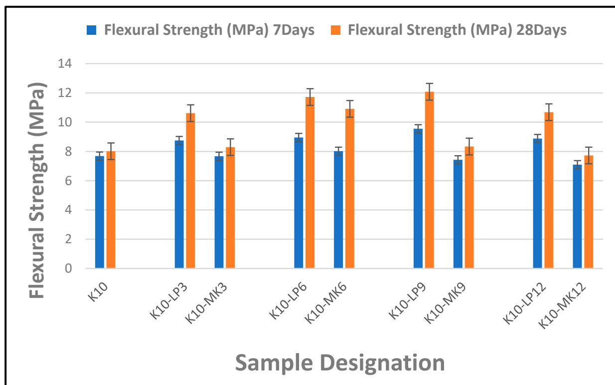
Figure 6. Flexural strength of composite boards reinforced by 10 wt.% of waste kraft fibre and 3–12% of limestone/metakaolin powder as partial cement replacement (7 and 28 days).
