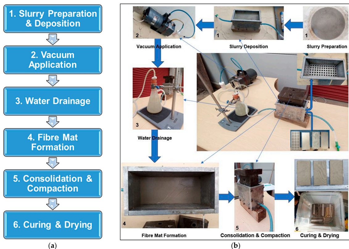
Figure 4. (a) Flowchart for vacuum dewatering process. (b) Laboratory setup for composite production.
