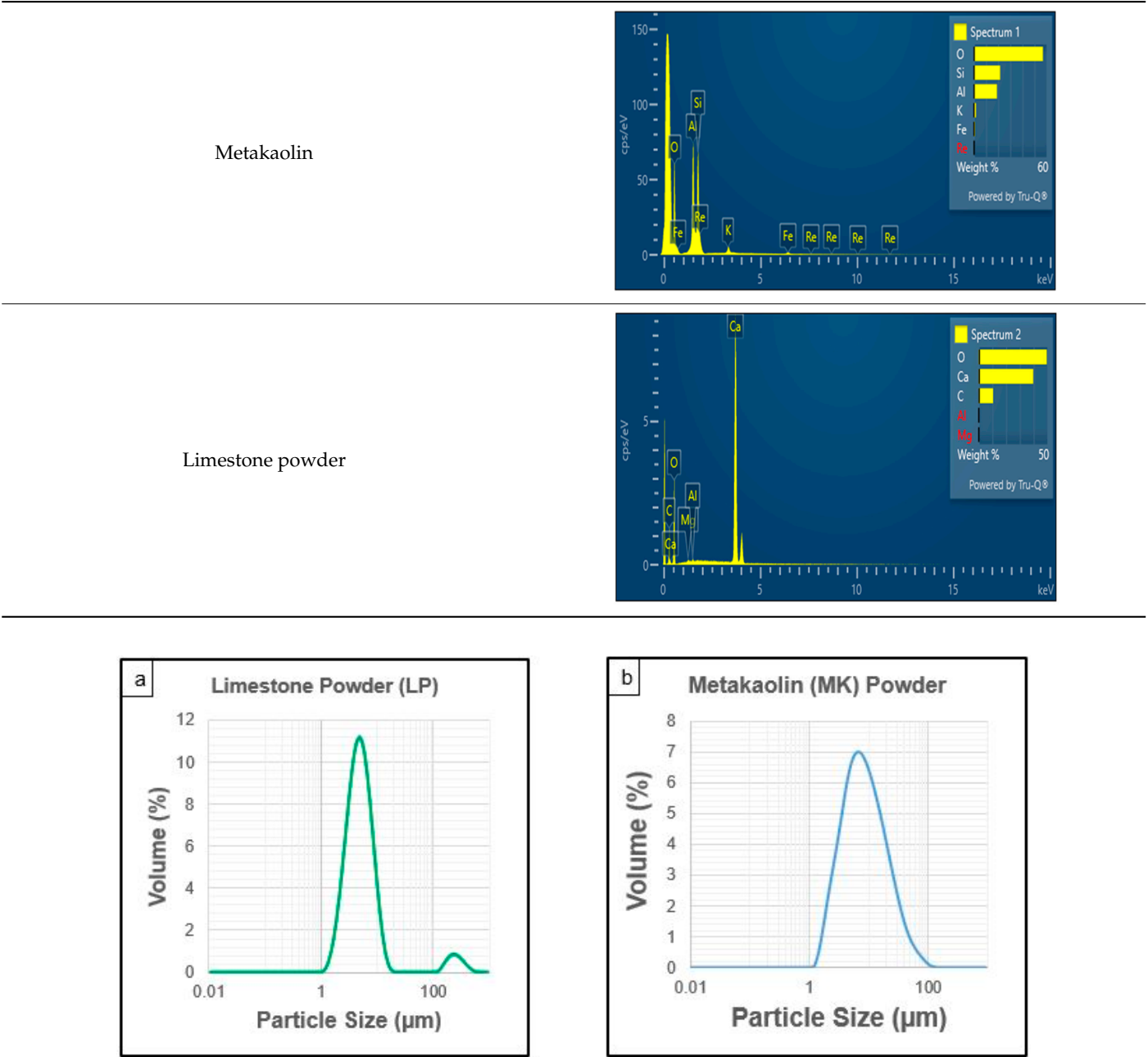
Figure 1. Master sizer particle size analysis of (a) limestone powder and (b) metakaolin powder.
