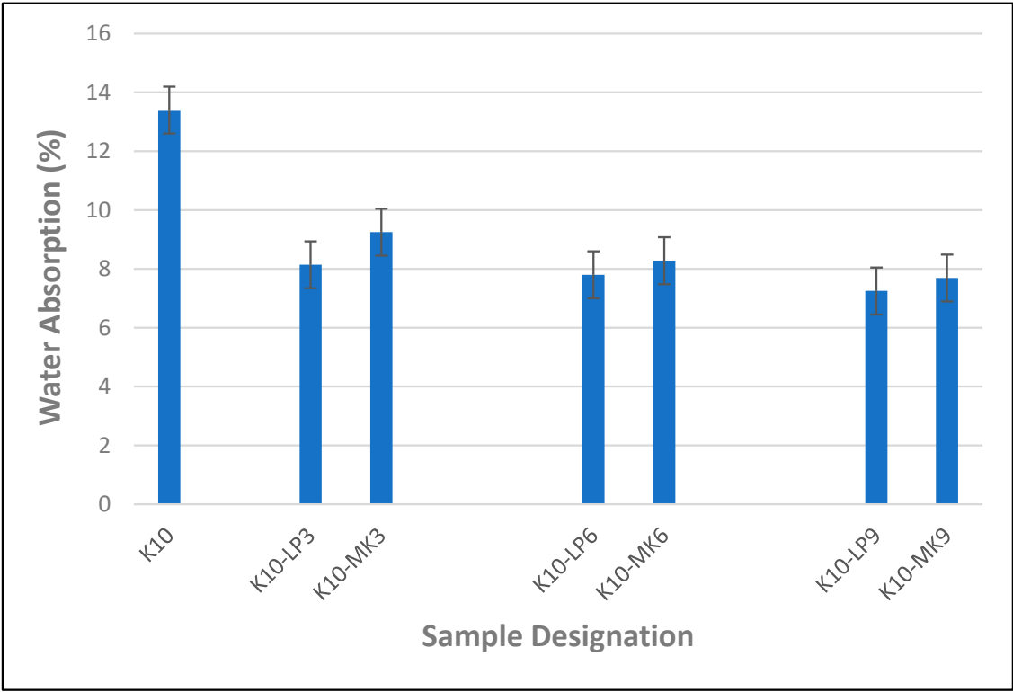
Figure 9. Water-absorption characteristics of waste kraft fibre-reinforced cement composite boards containing 3–9% metakaolin and limestone powder as partial cement replacement.
