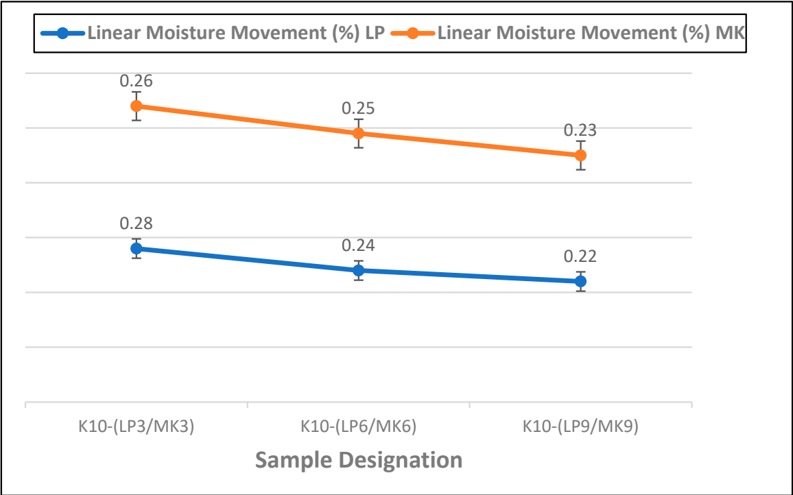
Figure 8. Linear moisture movement of composite boards containing 3–9% metakaolin and limestone powder as partial cement replacement.
