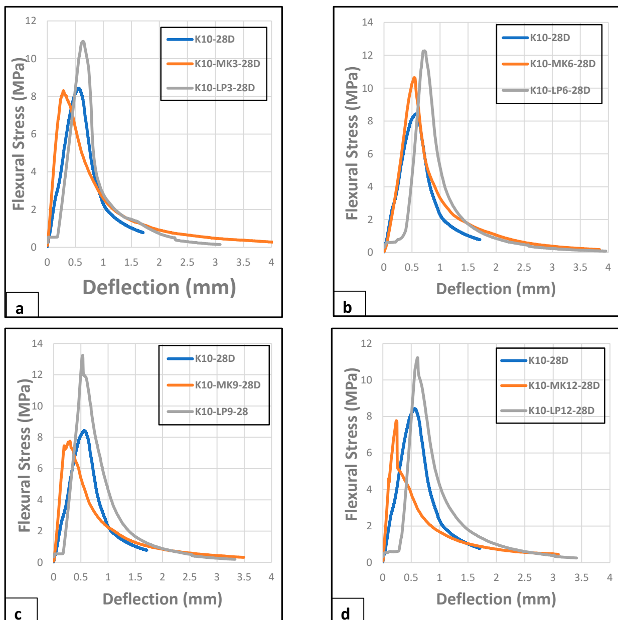
Figure 7. Flexural behaviour of composite boards reinforced by 10 wt.% of waste kraft fibre and (a) 3%, (b) 6%, (c) 9%, and (d) 12% of limestone powder/metakaolin as partial cement replacement (28 days).
