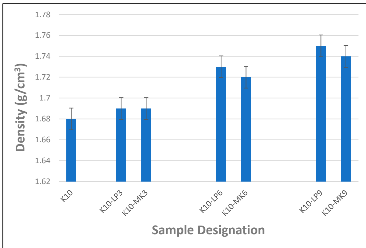
Figure 10. Density of waste kraft fibre-reinforced cement composite boards containing 3–9% metakaolin and limestone powder as partial cement replacement.
