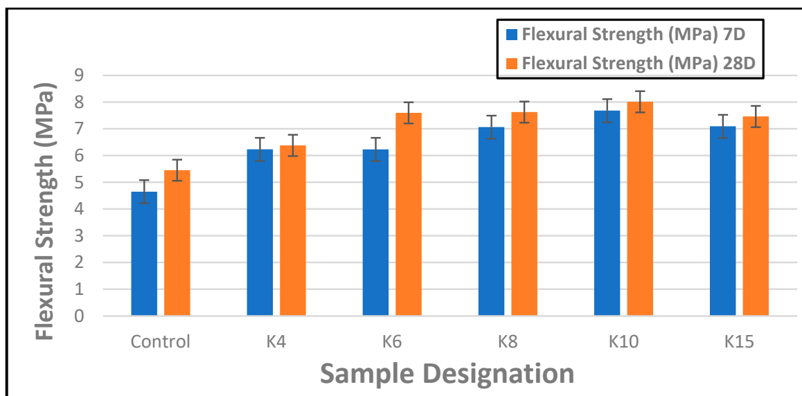
Figure 5. Flexural strength of composite boards reinforced with waste kraft fibre (7 and 28 days).
