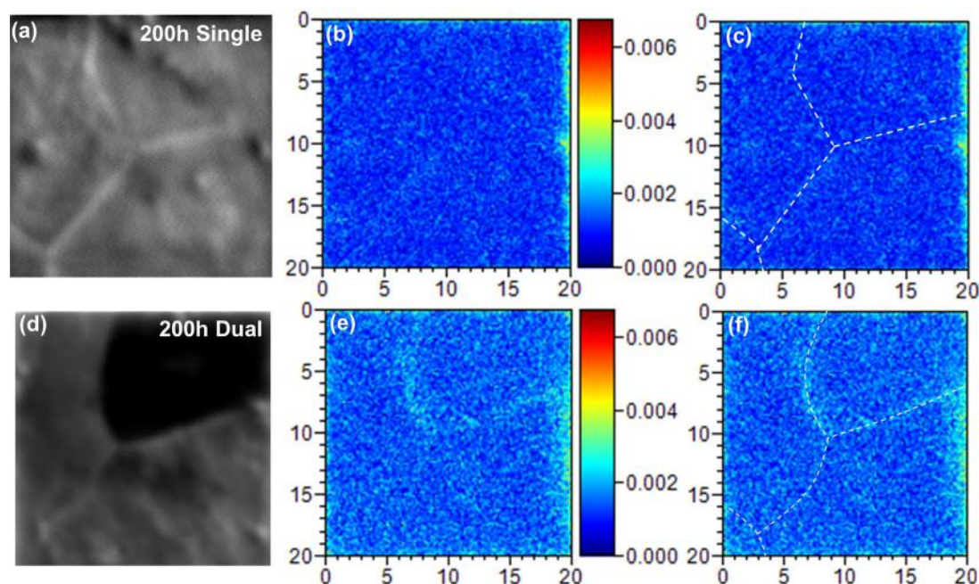
Fig. 5. Plane-view ToF-SIMS analysis of polished samples after exposure at 750 °C for 200 h under the single atmosphere (a–c) and the dual atmosphere (d–f). The two-dimensional distribution of hydrogen concentration is shown for the single atmosphere in (b), with grain boundaries highlighted by dashed lines in (c). Similarly, the two-dimensional hydrogen distribution under the dual atmosphere is presented in (e), with grain boundaries highlighted by dashed lines in (f). The field of view is 20 \mu\text{m} \times 20 \mu\text{m} . (For interpretation of the references to color in this figure legend, the reader is referred to the web version of this article.)
