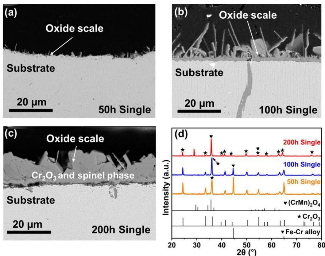
Fig. 1. SEM cross-section of SUS430 in cathode side exposed to the single atmosphere (air with 3% H 2 O) at 750 °C for 50 h (a), 100 h (b), and 200 h (c), along with corresponding surface XRD analysis (d). XRD analysis phase identification used Powder Diffraction Files (PDF): Fe–Cr alloy (PDF #00-054-0031), Cr 2 O 3 (PDF #01-070-3755) and (CrMn) 2 O 4 (PDF #00-045-0504).
