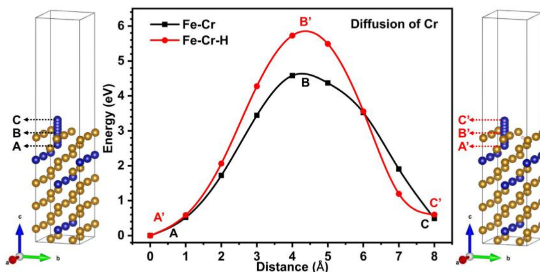
Fig. 7. The energy variation curve of diffusion path of Cr in Fe-Cr alloy. The black curve represents the Cr diffusion energy barrier (Fe-Cr) without hydrogen, while the red curve represents the Cr diffusion energy barrier (Fe-Cr-H) with hydrogen. The horizontal axis represents the distance of Cr diffusion path, and the vertical axis represents the energy at different positions during the diffusion process. (For interpretation of the references to color in this figure legend, the reader is referred to the web version of this article.)
