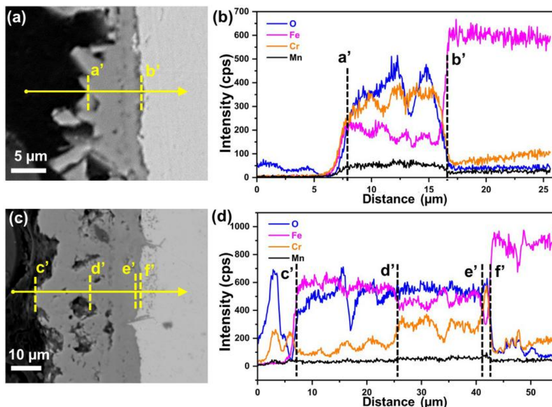
Fig. 3. SEM cross-section of SUS430 in cathode side exposed to the single atmosphere at 750 °C for 200 h (a) and the line scan. (b) SEM cross-section of SUS430 exposed to the dual atmosphere at 750 °C for 200 h (c) and the line scan (d).
