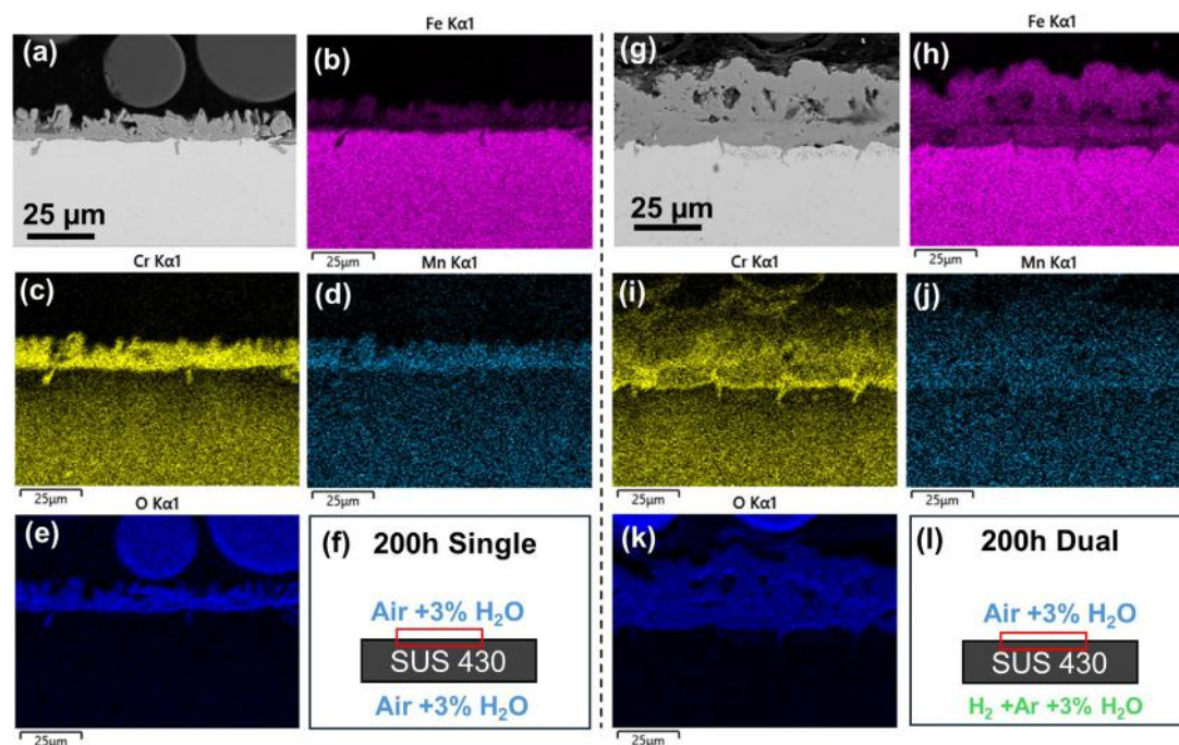
Fig. 4. SEM cross-section of SUS430 in cathode side exposed to the single atmosphere at 750 °C for 200 h (a) and the EDS maps (b–e), and schematic illustration of the single atmosphere test. (f) SEM cross-section of SUS430 exposed to the dual atmosphere at 750 °C for 200 h (g) and the EDS maps (h–k), and schematic illustration of the dual atmosphere test (l).
