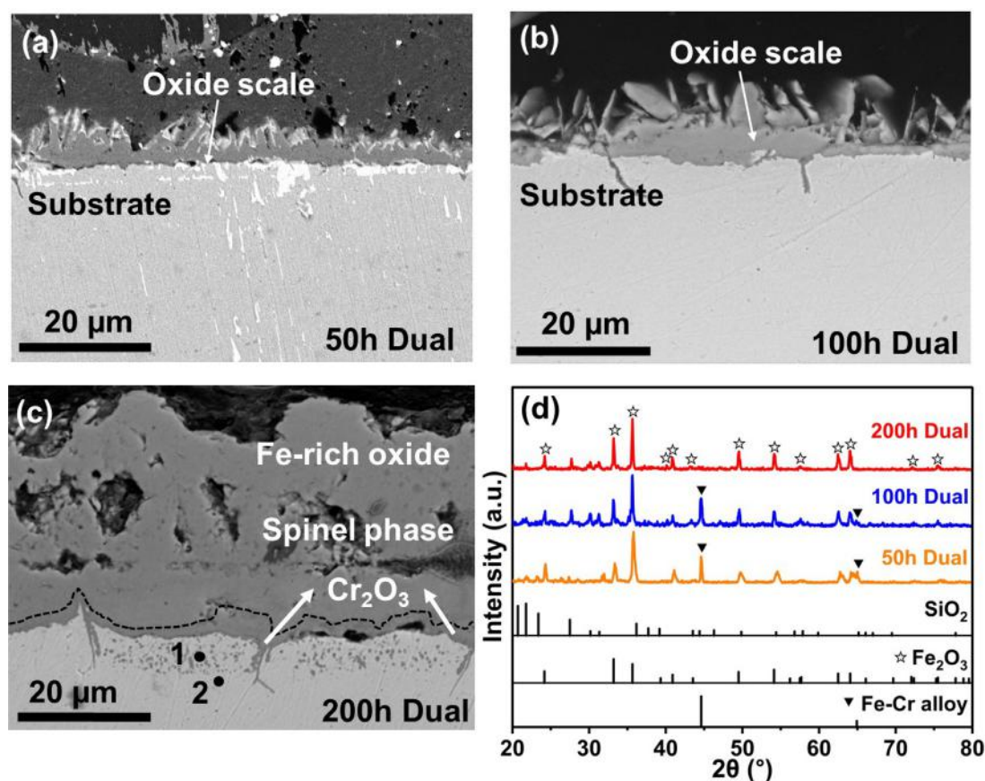
Fig. 2. SEM cross-section of SUS430 in cathode side exposed to the dual atmosphere (one side in air with 3% H 2 O; the other side in 2.91% H 2 , 94.09% Ar with 3% H 2 O) at 750 °C for 50 h (a), 100 h (b), and 200 h (c), along with corresponding surface XRD analysis (d). XRD analysis phase identification used PDF cards: Fe–Cr alloy (PDF #00-054-0031), Fe 2 O 3 (PDF #01-089-0599) and SiO 2 (PDF #00-042-1401).
