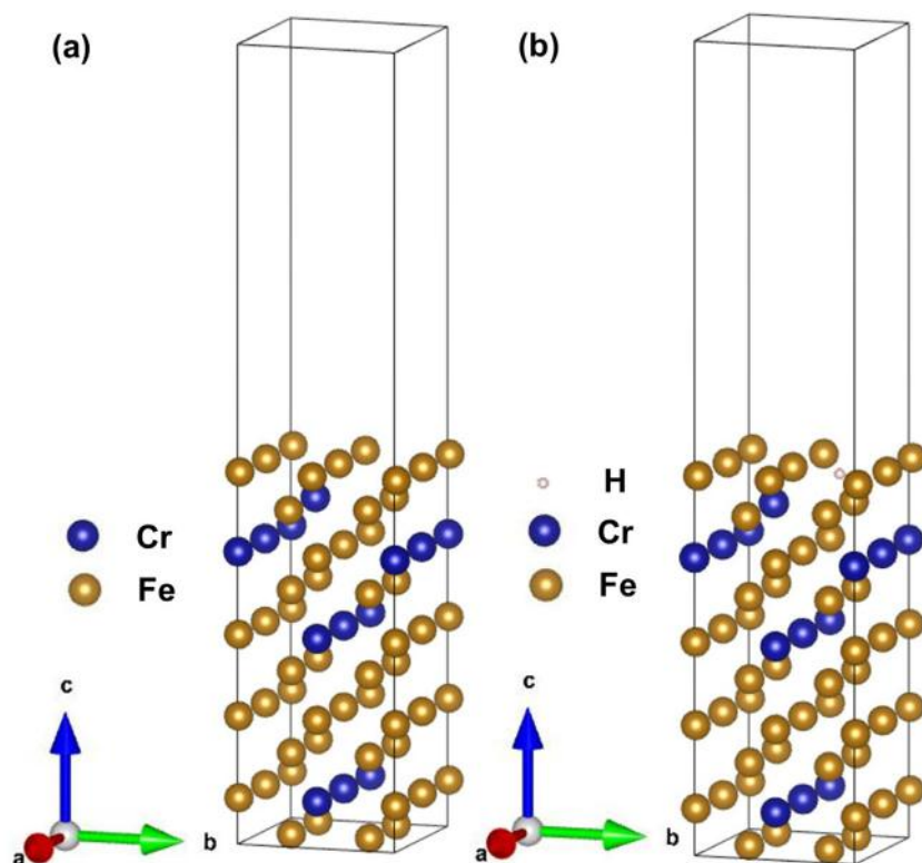
Fig. 6. Schematic diagram of Fe 33 Cr 7 supercell (a) and the same structure after hydrogen adsorption (b) in the (110) crystal plane.
