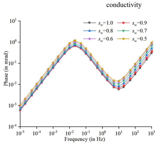
(c) Frequency-dispersion spectra of phase angle
