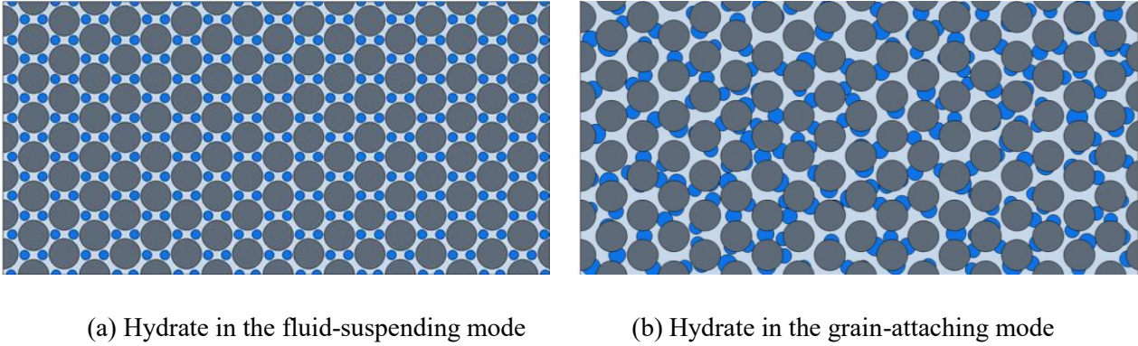
Fig. 1 Computational domains of the numerical models for different micro-distribution modes of hydrates (Blue: Hydrate cluster, Dark gray: solid grain, Light gray: pore water)
