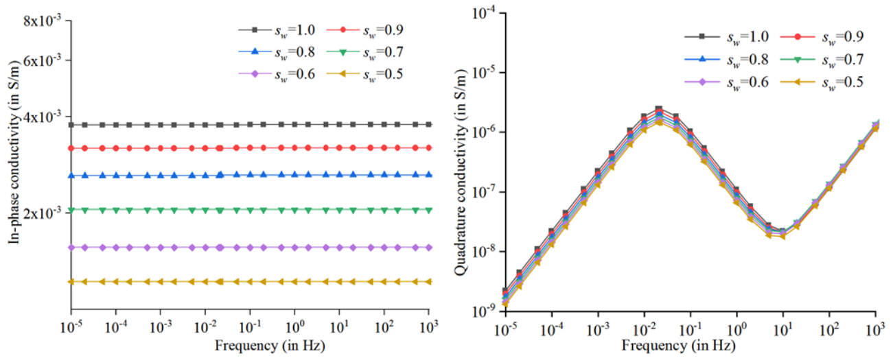
(a) Frequency-dispersion spectra of in-phase conductivity (b) Frequency-dispersion spectra of quadrature
