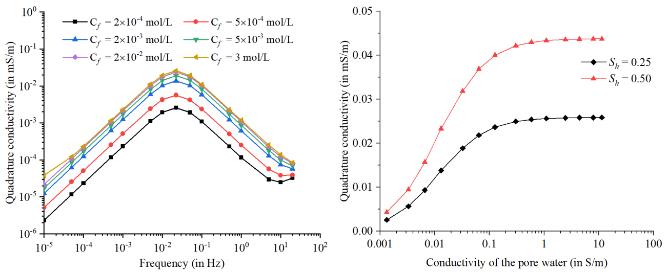
(a) Spectra of quadrature conductivity for S_h = 0.25
