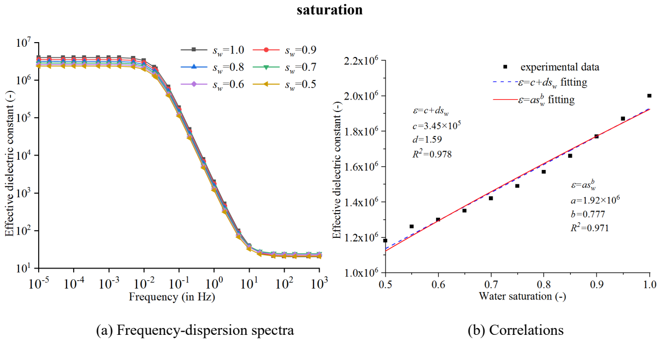
Fig. 6 Frequency-dispersion spectra of the effective dielectric constant and correlations between the effective dielectric constant at the peak frequency and water saturation
