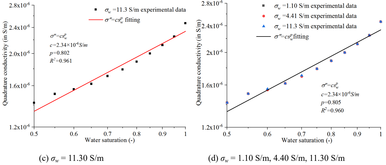
Fig. 8 Correlations between the quadrature conductivity and water saturation at high salinities of the pore water
