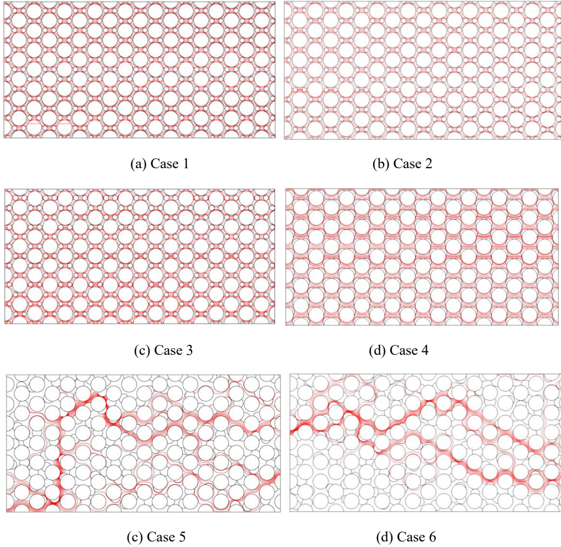
Fig. 10 Spatial distributions of the electrical current density for different micro-distribution modes of hydrates
