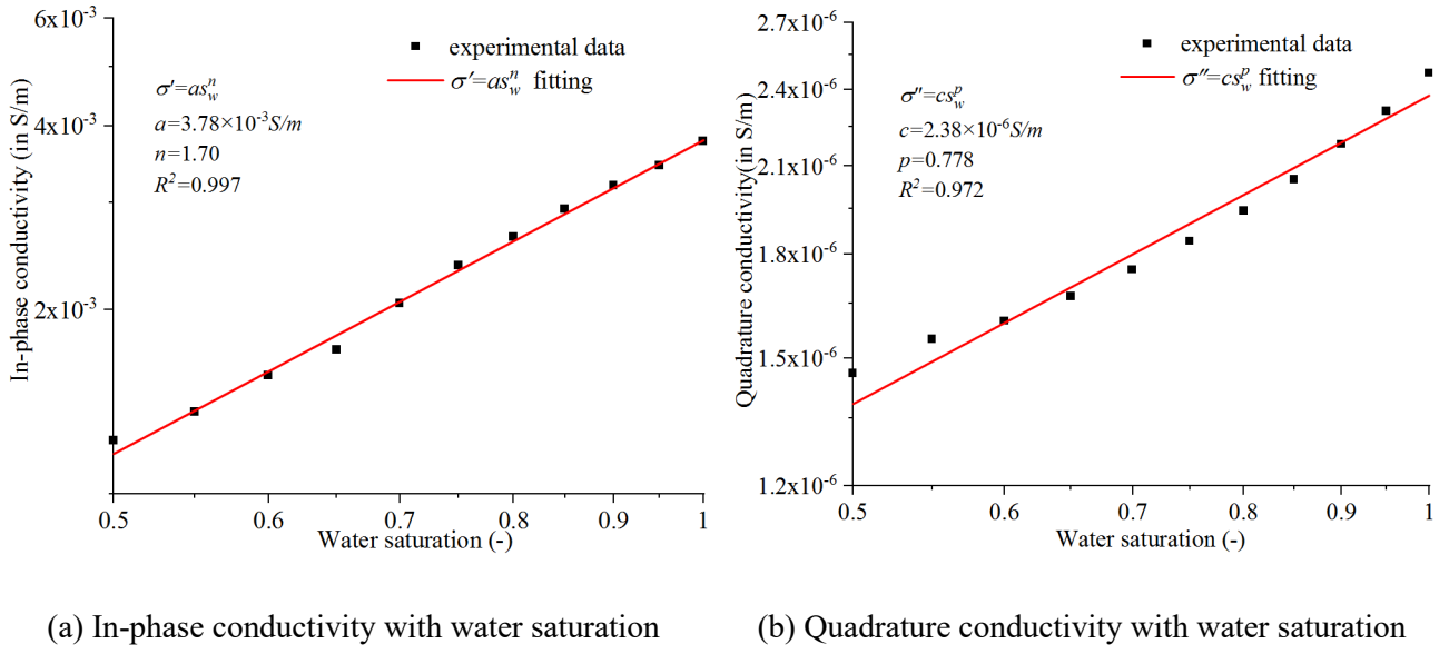
Fig. 5 Correlations between parameters of the complex conductivity at the peak frequency and water saturation
