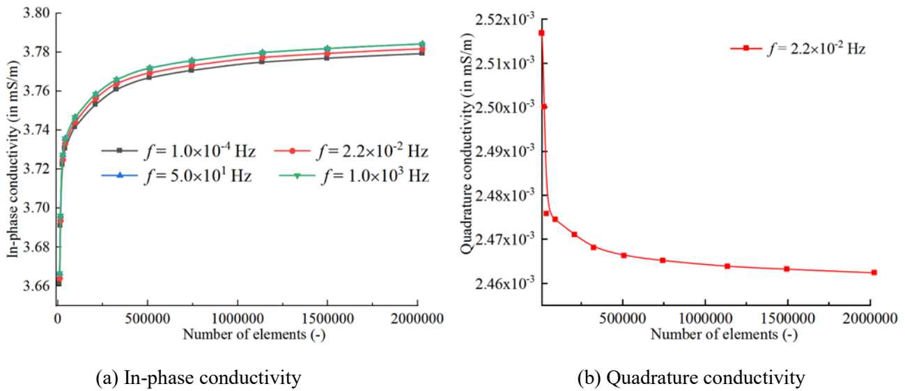
Fig 2 Variations of the complex conductivity with the number of elements for different levels of meshes
