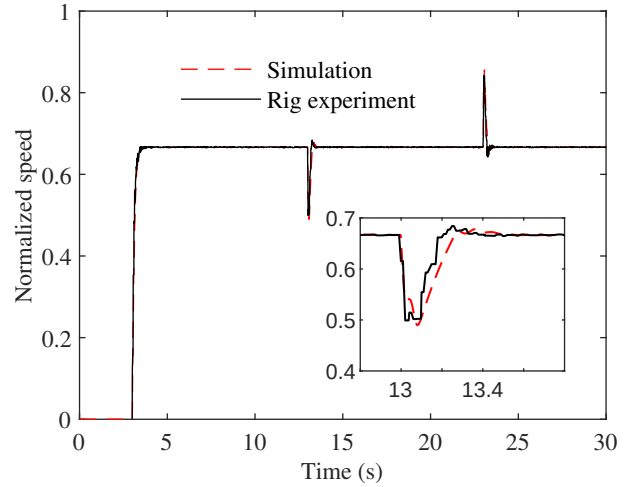
Fig. 11: Simulated and experimental results of the motor-side shaft with \tau_1 = T_d , K_p = 2.9 , K_i = 34.5 ( r = 0.67\omega_N , T_L = 0\text{ N}\cdot\text{m} , 0.67T_G and 0\text{ N}\cdot\text{m} at 3-13 s, 13-23 s and 23-30 s, respectively).
