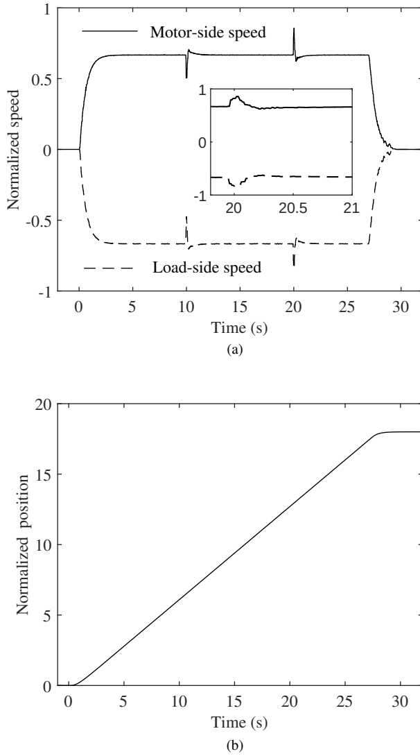
Fig. 16: Experimental measurements (a) operating speed (b) load-side position ( R_p = 18 , T_L = 0\text{ N}\cdot\text{m} , 0.67T_G and 0\text{ N}\cdot\text{m} at 0-10 s, 10-20 s and 20-35 s, respectively).
