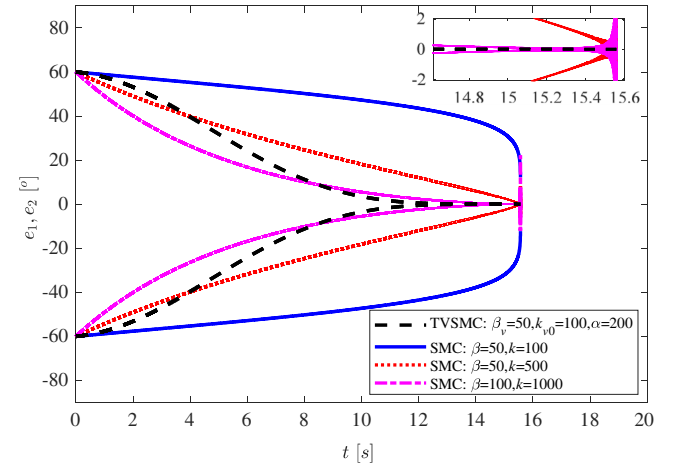
Fig. 2 Comparison of system tracking errors by SMC and TVSMC.
