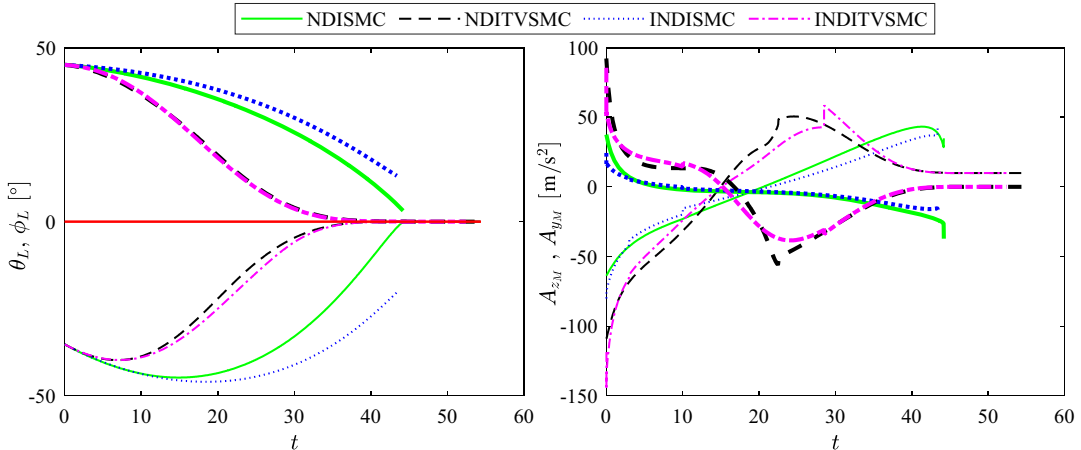
Fig. 9 Guidance performance against the constant moving target under \theta_{LF} = 0^\circ, \phi_{LF} = 0^\circ .
