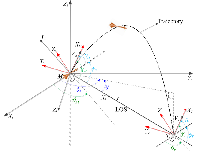
Fig. 1 Three-dimensional interception geometry for the missile and target.
