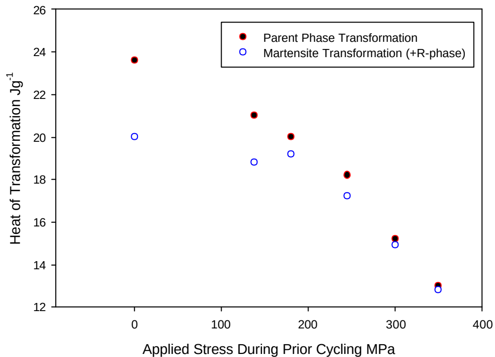
Graph 12-2 Heats of Transformation After 100 thermal Cycles at Five Different Stresses
