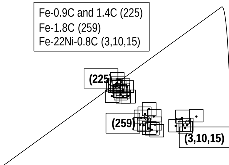
Figure 2-5 Some habit plane determinations in iron alloys. Greninger and Troiano 33 34
