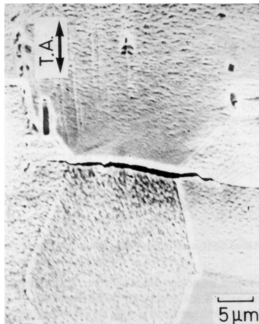
Figure 13-8 Fatigue crack nucleation along a grain boundary in a NiTi alloy 181
