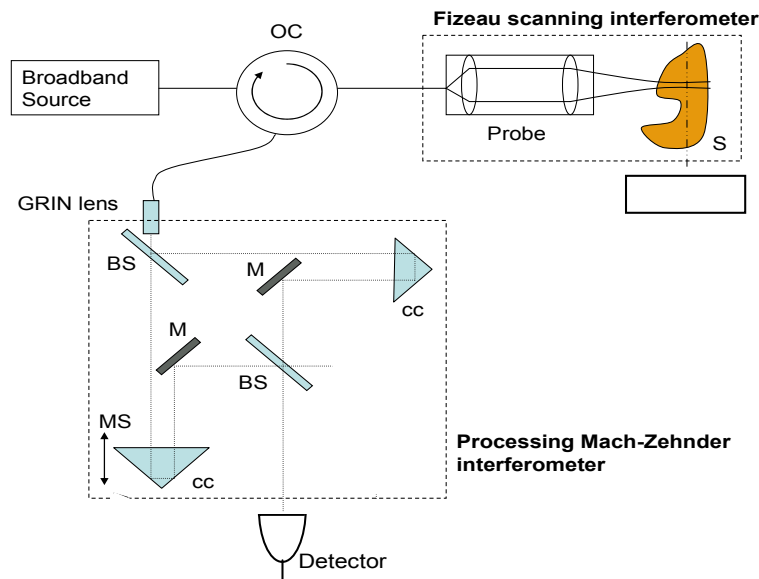
Fig. 3. Configuration for Fizeau-based OCT system with Mach-Zehnder type processing interferometer. OC = optical circulator, S = sample, BS = beam splitter, M = mirror, CC = corner cube prism, MS = micropositioning stage.
