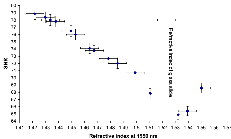
Fig. 5. SNR of the OCT signal for a series of oils of known refractive index, deposited on a glass microscope slide.
