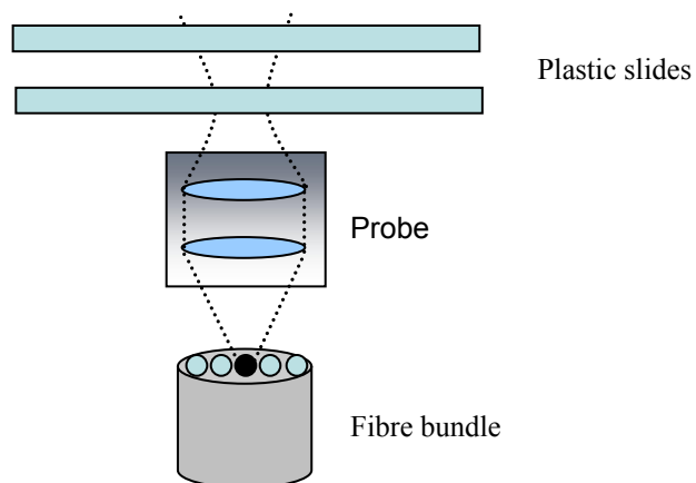
Fig. 10. Experimental arrangement of the fibre bundle, probe and a sample of two plastic projector slides.
