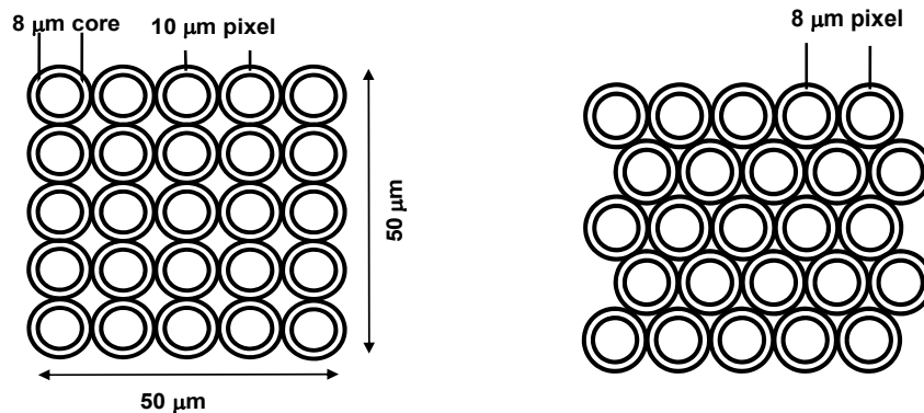
Fig. 7. Fibre bundle packaging arrangements: left , wound bundle; right, leached bundle.
