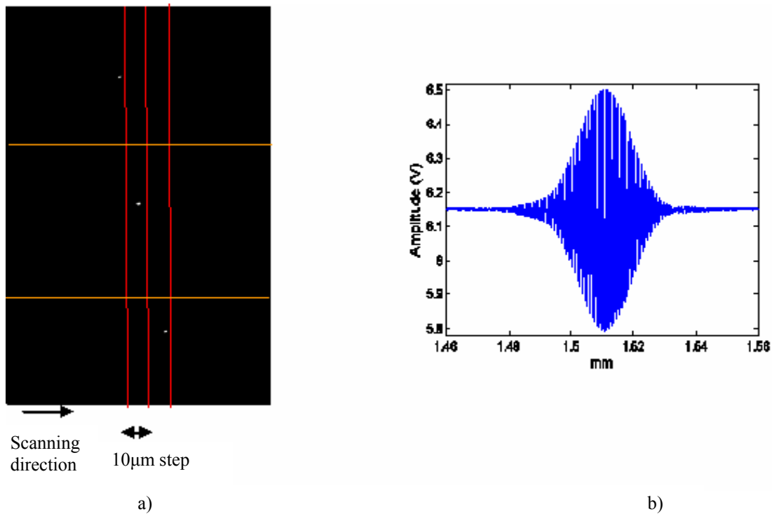
Fig. 8. a) 3 fibres illuminated in sequence, by scanning of the input beam. b) Coherence envelope using mirror as sample.
