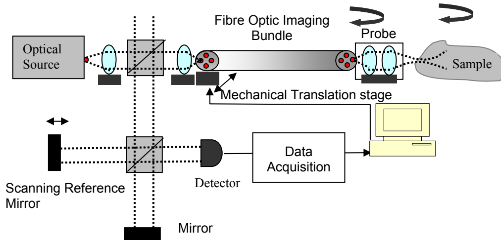
Fig. 6. Fizeau based OCT incorporating a coherent imaging fibre optic bundle.
