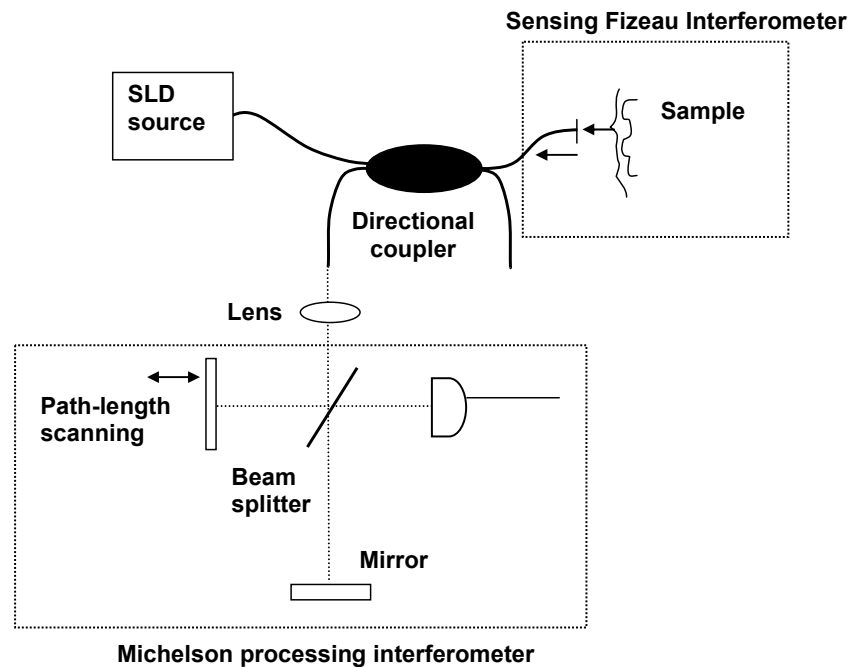
Fig. 1. Configuration for Fizeau configuration OCT system with a Michelson processing interferometer.
