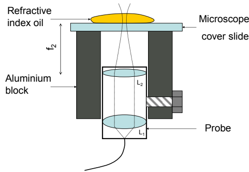
Fig 4. Experimental arrangement for reflectivity measurements on calibrated refractive-index oils. L = lens. The distance f_2 corresponds to the focal length of the second lens in the probe head.
