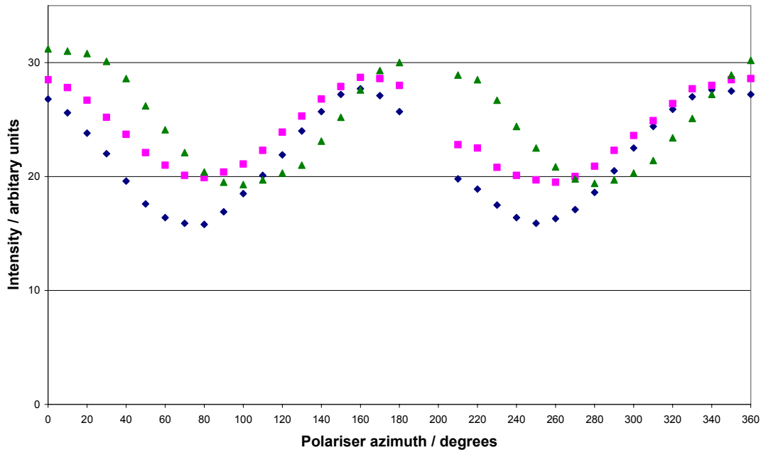
Fig. 2. Plot of intensity variation in the output from three individual fibres of the bundle, as a polarizer is rotated at the output, showing that the state of polarization differs between fibres.
