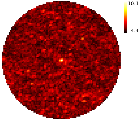
FIG. 4. SNR sky map for outlier A14. The disk (0.025 rad radius) is centered on the location of the signal. Each pixel (0.555 mrad) on the sky map shows the SNR maximized over a 5 \times 5 template sub-grid and all polarizations. The high frequency of the signal (1404 Hz) allows good localization.
