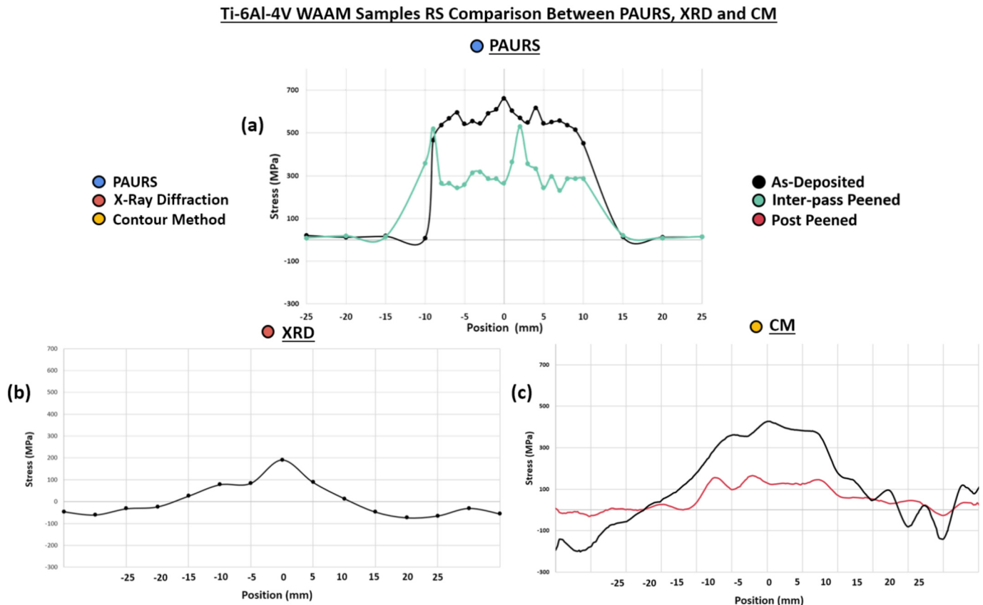
Fig. 31. (a) Final PAURS RS measurements, (b) XRD as-deposited RS, (c) CM RS for as-deposited and post-peened samples.
