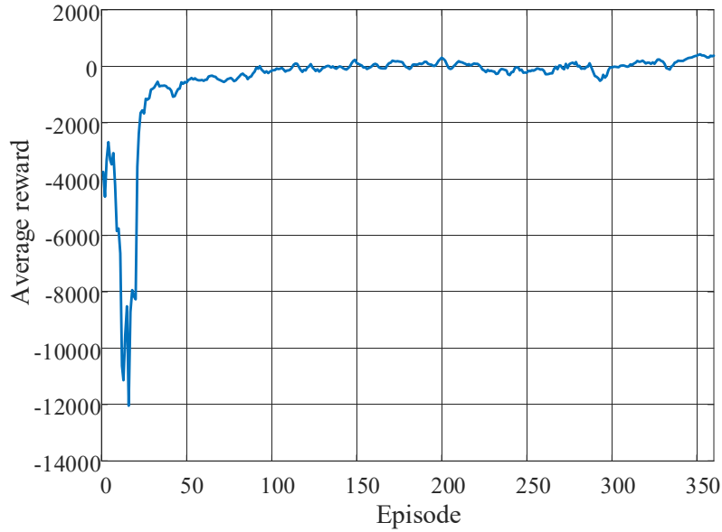
Fig. 5. Convergence of training.
