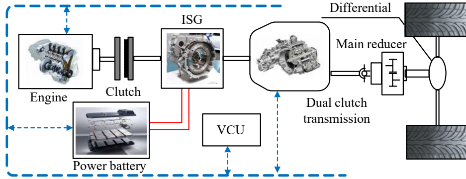
Fig. 2. Powertrain system of the PHEV.
