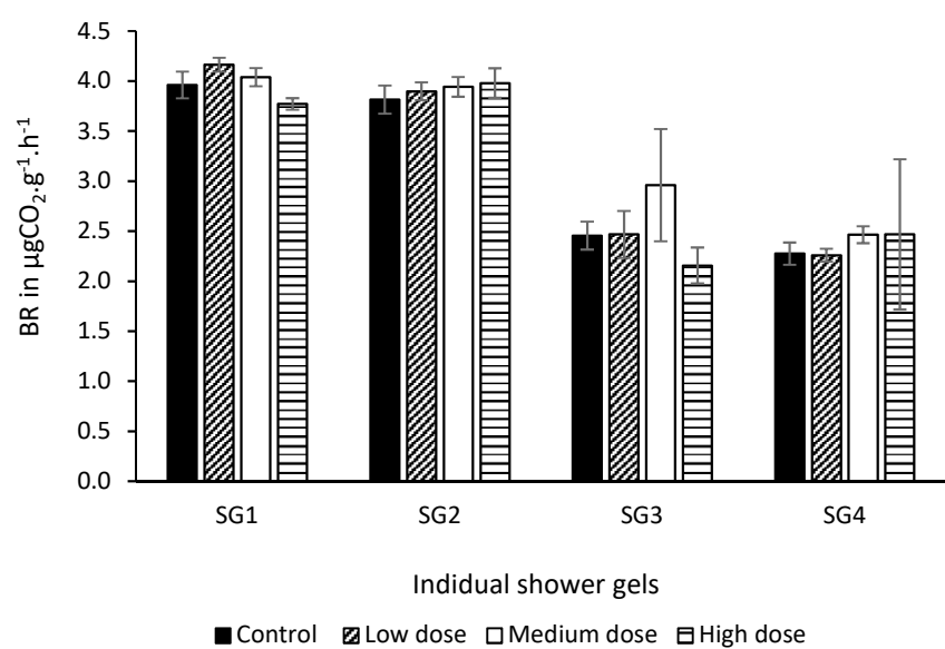
Figure 5. Average basal respiration of soil (BR - in \mu\text{gCO}_2.\text{g}^{-1}.\text{h}^{-1} ) exposed to low ( 0.7 \mu\text{g.L}^{-1} ) medium ( 1.4 \mu\text{g.L}^{-1} ) and high doses ( 2.8 \mu\text{g.L}^{-1} ) of four shower gels.
