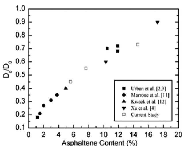
Figure 10. Effect of asphaltene content in VRs on the size ratio of coke particle to initial droplet.
