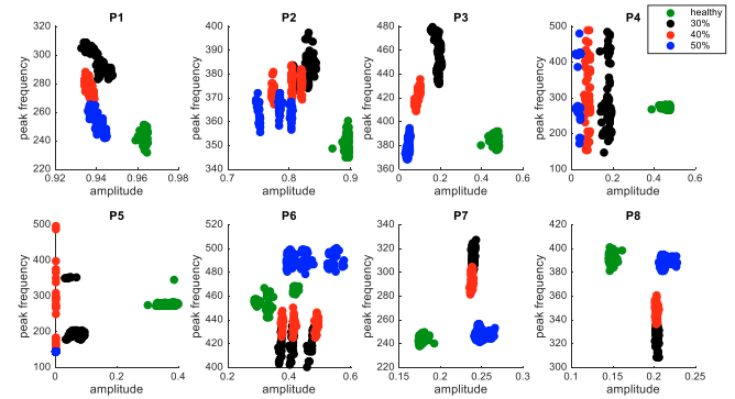
Fig. 2. Clustering visualisation for all 8 considered channels, where each faulty case has 81 combinations of degradation.
