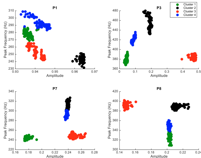
Fig. 4. Classification results of fault severity level using the k-means approach (k=4).
