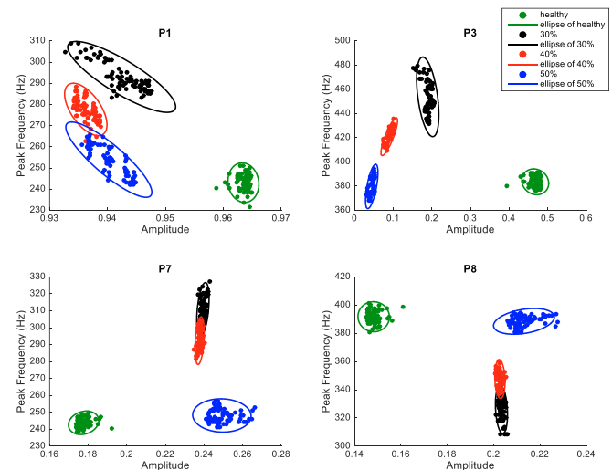
Fig. 5. The result of fault identification using the 95% confidence ellipses.
