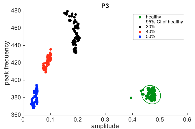
Fig. 3. An example of fault detection based on the channels P3, where the ellipse represents the 95% confidence level of healthy behaviour.
