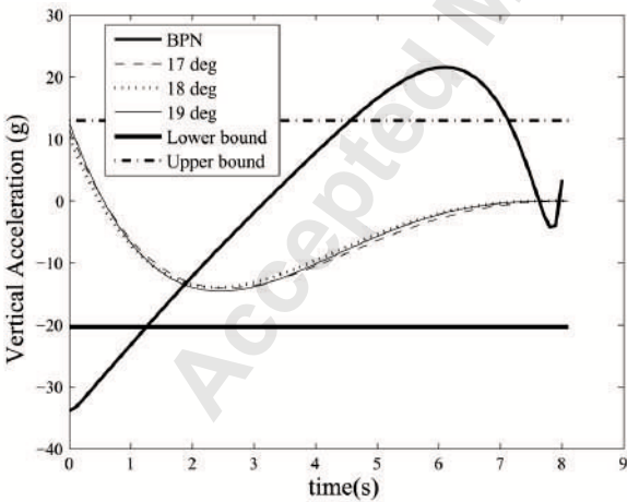
Fig. 24 Vertical Acceleration for varying bounds
