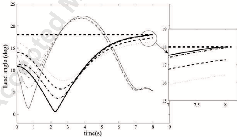
Fig. 22 Lead angle with varying \Psi_m
