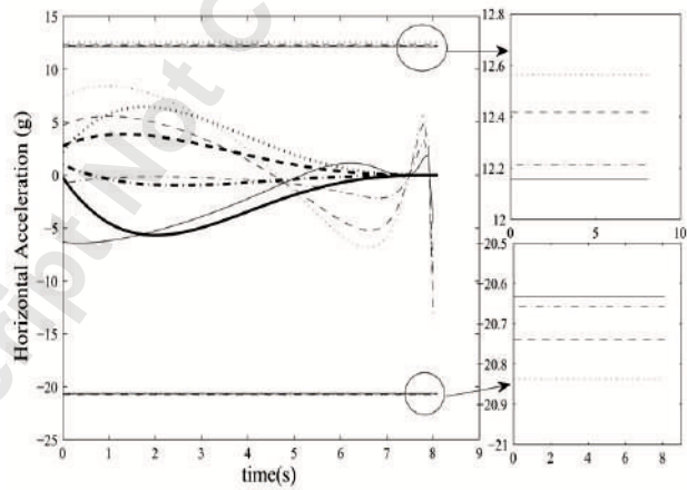
Fig. 21 Horizontal Acceleration with varying \Psi_m
