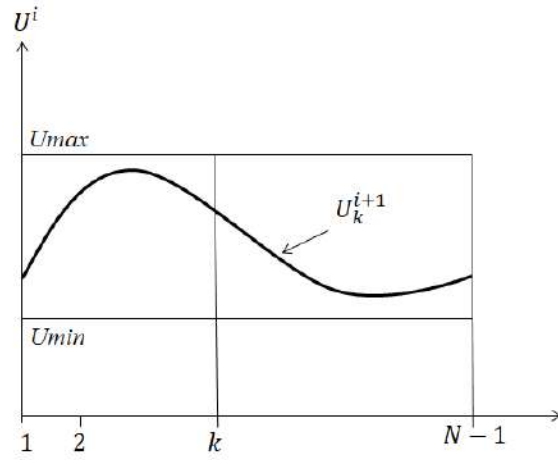
Fig. 4 Control Constraints [39]
