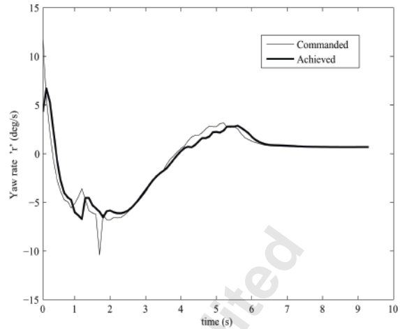
Fig. 36 Yaw rate
