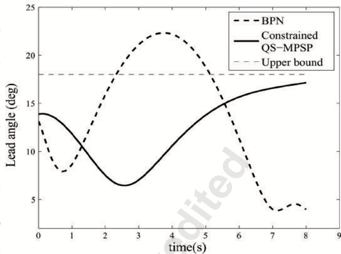
Fig. 8 Lead Angle
