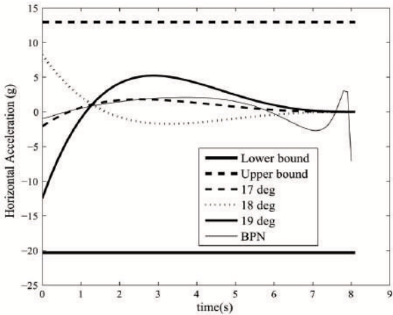
Fig. 25 Horizontal Acceleration for varying bounds
