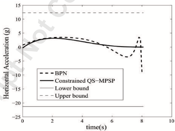
Fig. 10 Horizontal Acceleration
