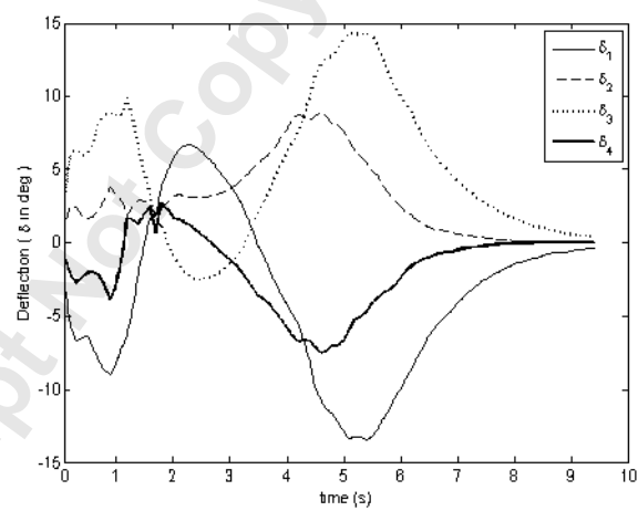
Fig. 38 Roll, pitch and yaw deflection
