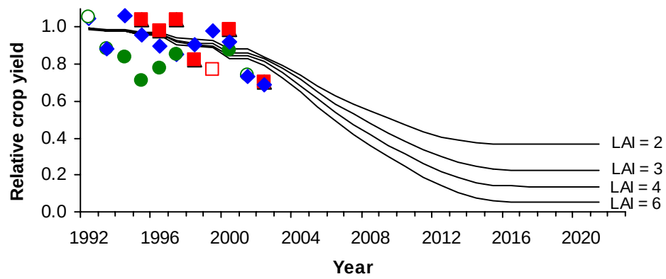
Figure 4.5 The sensitivity of crop yield relative that of a sole crop to a) light extinction coefficient 0.3-0.7 assuming an leaf area index of 4, and b) leaf area index from 2 to 6 assuming a light extinction coefficient of 0.5, as predicted by the model (lines). Measured relative crop yields: winter crop at Cirencester ●; spring crop at Cirencester: ○; ; winter crop at Leeds ◆; spring crop at Leeds: ◇; winter crop at Silsoe: ■; spring crop at Silsoe: □
