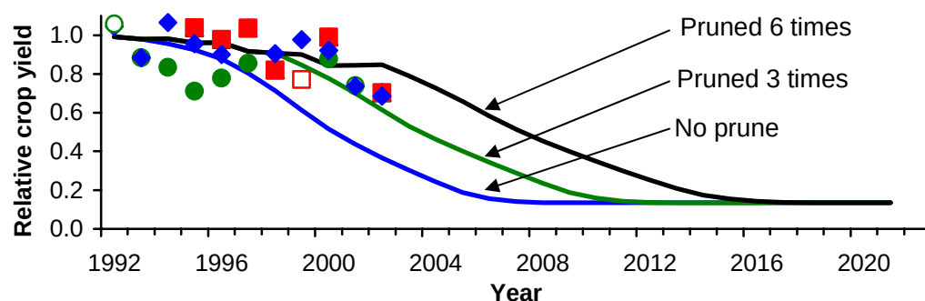
Figure 4.8 The predicted effect of pruning on crop yields relative to that of a sole crop with a yield class of 9 (assuming a leaf area index of 4 and a light extinction coefficient of 0.5). Actual relative yields at each of the three sites in each year: winter crop at Cirencester ●; spring crop at Cirencester: ○; winter crop at Leeds ◆; spring crop at Leeds: ◇; winter crop at Silsoe: ■; spring crop at Silsoe: □.
