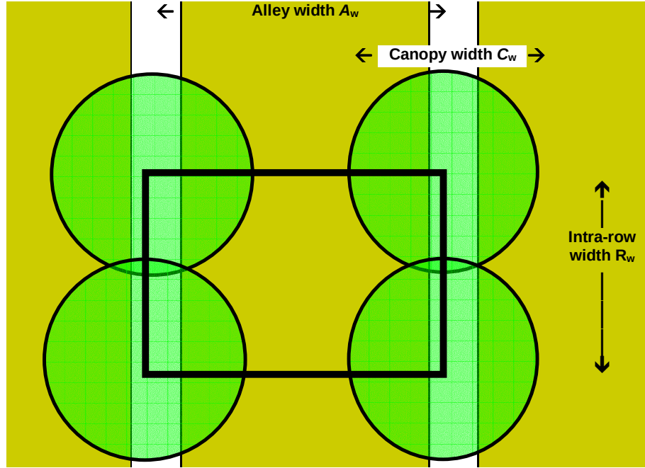
Figure 4.4 Calculation of the projected area of the canopy. Yellow = alley; white = tree row understorey; green = tree.
