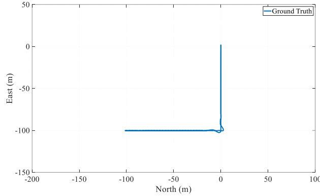
Figure 10: Ground Truth UAV Trajectory for Simulation
