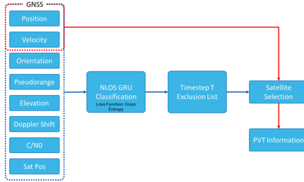
Figure 7: Multipath Detection and Exclusion
