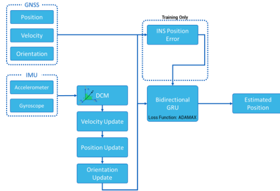
Figure 6: INS Error Correction Algorithm
