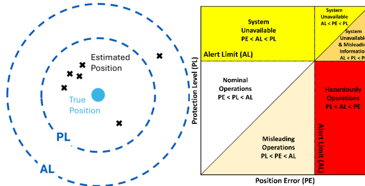
Figure 1: Illustration of the Relationship between Estimated, True Position, and Required Integrity Levels.
