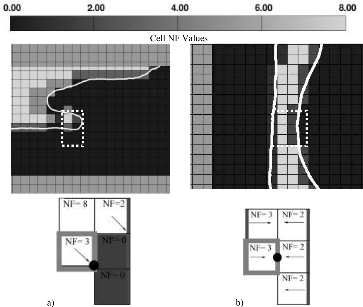
Figure 2. Example of entrainment logic. (Arrows represent velocity vector) a) Returning wave as seen in Figure 8. b) Colliding fronts as seen in Figure 6b.
