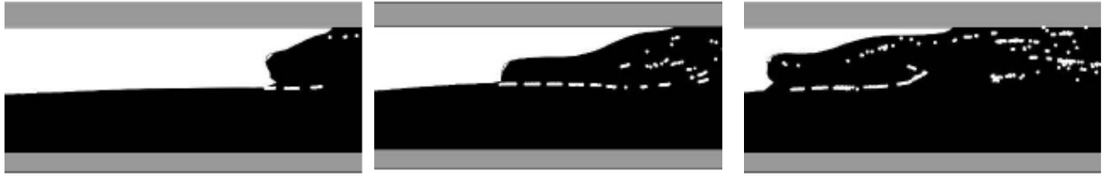
Figure 8. Entraining return wave propagating along the channel showing marker particles
