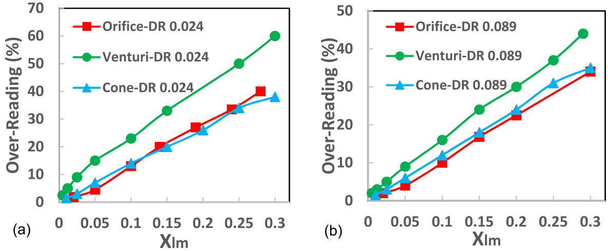
Fig. 10. Comparison of orifice, Venturi, and Cone meter in a horizontal orientation at different pressures a) 15 bar b) 60 bar.
