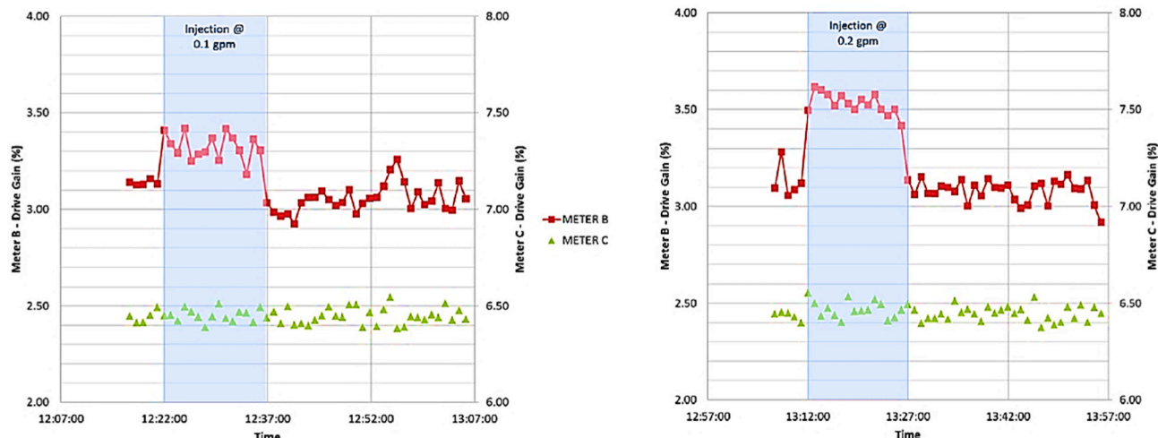
Fig. 11. Drive gain response, 0.1gpm liquid, 0.2gpm liquid injection [85].
