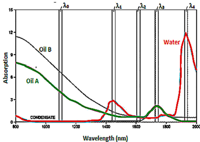
Fig. 20. NIR Absorption spectrum of water and oil [2].
