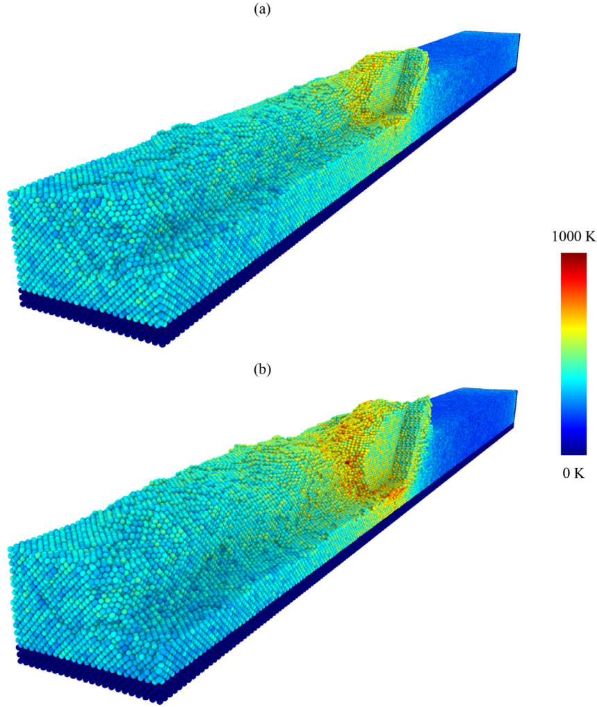
Fig. 14. Workpiece temperature for (a) k_g = 0.00125 nN/Å and (b) k_g = 0.02 nN/Å at N_{ts} = 400,000 .
