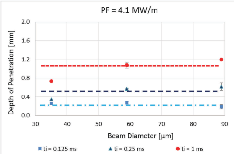
FIGURE 3 Graph showing the effect of the beam diameter on the depth of penetration of CW processing of stainless steel at different interaction times and a constant power of 4.1 MW/m.
