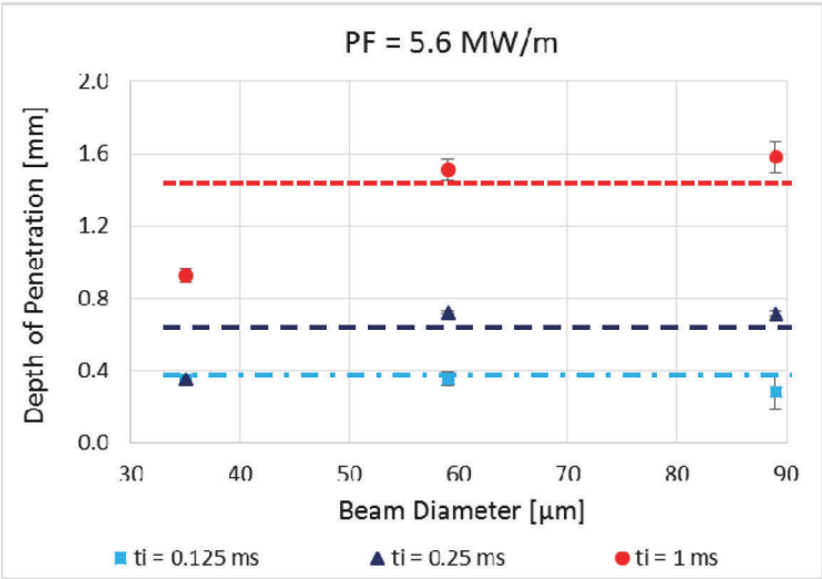
FIGURE 2 Graph showing the effect of the beam diameter on the depth of penetration of CW processing of stainless steel at different interaction times and a constant power of 5.6 MW/m.
