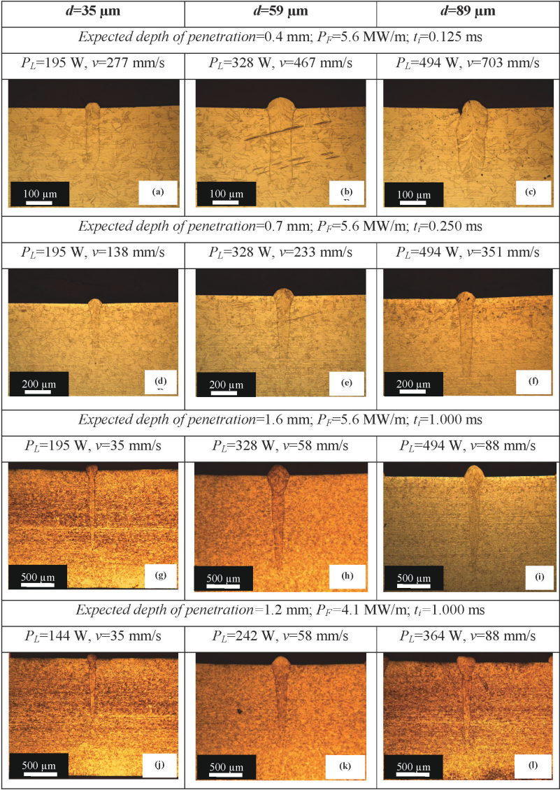
FIGURE 6 Optical micrographs showing constant combinations of power factor and interaction time for different weld depths expected when CW laser microwelding stainless steel.
