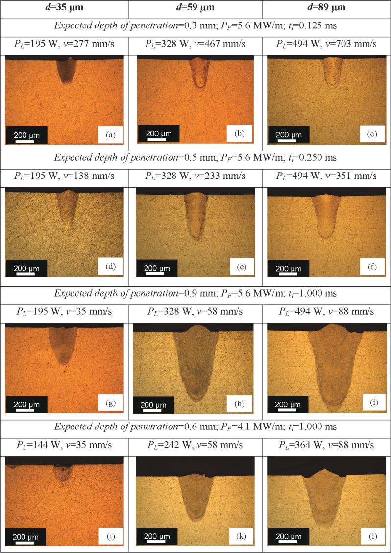
FIGURE 11 Optical micrographs showing constant combinations of power factor and interaction time for different weld depths when CW laser microwelding aluminium.
