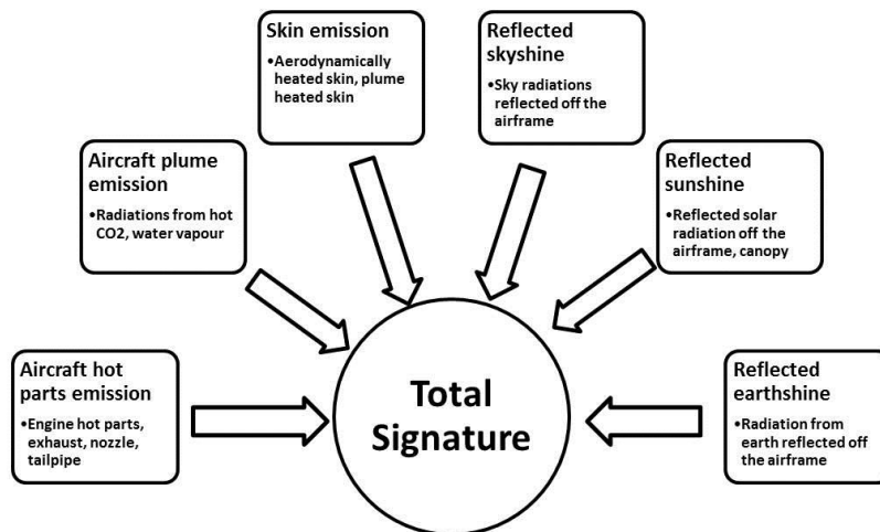
Figure 9. Contributors to an aircraft's total IR signature.
