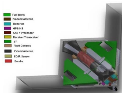
Figure 18. Cerberus UCAV systems arrangement.
