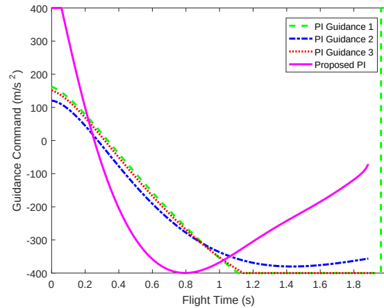
Fig. 8: The acceleration command of different guidance laws.
