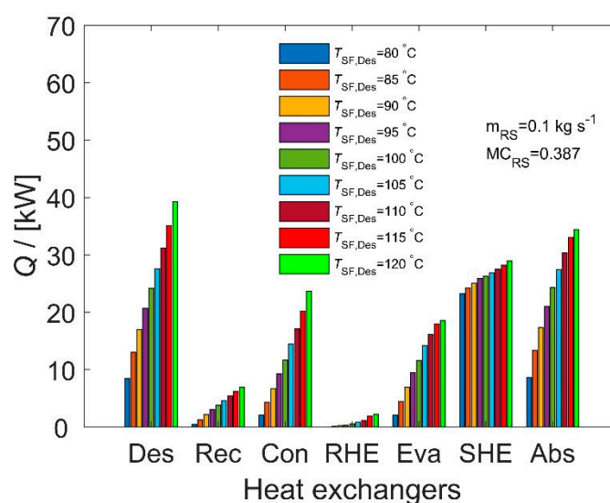
Figure 8. Heat exchanger loads as functions of heat source temperature for the rich solution of 0.1 kg s −1 and 0.387.
