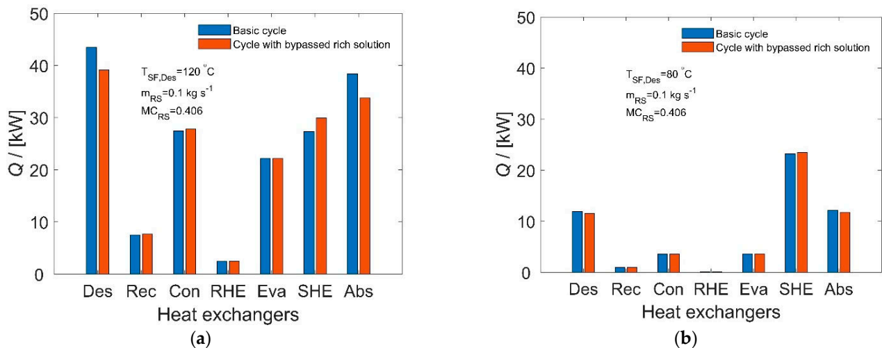
Figure 14. Heat exchanger loads of cycle with bypassed rich solution and basic cycle for different heat source temperature. (a) 120 °C, (b) 80 °C.
