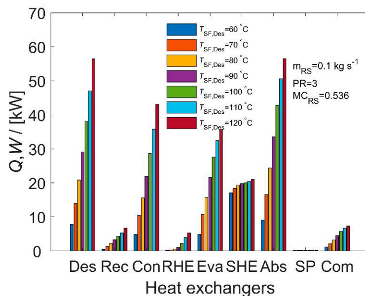
Figure 11. Heat exchanger loads and power consumption as functions of heat source temperature for the pressure ratio of 3.
