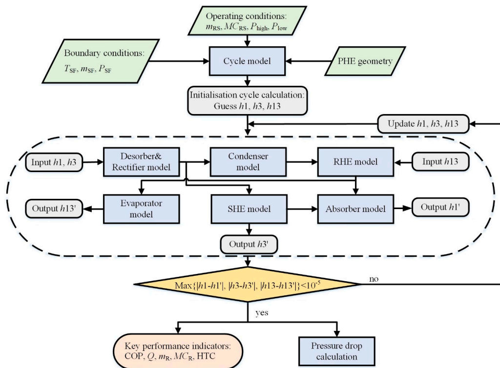
Figure 5. Simulation platform of the integrated cycle model and heat exchanger models.
