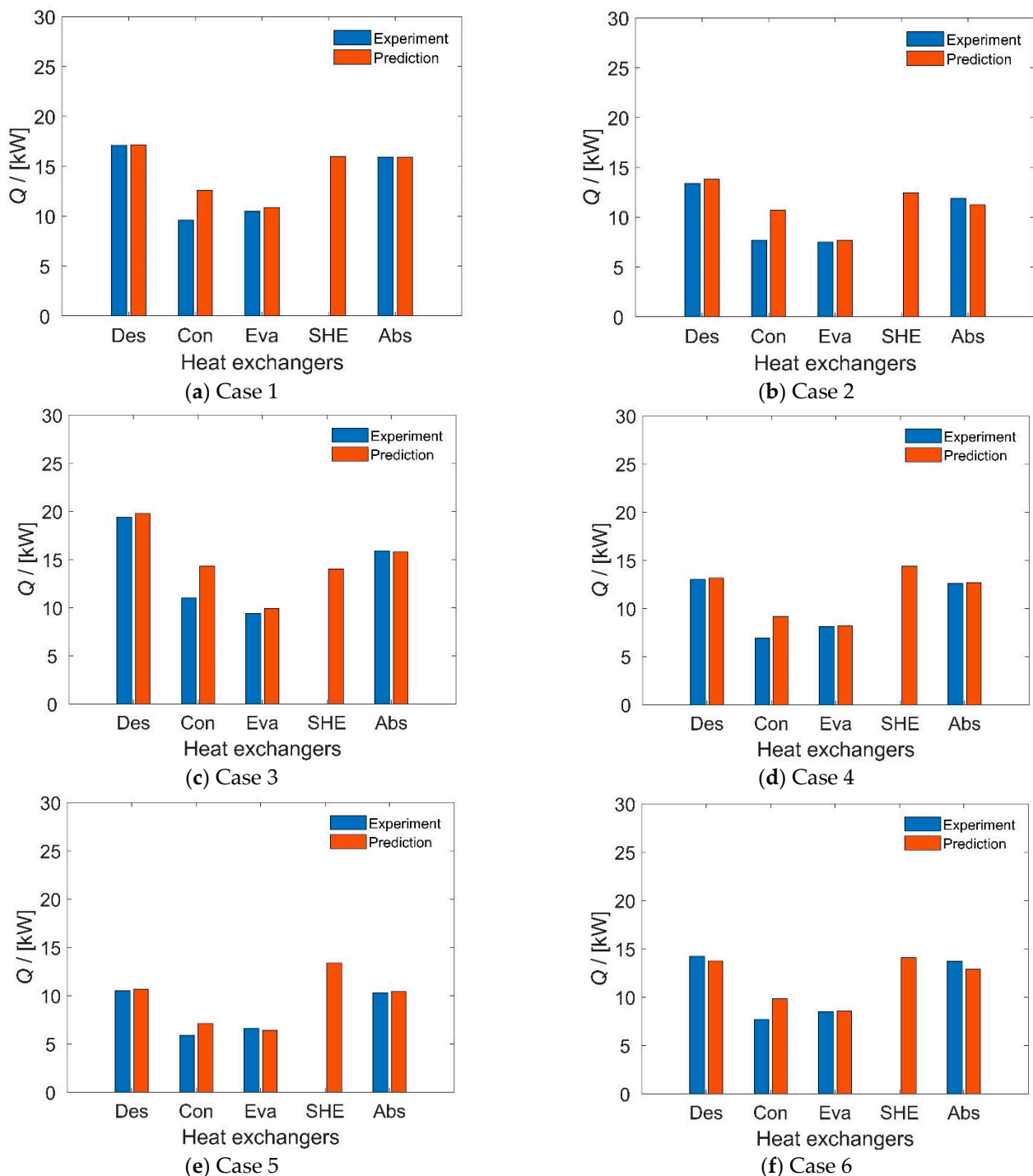
Figure 6. Comparison of the predicted heat loads through this study with the experimental data of Le Lostec et al. [19] for (a) Case 1, (b) Case 2, (c) Case 3, (d) Case 4, (e) Case 5, (f) Case 6.
