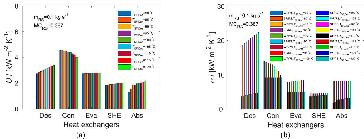
Figure 9. Overall HTCs (a) and two sides HTCs (b) of the heat exchangers for the rich solutions of 0.1 \text{ kg s}^{-1} and mass concentration 0.387. For Des, Con, Eva and Abs, the two sides are working fluid (WF) and secondary fluid (SF). For SHE, the two sides are poor solution (PS) and rich solution (RS).
