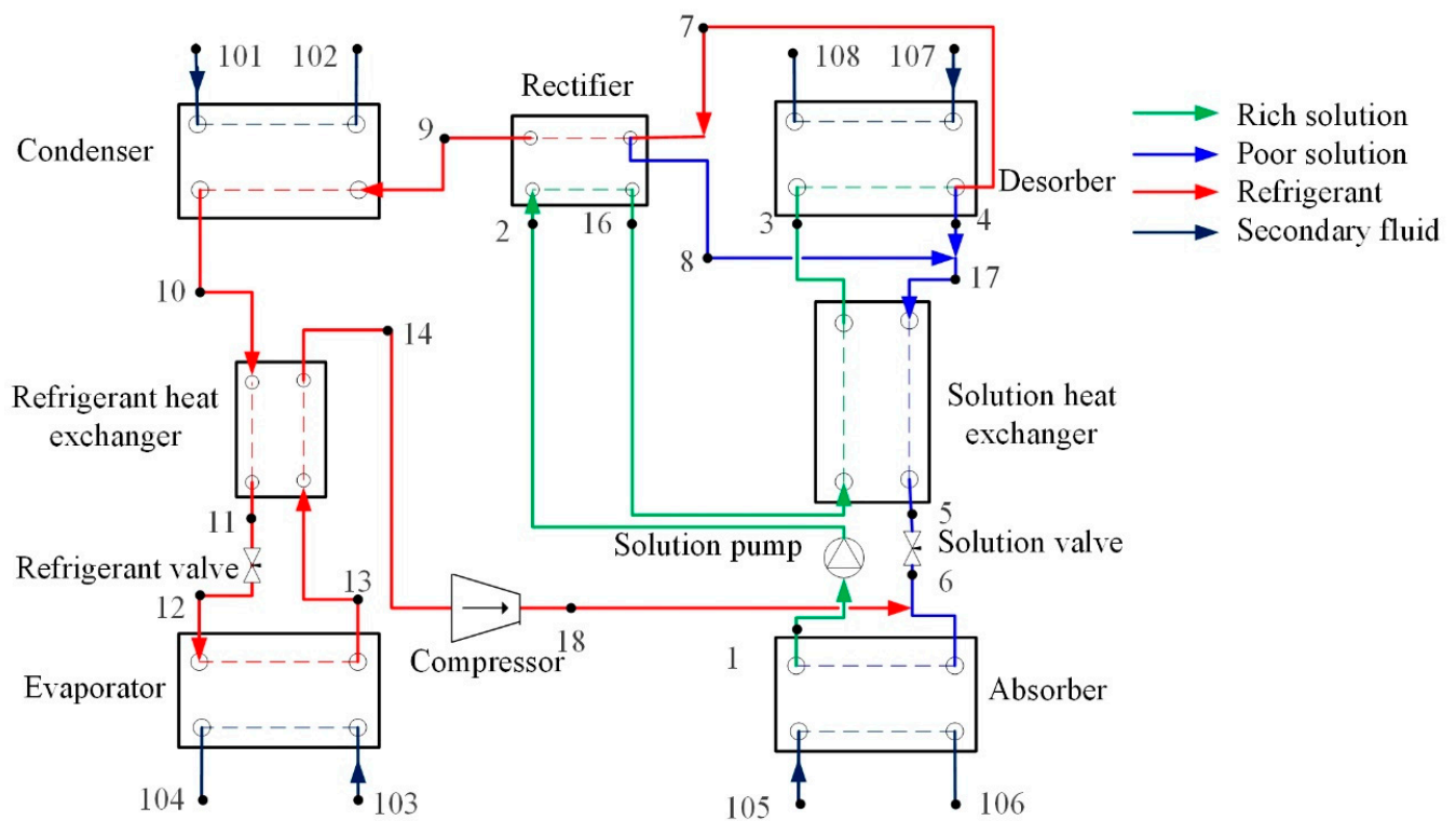
Figure 2. Flow diagram of compression-assisted ammonia/water absorption cycle.
