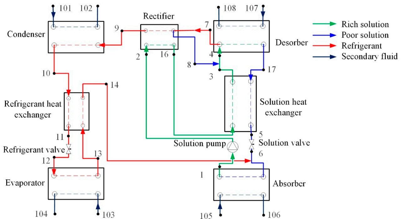
Figure 3. Flow diagram of ammonia/water absorption cycle with counter-current desorber.
