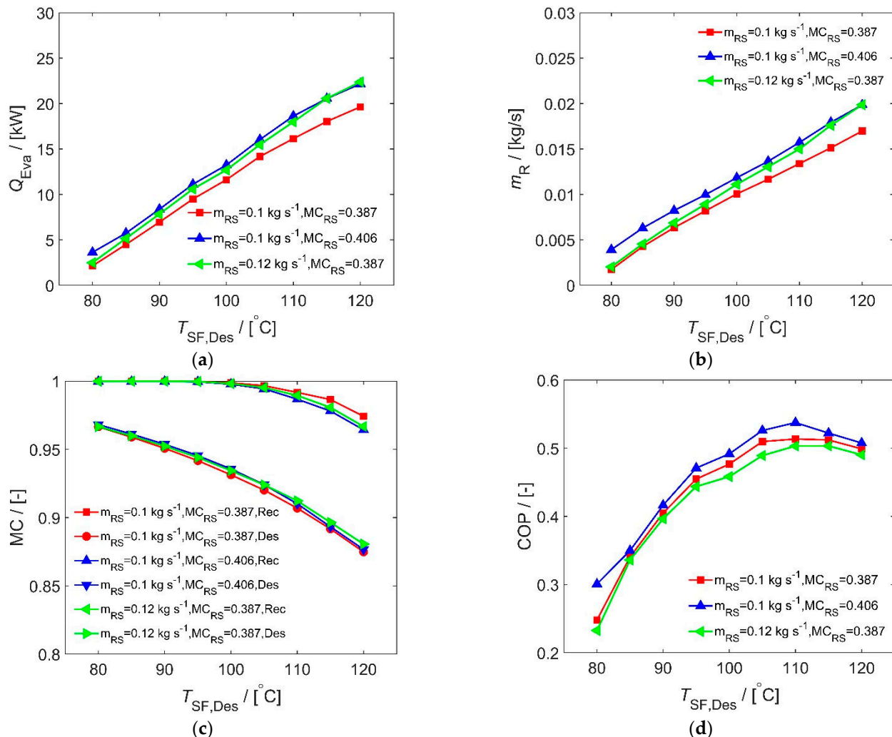
Figure 7. Performances of basic cycle as a function of heat source temperature, the mass flow rate and mass concentration of the rich solution. Cycle performances are (a) Cooling capacity, (b) Refrigerant mass flow rate, (c) Vapour mass concentration at the outlet of the desorber and rectifier, (d) COP.
