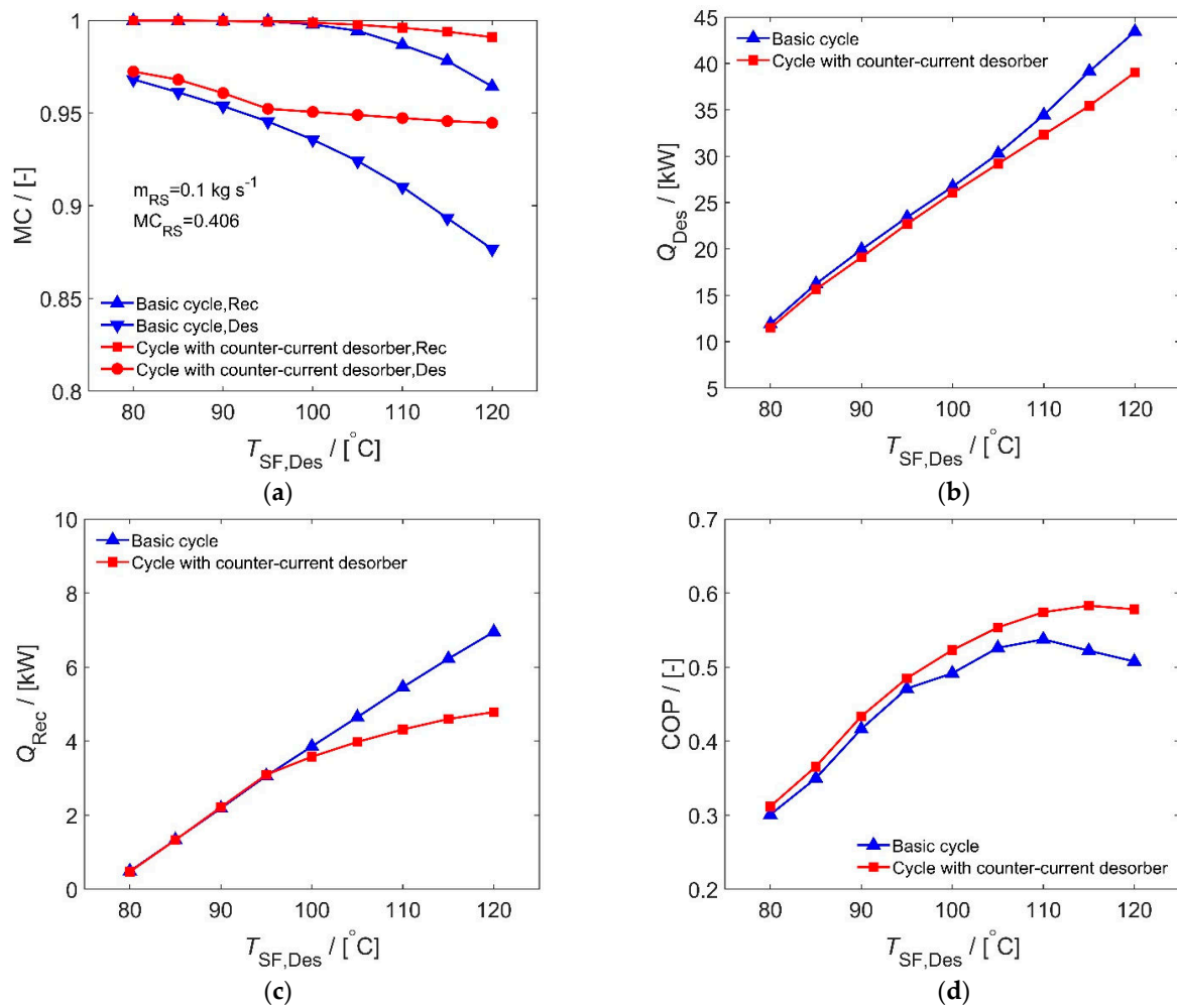
Figure 12. Performances of cycle with counter-current desorber and basic cycle as a function of heat source temperature. Cycle performances are (a) Vapour mass concentration at the outlet of the desorber and rectifier, (b) Heating capacity, (c) Heat loads of the rectifier, (d) COP.
