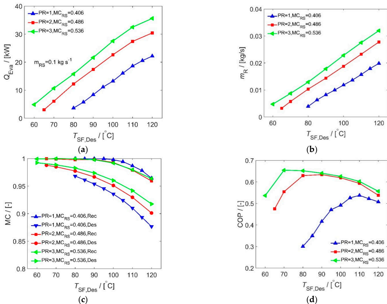
Figure 10. Performances of compression-assisted cycle as a function of heat source temperature and pressure ratio. Cycle performances are (a) Cooling capacity, (b) Refrigerant mass flow rate, (c) Vapour mass concentration at the outlet of the desorber and rectifier, (d) COP.
