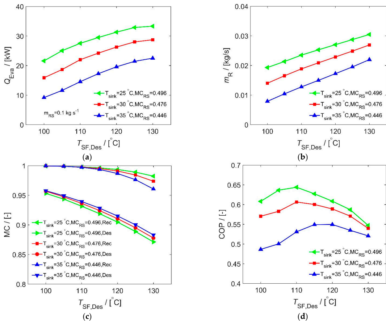
Figure 16. Cycle performances as a function of heat source temperature and heat sink temperature. Cycle performances are (a) Cooling capacity, (b) Refrigerant mass flow rate, (c) Vapour mass concentration at the outlet of the desorber and rectifier, (d) COP.
