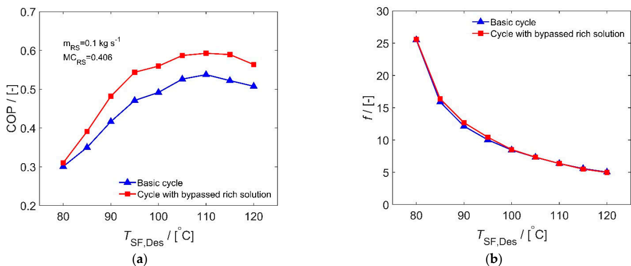
Figure 13. Performances of cycle with bypassed rich solution and basic cycle as a function of heat source temperature. Cycle performances are (a) COP, (b) Solution circulation ratio.
