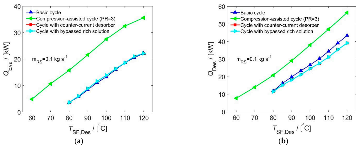
Figure 15. Performance comparison of different cycles. (a) Cooling capacity, (b) Heating capacity.
