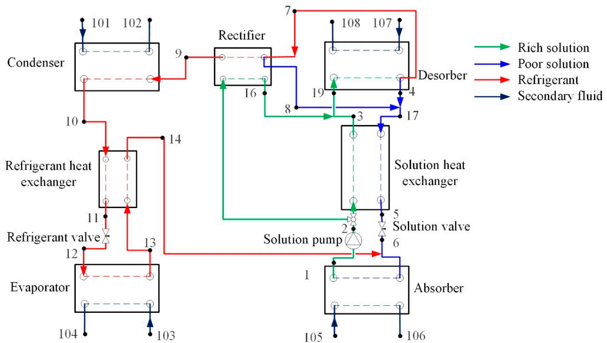
Figure 4. Flow diagram of ammonia/water absorption cycle with bypassed rich solution.
