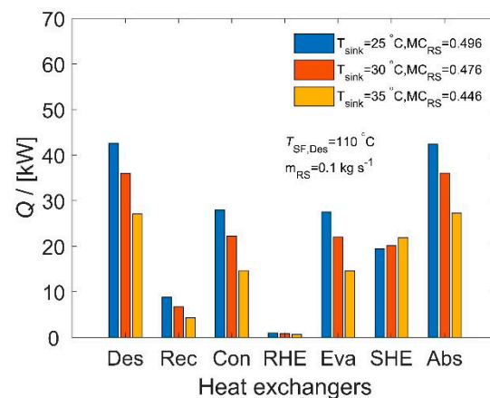
Figure 17. Heat exchanger loads as a function of heat sink temperature.
