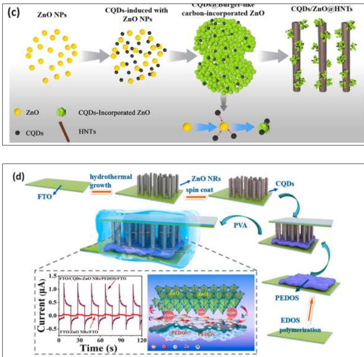
Figure 4. (a) Nitrogen-doped carbon quantum dot (N-CQD) decorated ZnO nanorods, Adopted with permission from [57], (b) N-doped CQDs/Ni-doped ZnO nanocomposites for visible light photodegradation of organic pollutants, Adopted with permission from [62], (c) Formation of CQDs/ZnO@HNTs in a stepwise synthetic process, Adopted with permission from [50], and (d) Organic-inorganic face-to-face ZnO nanorod-based self-powered UV photodetector enhanced by carbon quantum dots, Adopted with permission from [48].
