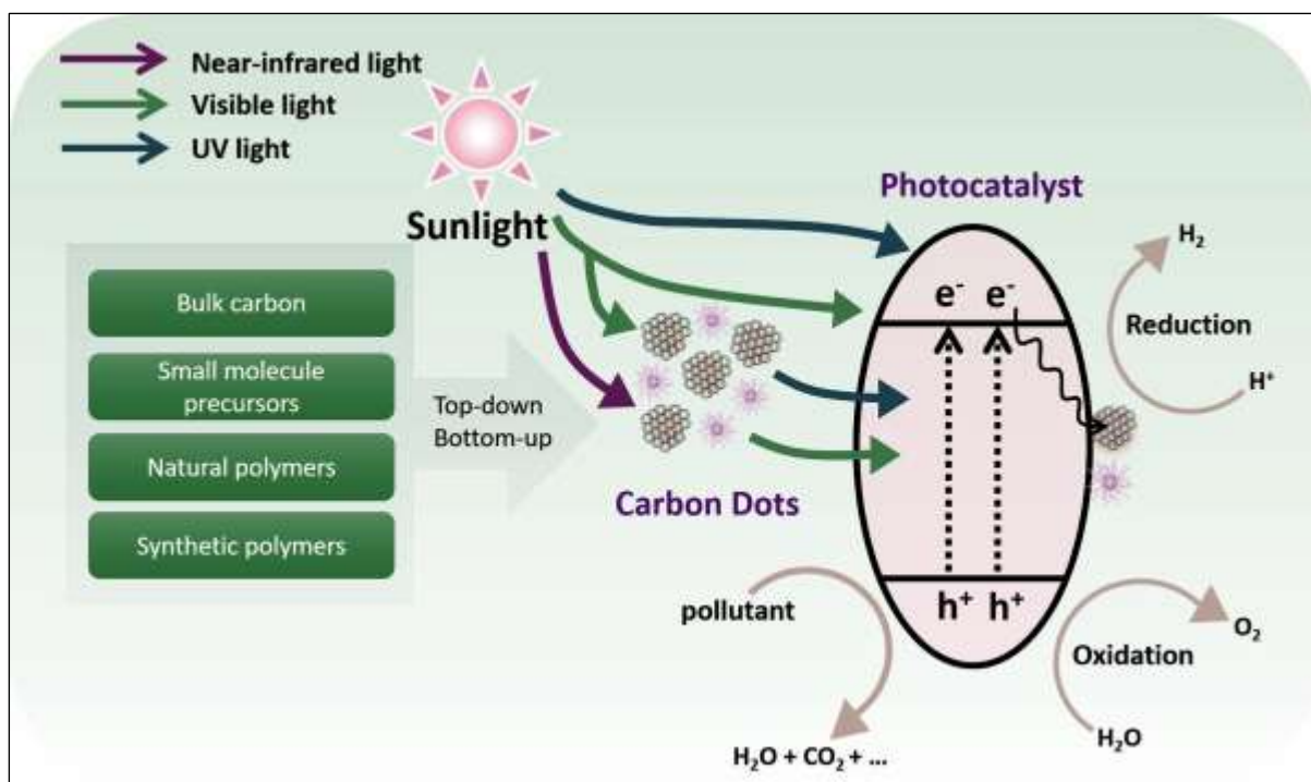
Figure 12: Combination of CDs and ZnO in nanocomposites for photocatalytic activity, particularly in the degradation of dyes and gas-phase pollutants, Adopted with permission from [130].
