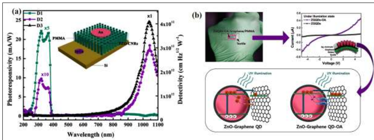
Figure 20. (a) Self-powered \text{TeO}_2 -doped ZnO composite nanorods/Si heterojunction photodetectors with distinct responses to UV and NIR lights, Adopted with permission from [203], (b) Transparent and flexible UV photodetector with ZnO@graphene quantum dots (ZGQDs) on eco-friendly keratin textile, Adopted with permission from [201,202].
