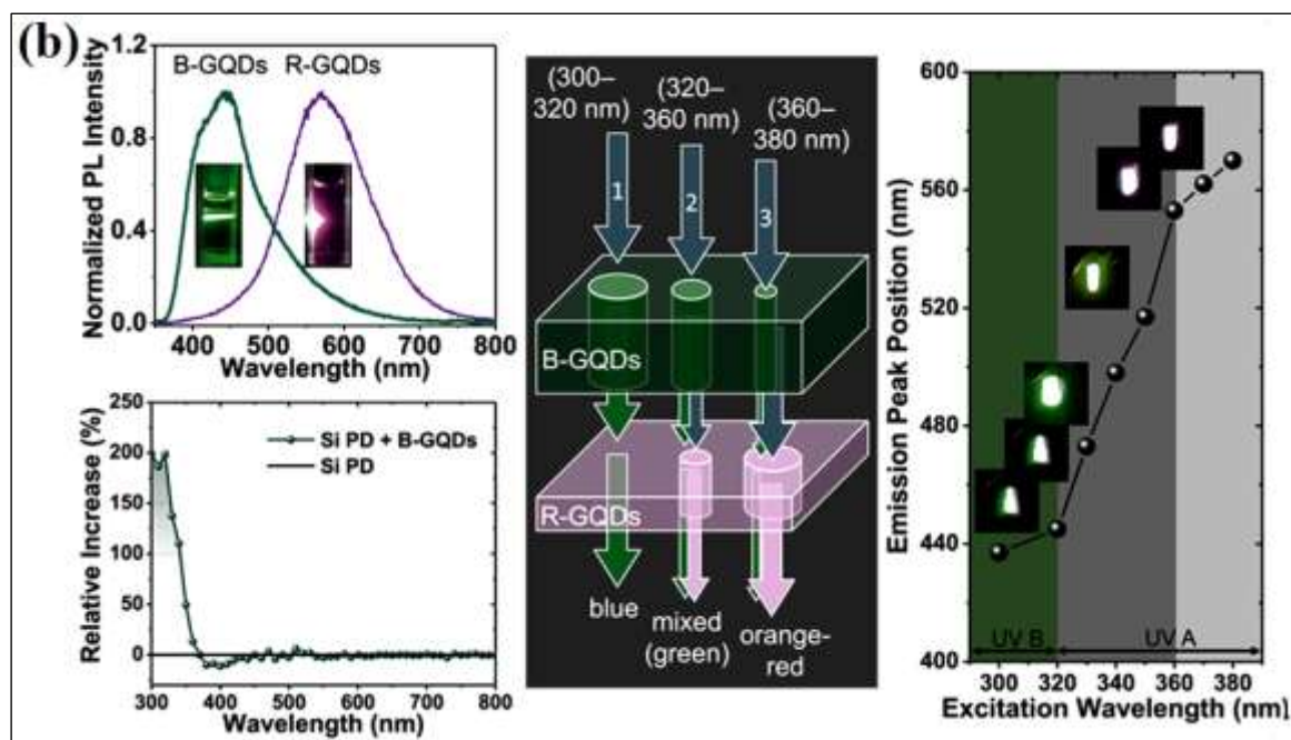
Figure 19. (a) Schematic representation of the polymer-based photodetector utilising ZnO@graphene quantum dots (GQDs) in a Poly (vinyl alcohol) matrix, Adopted with permission from [199], (b) UV detection with graphene quantum dots (GQDs): Solution-processed GQDs sensitise Si photodiodes, extending responsiveness down to 300 nm, and facilitating visible responses to UV excitation, Adopted with permission from [200].
