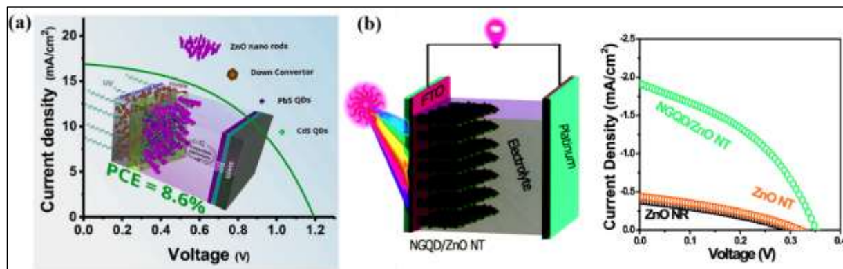
Figure 16. (a) Cost-effective architecture for PbS/CdS quantum dots sensitised ZnO nanorods array solar cells by using down-converting glass as a substrate, enhancing the absorption spectrum, Adopted with permission from [168], (b) ZnO nanotapers arrays grown on FTO-coated glass substrates using the hydrothermal method with nitrogen-doped graphene quantum dots (NGQDs) sensitised nanotaper photoanodes in quantum dot-sensitised solar cells, Adopted with permission from [171].
