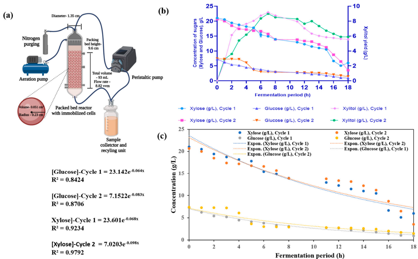
Figure 6. (a) Packed bed reactor (PBR) for immobilized cell-based fermentation. (b) Fermentation profile of hemicellulosic hydrolysate for xylitol production under microaerophilic immobilized-cell conditions. (c) Substrate (glucose and xylose) consumption profile (based on first-order rate).
