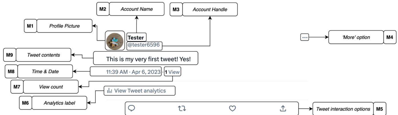
Fig. 40. Twitter CR markup showing 9 'marks' for authentication.
