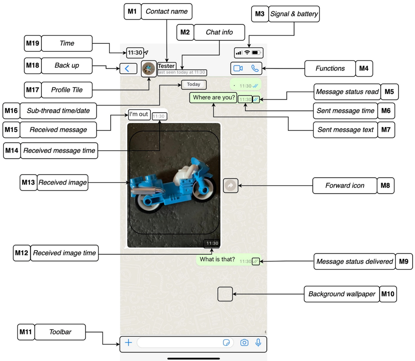
Fig. 2. WhatsApp CR markup on iOS showing 19 'marks' for authentication.
