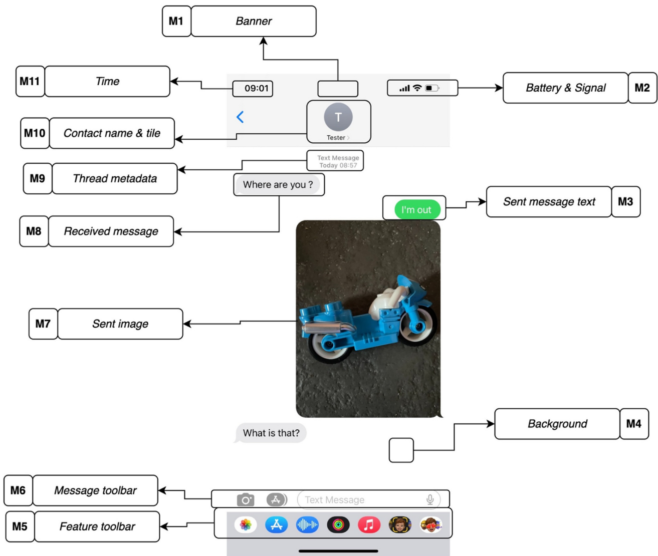
Fig. 30. iMessage CR markup showing 15 'marks' for authentication.
