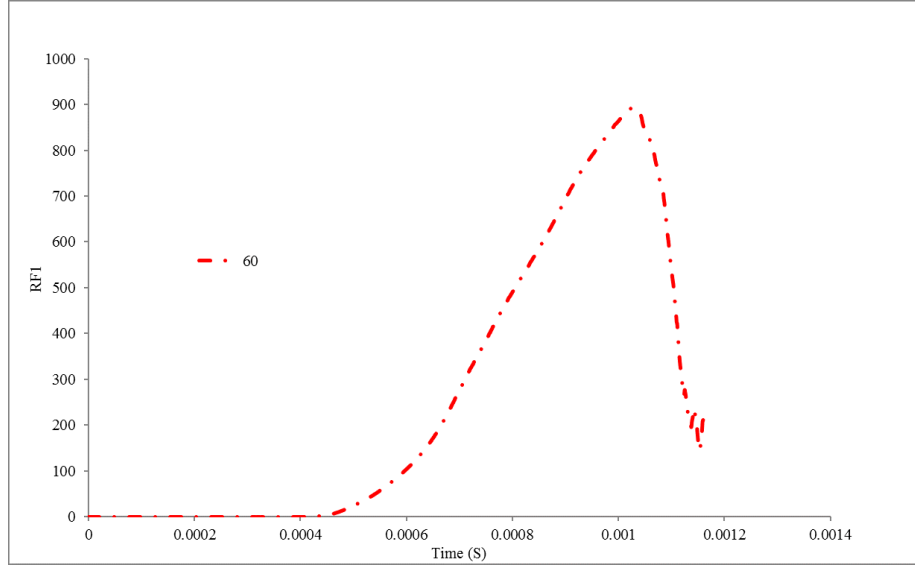
Figure 18: Reaction forces versus time under dynamic conditions for 60^\circ laminate.
