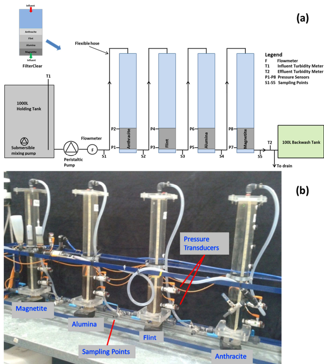
Figure 1: (a) Schematic and (b) photograph of the pilot filter rig.
