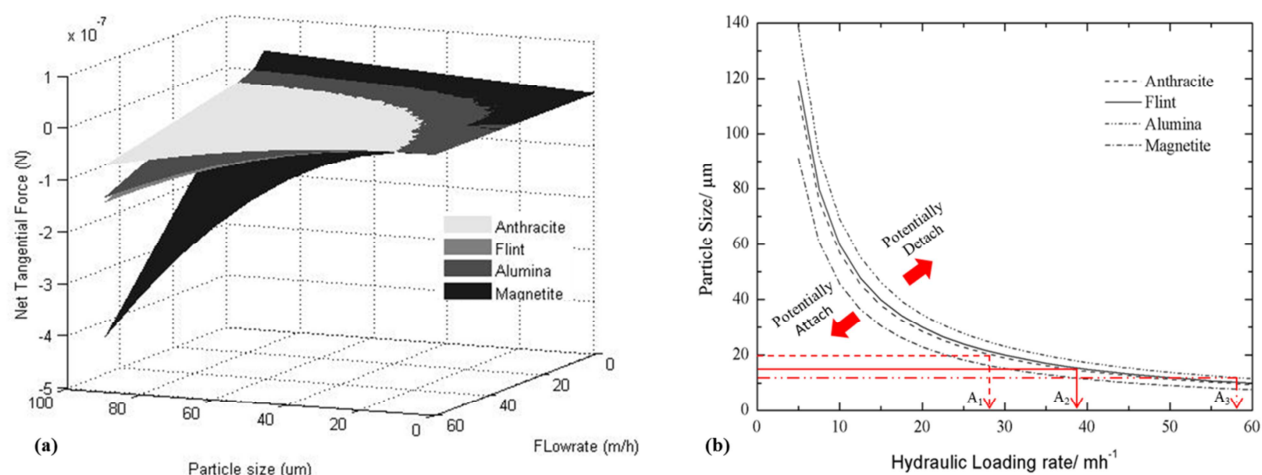
Figure 6: Modelled net tangential force (equation (3) and (4)) in a clean bed ( \sigma = 0 ) (a) 3D plot for the different particle sizes and HLRs in the four media layers, (b) Plot of the particle sizes and HLR when the net tangential force is zero for the four layers ( k_f = 3.79 \times 10^{-6} \text{ m} from Bai and Tien (1997), H = 1.4 \times 10^{-20} \text{ kgm}^2\text{s}^{-2} and \delta = 3 \times 10^{-10} \text{ m}^{24} , \mu = 0.000955 \text{ kgm}^{-1}\text{s}^{-1} and the parameters defined in Materials and Methods were used in the simulation).
