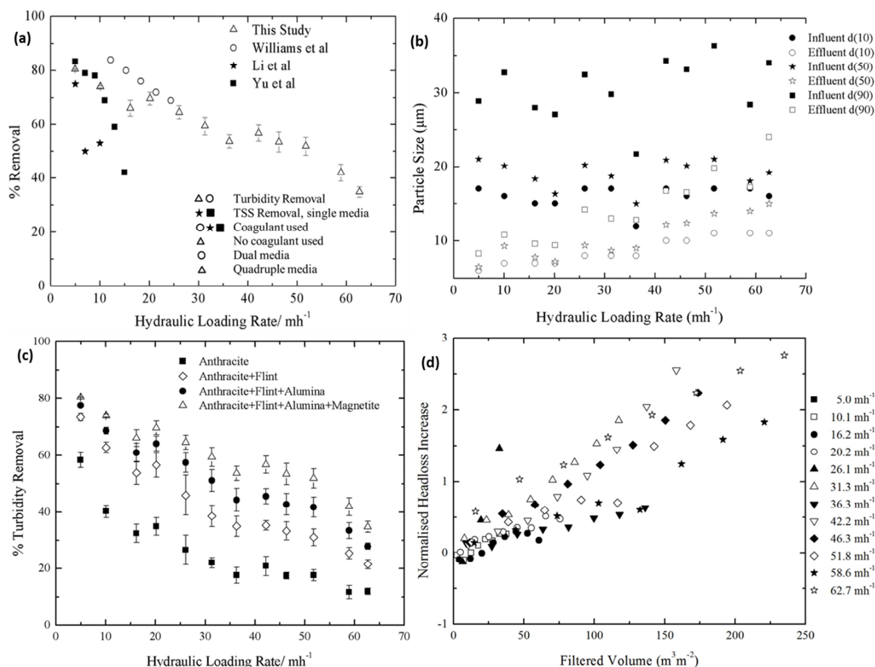
Figure 2: (a) Overall turbidity removal efficiency in this study and comparable data from previous studies, (b) d(10), d(50), d(90) particle sizes for both the influent and effluent at different HLRs. (c) The impact of HLR on the average filter turbidity removal efficiency for the quadruple (anthracite, flint, alumina and magnetite) filter, tri-media (anthracite, flint and alumina) filter, dual-media (anthracite and flint) filter and the mono-media (anthracite) filter, (d) Change in NHL increase with filtered volume at different HLRs.
