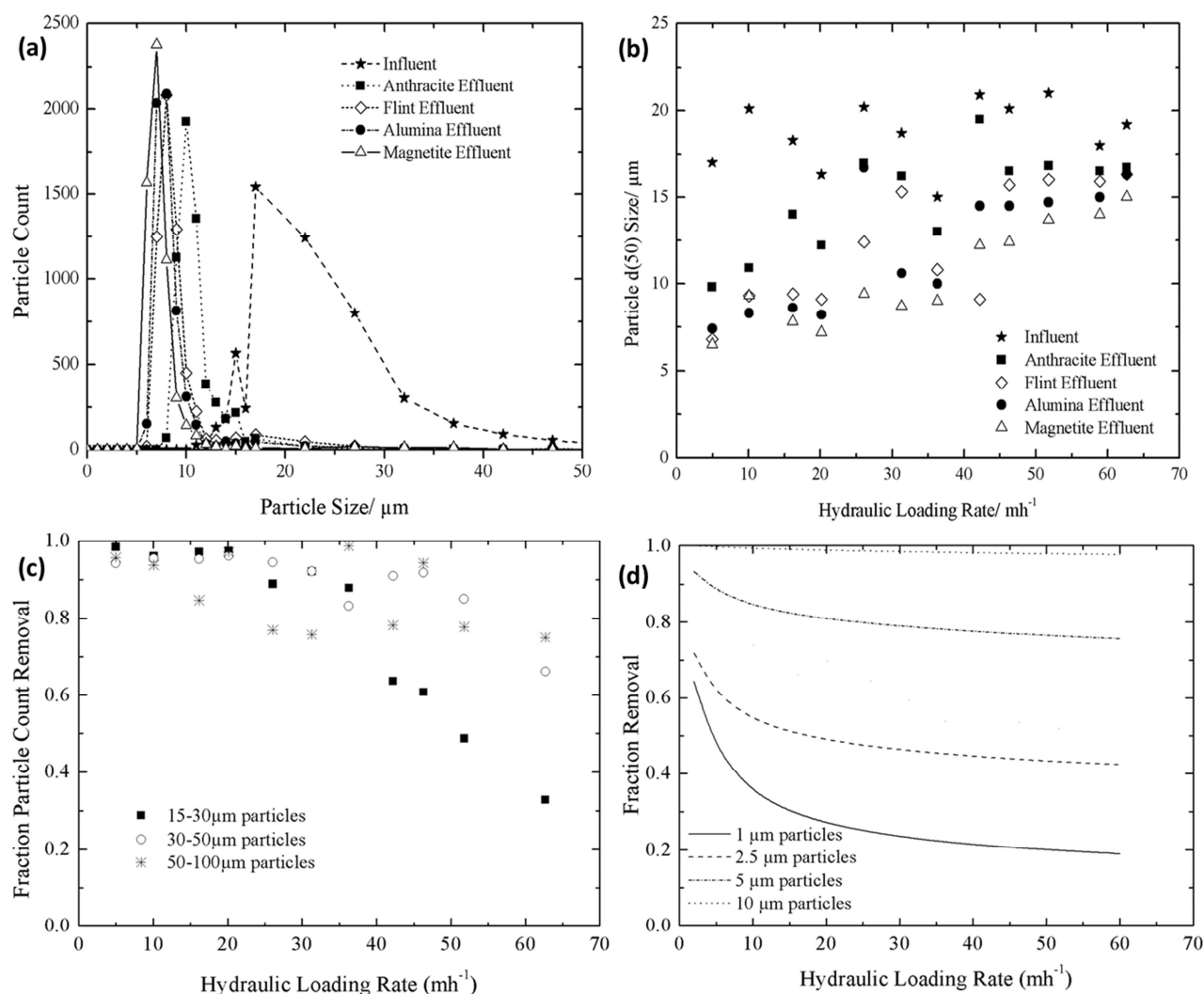
Figure 5: (a) Typical PSDs of the wastewater at different stages through the filter (for the 5 \text{mh}^{-1} filter run), (b) The average size of particles passing through each filter stage at different HLRs, (c) Overall removal of 15-30 \mu\text{m} , 30-50 \mu\text{m} and 50-100 \mu\text{m} particles, (d) The TE model plots for the particle sizes 1, 2.5, 5 and 10 \mu\text{m} .
