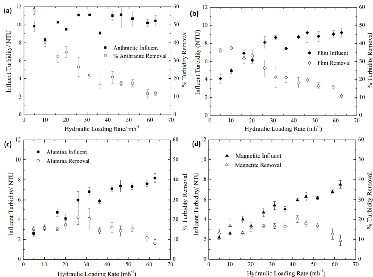
Figure 3: Turbidity removal for each media at different HLRs and the turbidity influent to each layer.
