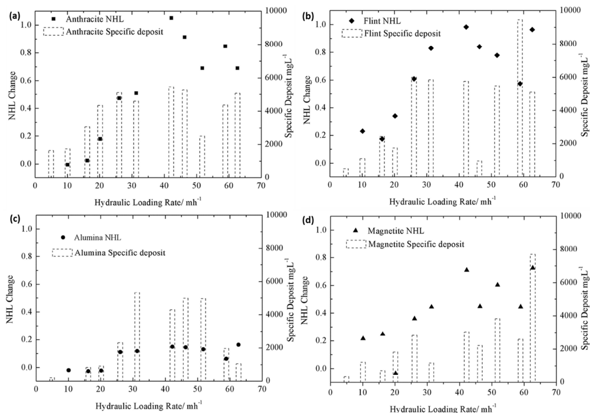
Figure 4: NHL change and specific deposit at different filtration rates for the four media.
