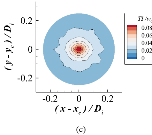
Figure 3: Flow field of wing-tip vortex in freestream flow, Re_v = 1.6Re_{v,ref} , (a) Tangential velocity ( V_\theta/w_0 ), (b) Streamwise vorticity ( \omega_z D_i/w_0 ), (c) Turbulence intensity ( TI/w_0 )
