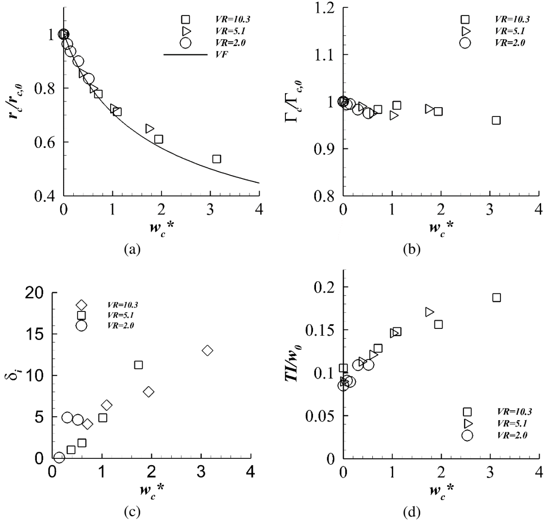
Figure 5: Data for Re_v = 1.6Re_{v,ref} , for intake velocity ratios (VR) of 10.3, 5.1 and 2.0, as a function of normalised local velocity ratio ( w_c^* = w_c/w_{c,0}-1 ), (a) Change in vortex core radius ( r_c/r_{c,0} ) compared to vortex filament (VF) theory, (b) Change in vortex core circulation ( \Gamma_c/\Gamma_{c,0} ), (c) Apparent diffusion coefficient ( \delta_i ), (d) Turbulence intensity ( TI/w_0 )
