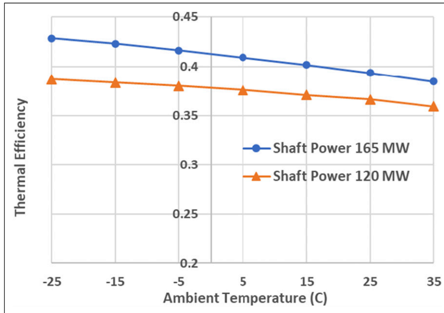
Figure 20. Thermal efficiency versus ambient temperature.
