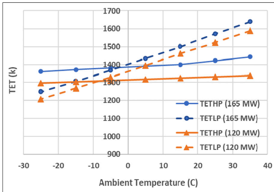
Figure 17. TETs versus ambient temperature ( P_{\text{amb}} = 1 \text{ atm} ).
