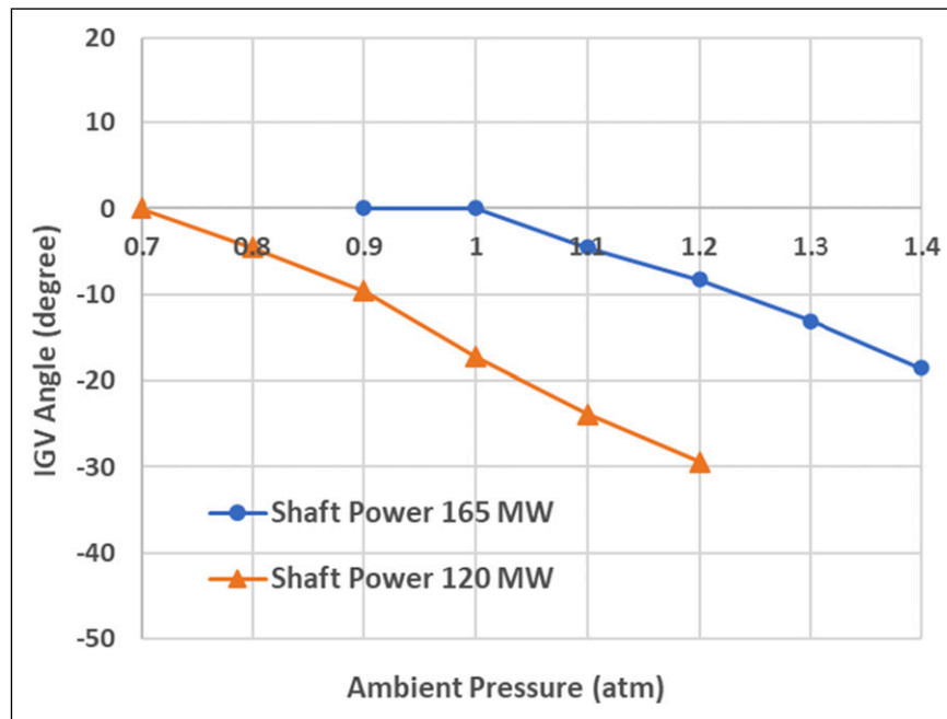
Figure 22. IGV angle versus ambient pressure.
