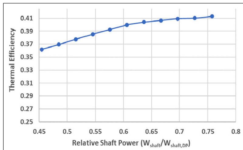
Figure 28. Thermal efficiency versus relative shaft power.
