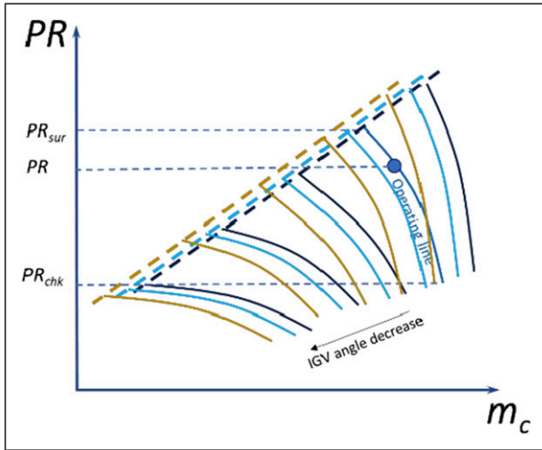
Figure 4. Characteristic map of compressor with variable IGV.
