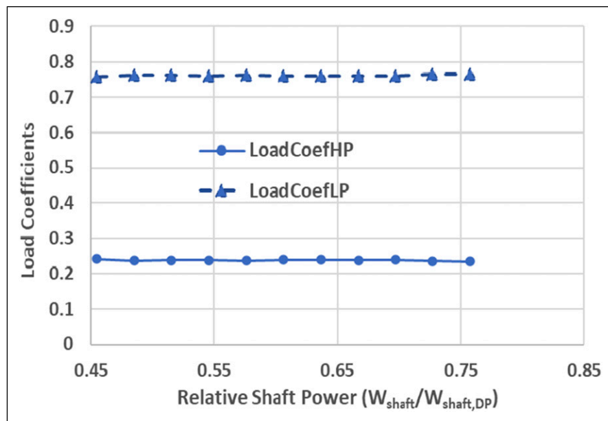
Figure 27. Load coefficients varying with relative shaft power ( T_{\text{amb}} = 5^\circ\text{C} & P_{\text{amb}} = 0.7 atm).
