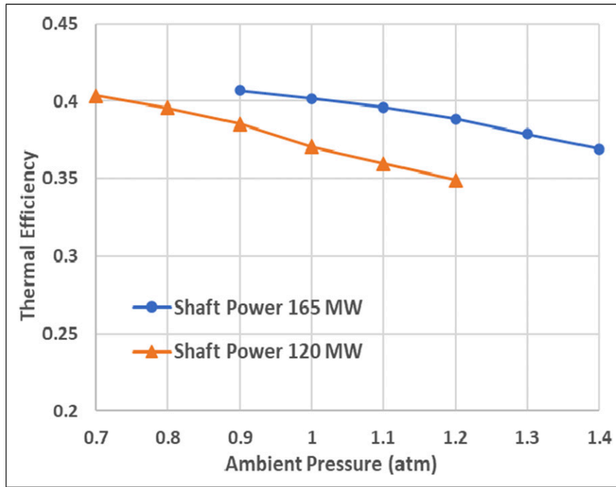
Figure 24. Thermal efficiency versus ambient pressure.
