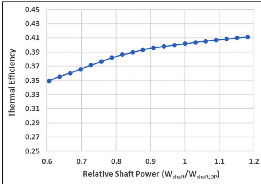
Figure 16. Thermal efficiency versus relative shaft power ( T_{\text{amb}} = 15^\circ\text{C} & P_{\text{amb}} = 1 \text{ atm} ).
