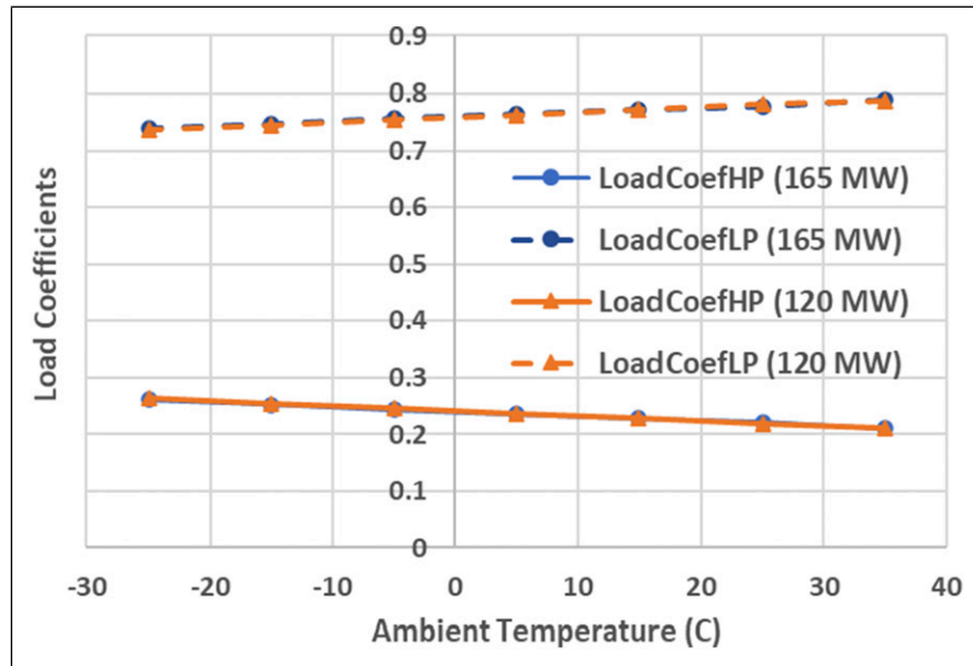
Figure 19. Load coefficients varying with ambient temperature ( P_{amb} = 1 \text{ atm} ).
