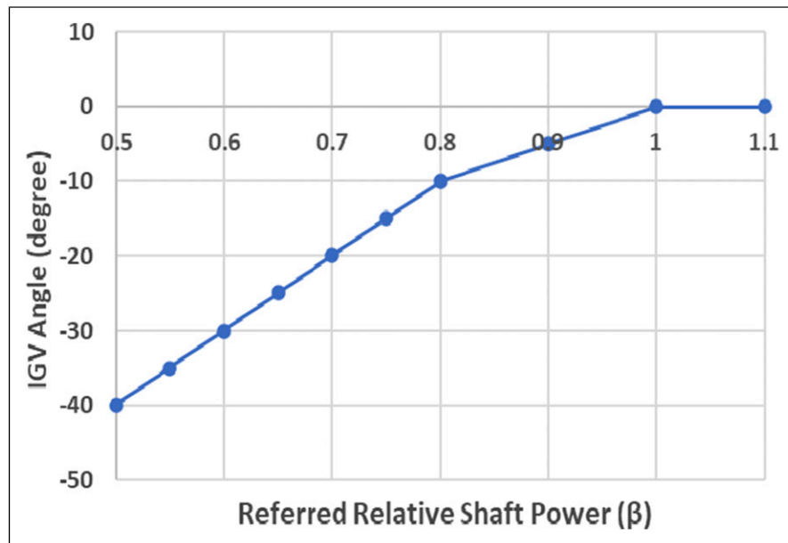
Figure 11. IGV control schedule.
