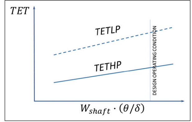
Figure 8. TETHP - W_{shaft} \cdot (\theta/\delta) control schedule.
