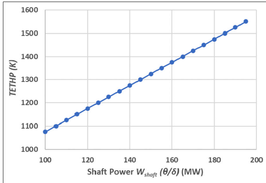
Figure 10. Off-design performance control schedule.
