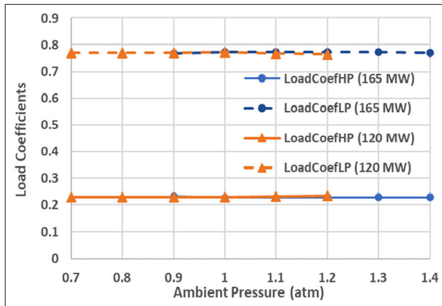
Figure 23. Load coefficient varying with ambient pressure ( T_{amb} = 288.15 K).
