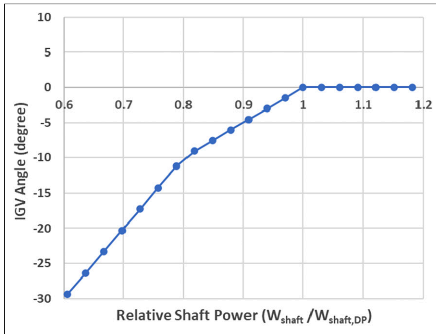
Figure 13. IGV Angle versus relative shaft power ( T_{amb} = 15^\circ\text{C} & P_{amb} = 1 \text{ atm} ).
