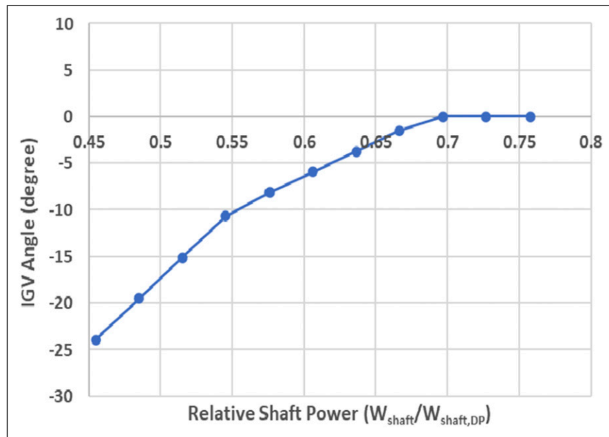
Figure 26. IGV angle versus relative shaft power.
