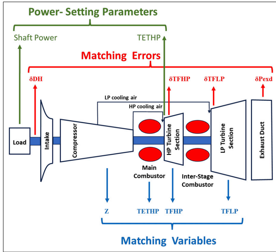
Figure 3. Model gas turbine with sequential combustors.
