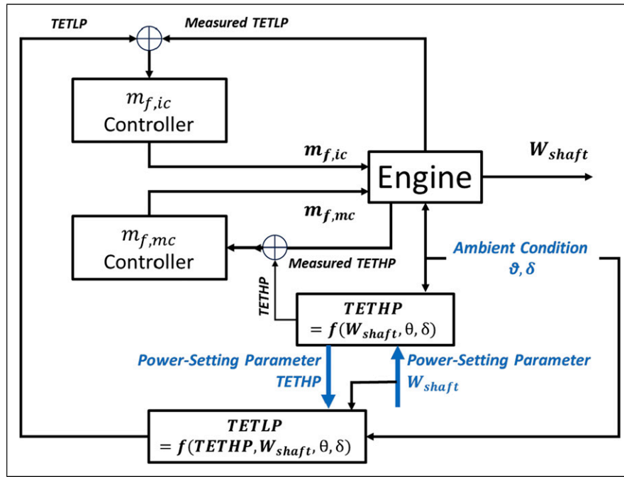
Figure 9. Schematic engine control system.
