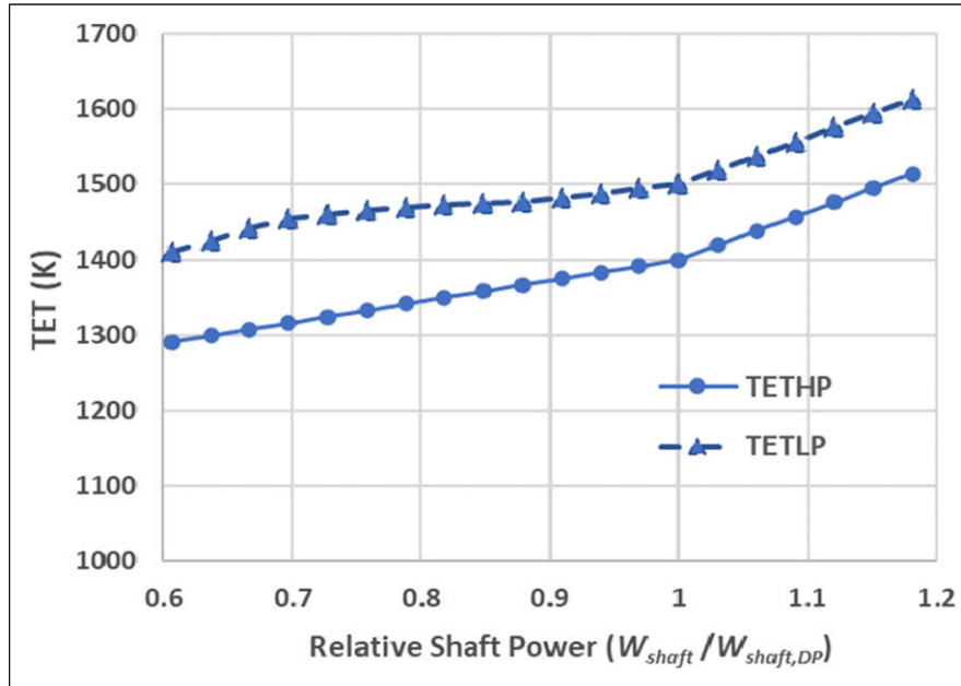
Figure 12. TETs vs relative shaft power ( T_{amb} = 15^\circ\text{C} & P_{amb} = 1 \text{ atm} ).
