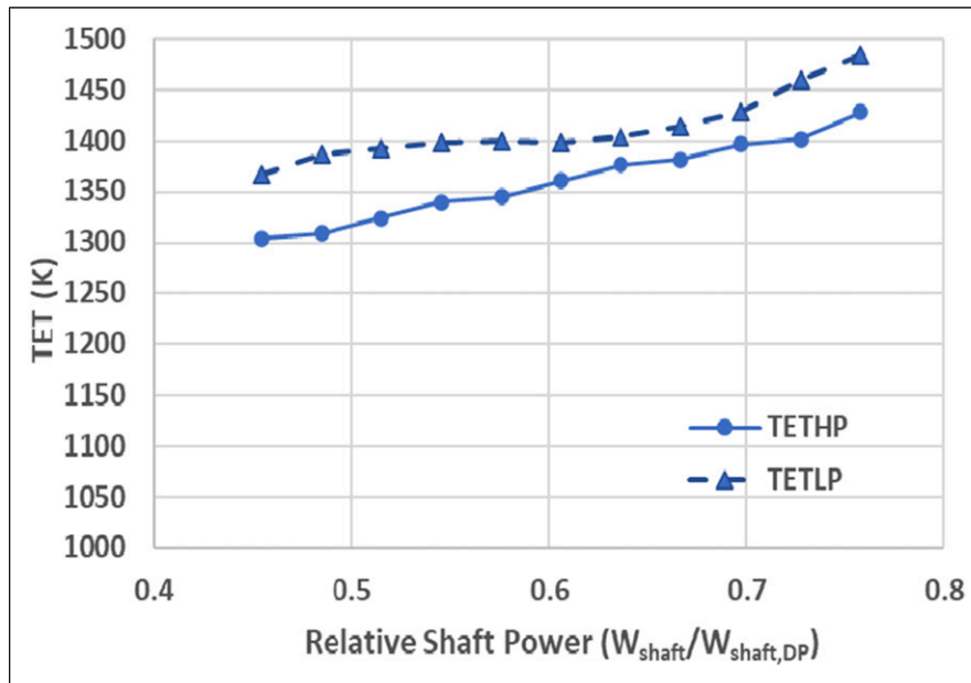
Figure 25. TETs varying with relative shaft power ( T_{amb} = 5^\circ\text{C} & P_{amb} = 0.7 atm).
