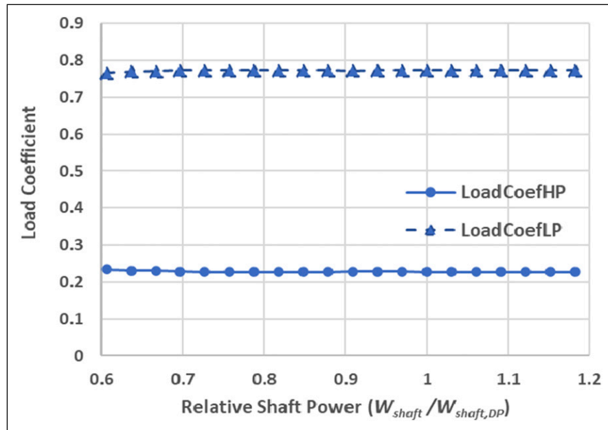
Figure 15. Load coefficients versus relative shaft power ( T_{amb} = 15^{\circ}\text{C} & P_{amb} = 1 \text{ atm} ).
