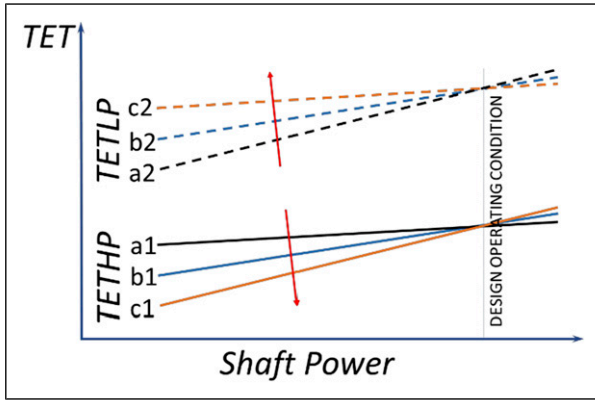
Figure 6. Off-design control schedule – TETHP & TETLP varying with shaft power.
