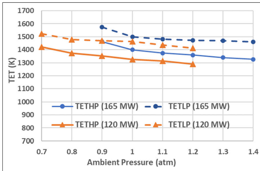
Figure 21. TET varying with ambient pressure ( T_{amb} = 288.15 K).
