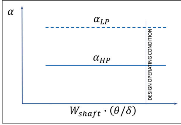
Figure 7. Load coefficients versus corrected shaft power.
