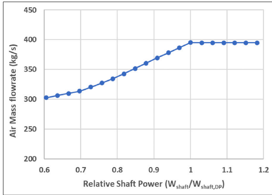
Figure 14. Air flow rate versus relative shaft power ( T_{amb} = 15^{\circ}\text{C} & P_{amb} = 1 \text{ atm} ).
