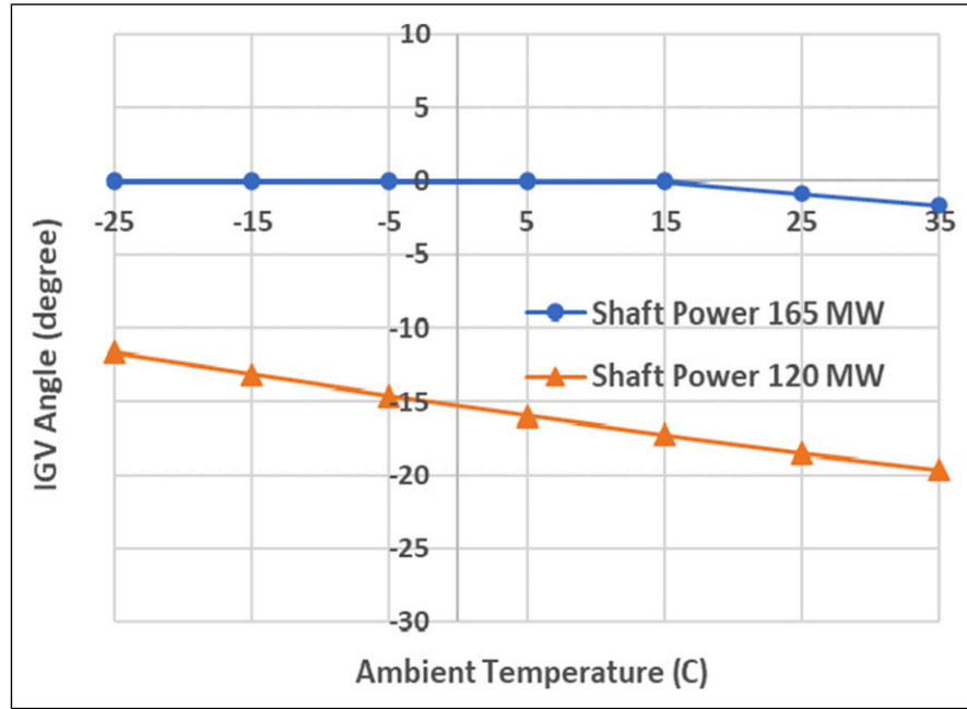
Figure 18. IGv angle versus ambient temperature ( P_{amb} = 1 \text{ atm} ).
