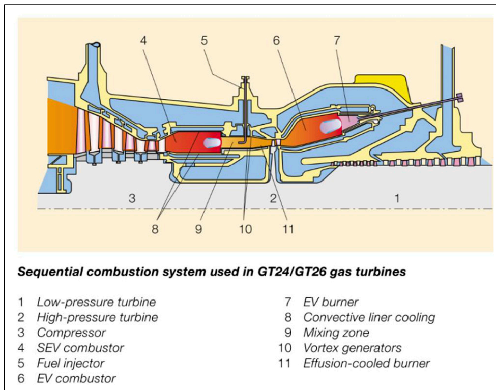
Figure 2. GT24/GT26 gas turbines. 9,10
