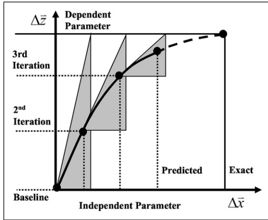
Figure 5. Newton Raphson iterations.
