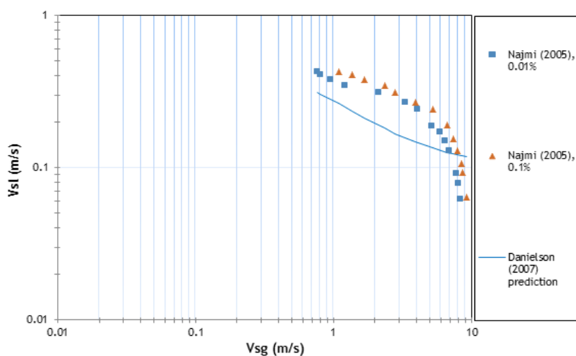
b) Tests of 4 inch pipe with sand nominal size of 300 \mu\text{m}
