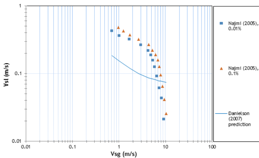
a) Tests of 2 inch pipe with sand nominal size of 300 \mu\text{m}
