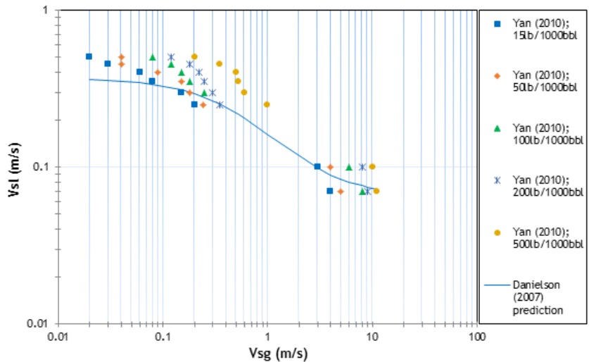
a) Tests of 2 inch pipe with sand nominal size of 200μm
