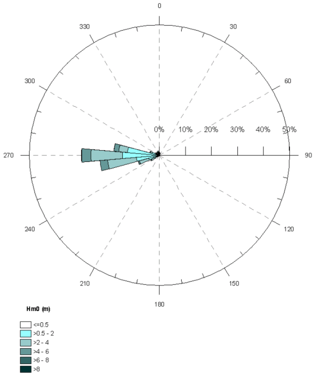
Fig. 3. Wave rose plot for the Wave Hub site between Aug 2009 and Jan 2010 [21]
