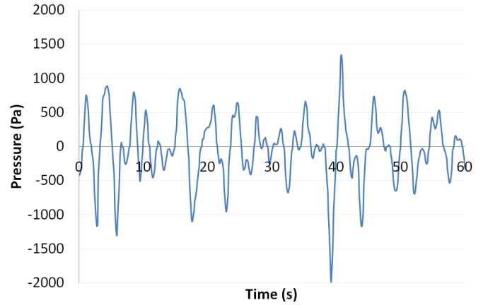
Fig. 16. Pressure plot for a scaled Breitschneider derived irregular wave with a significant wave height of 4.5m and a peak period of 12 s.
