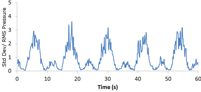
Fig. 14. Standard deviation of the total pressure measurements divided by the RMS pressure for a wave of 12s period and 1.8 \text{ m}^3/\text{s} flow rate.
