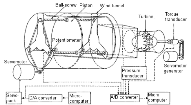
Fig. 2. Test rig using a piston [7].
