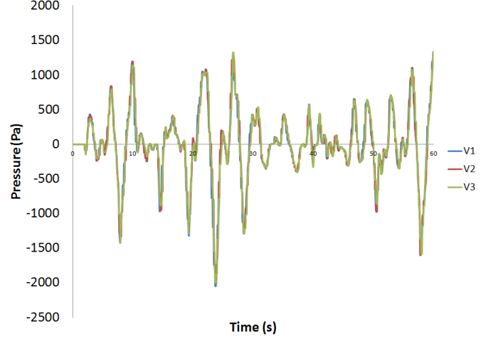
Fig. 15. Pressure plot for a scaled Pierson-Moskowitz derived irregular wave with a wind speed of 15.4 m/s.
