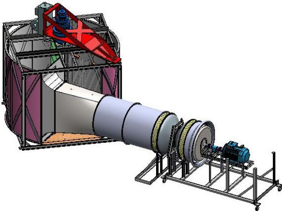
Fig. 4. CAD drawing of PWG test facility.
