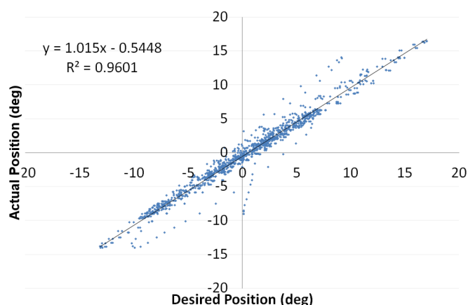
Fig. 17. Accuracy for a Pierson-Moskowitz wave.
