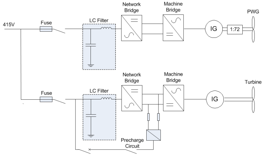
Fig. 7. Single line diagram.
