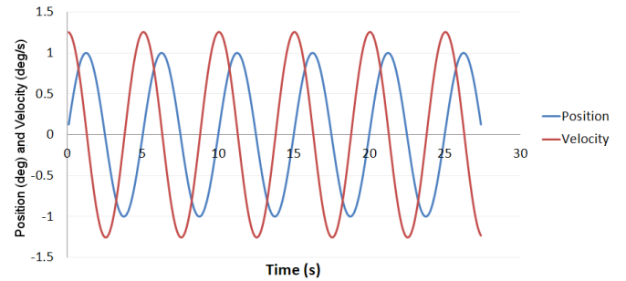
Fig. 8. Phase relationship between position and velocity.
