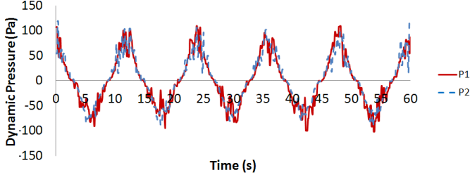
Fig. 13. Dynamic pressure measurements for a wave of 12s period and 1.8 \text{ m}^3/\text{s} flow rate.
