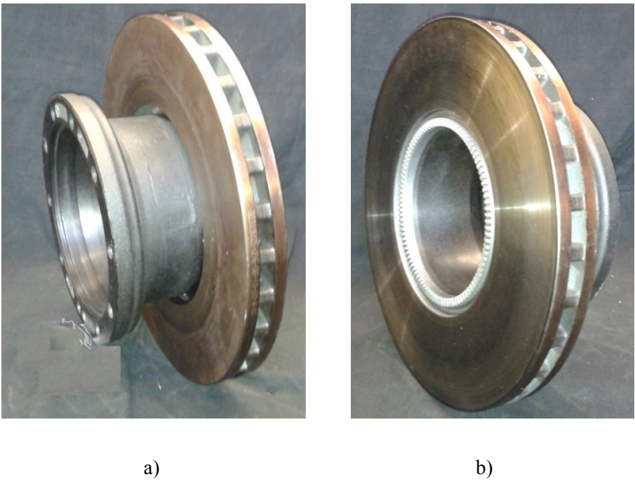
Figure 1: Brake disc analysed: a) Outboard view; b) Inboard view
