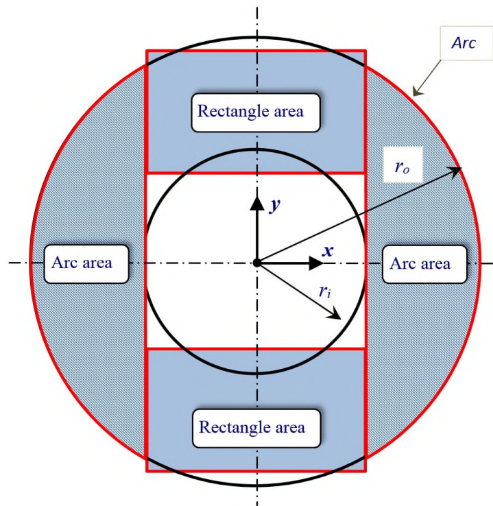
Figure 3: Partition of the disc friction surfaces into simplified geometry areas (not to scale)
