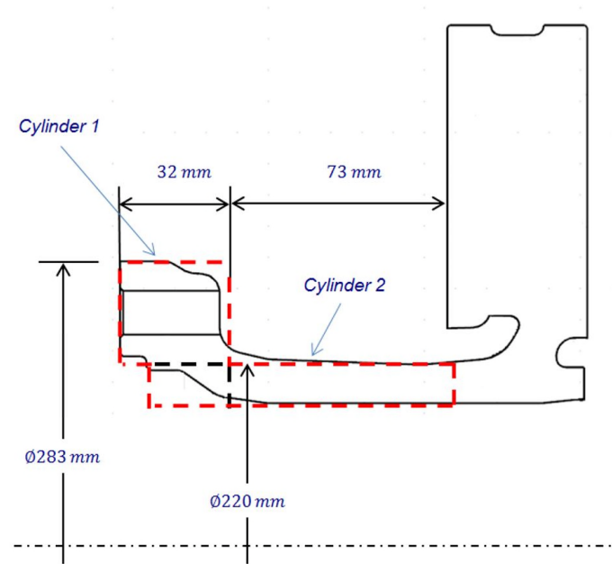
Figure 9: Simplified hat geometry
