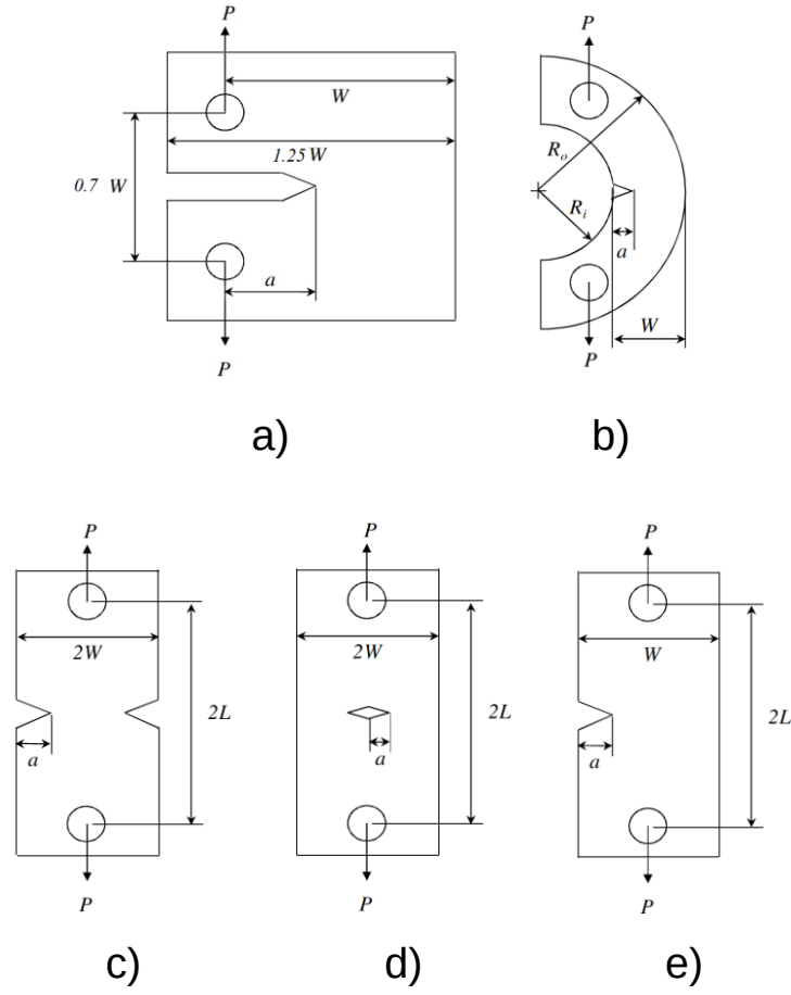
Fig. 3. Schematic illustration of specimen geometries (a) C(T), (b) CS(T), (c) DEN(T), (d) M(T), (e) SEN(T)
