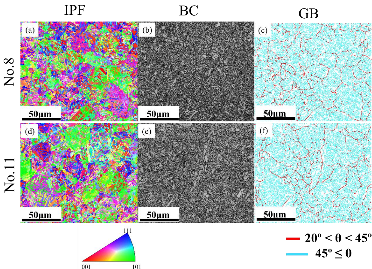
Figure 9. Inverse pole figures (IPF), band contrast maps, and grain boundary maps corresponding to the orthogonal testing numbers (a–c) No. 8; (d–f) No. 11.
