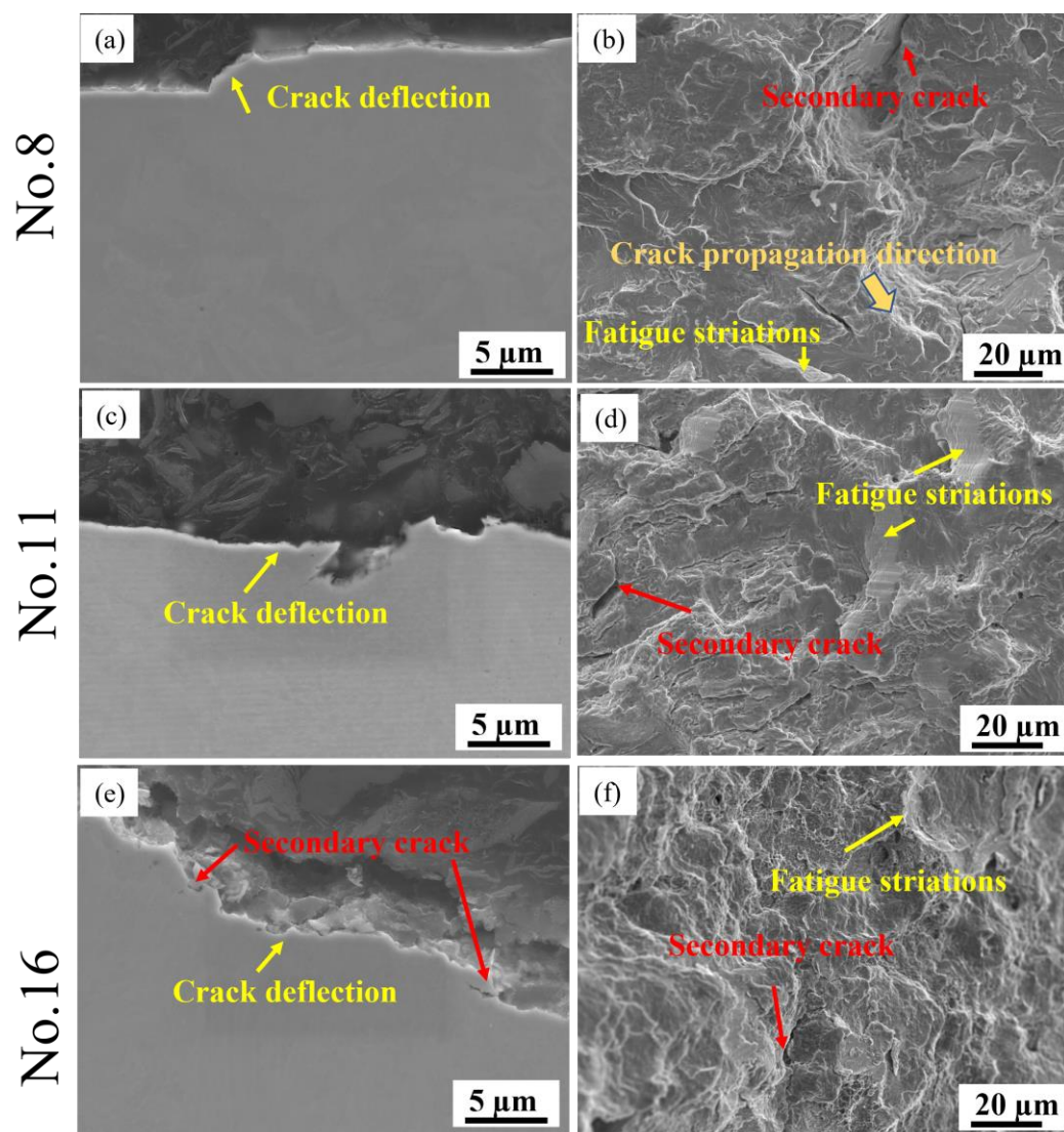
Figure 12. Fracture observation of testing specimens: (a,b) No. 8; (c,d) No. 11; (e,f) No. 16.
