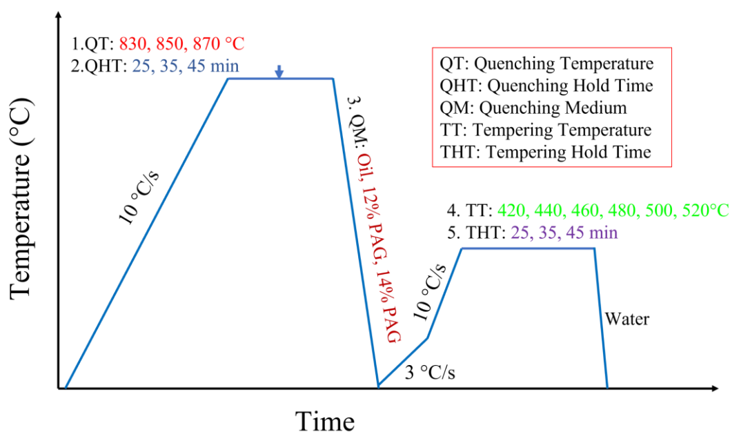
Figure 1. Diagram showing the factors considered at each stage of the heat treatment cycles.
