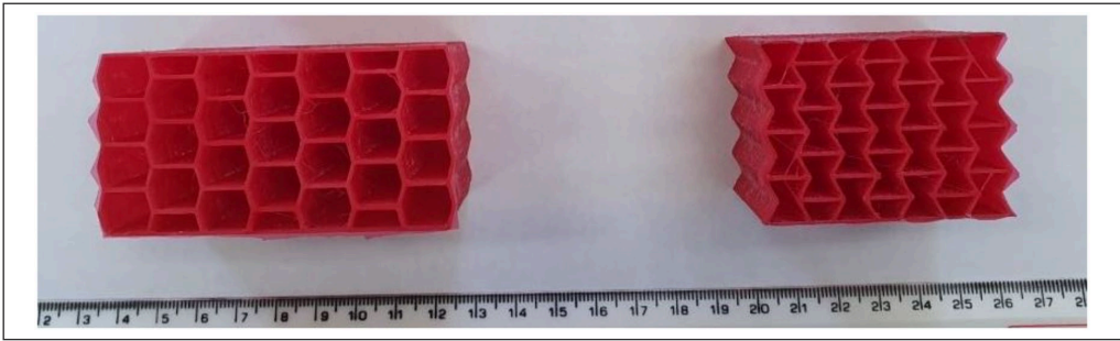
Figure 5. Example of salient honeycomb and re-entrant of shock tube samples post experiment.
