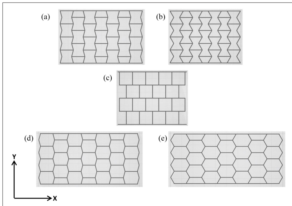
Figure 1. Cellular view of 3D printed structures comprising of: (a) -ve 15^\circ re-entrant cells, (b) -ve 30^\circ re-entrant cells, (c) 0^\circ rectangle cells, (d) +ve 15^\circ honeycomb cells and (e) +ve 30^\circ honeycomb cells. All samples were loaded in the negative Y-Axis.
