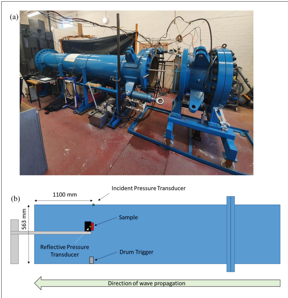
Figure 3. (a) Cranfield University Shock tube in an open position and (b) diagram of experimental setup (not to scale).
