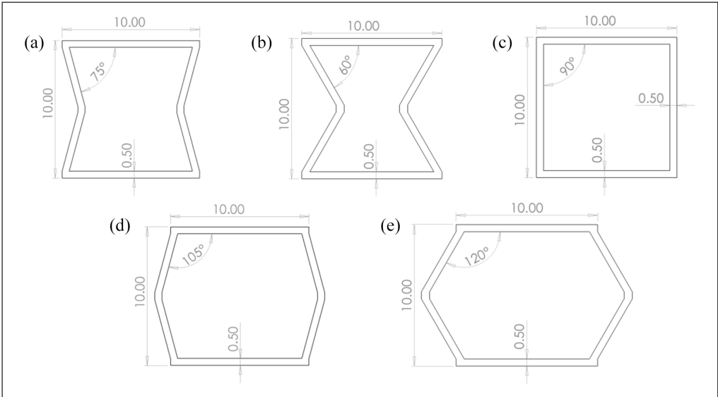
Figure 2. Individual cell dimensions for: (a) –ve 15° re-entrant cells, (b) –ve 30° re-entrant cells, (c) 0° rectangle cells, (d) +ve 15° honeycomb cells and (e) +ve 30° honeycomb cells.
