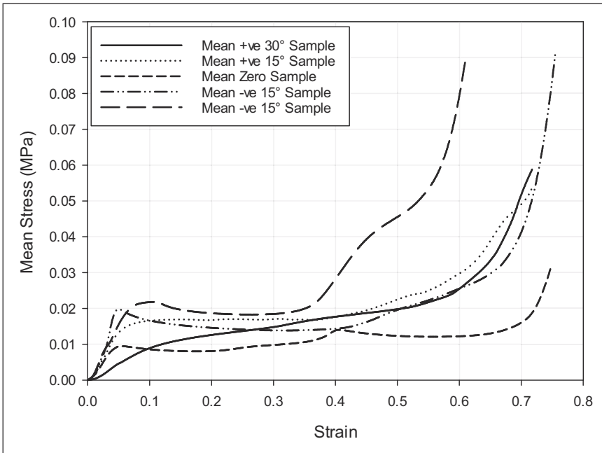
Figure 4. Mean stress-strain response of 3D printed pliable honeycomb samples (all geometries) acquired through the static compression test.
