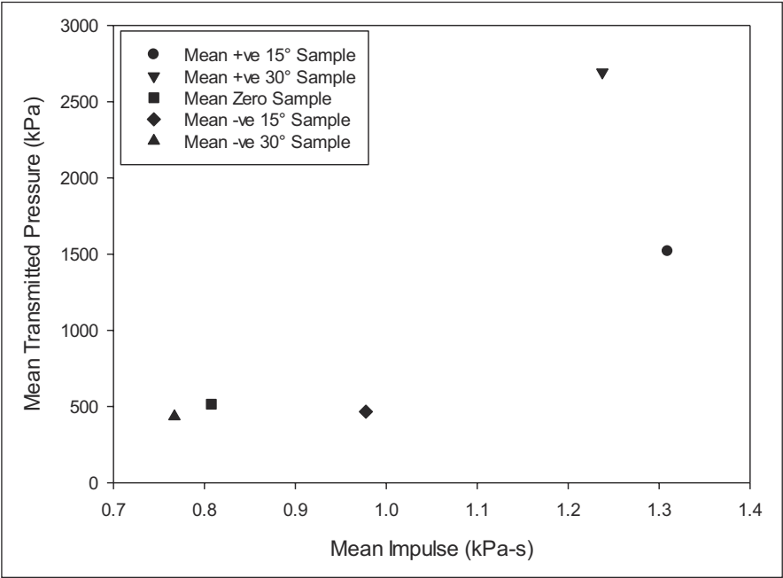
Figure 10. Mean peak transmitted pressure versus impulse response of tested structures normalised about relative density.
