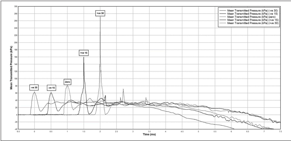
Figure 7. Mean transmitted Pressure-Time profiles for each design tested. Profiles have been offset from each other by 0.5 ms to aid readership. Full colour version normalised about 0 ms is available in Supplemental Information B.
