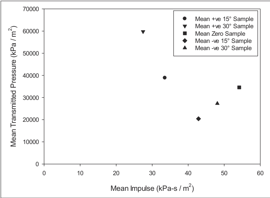
Figure 9. Mean peak transmitted pressure versus impulse response of tested structures normalised about surface area.
