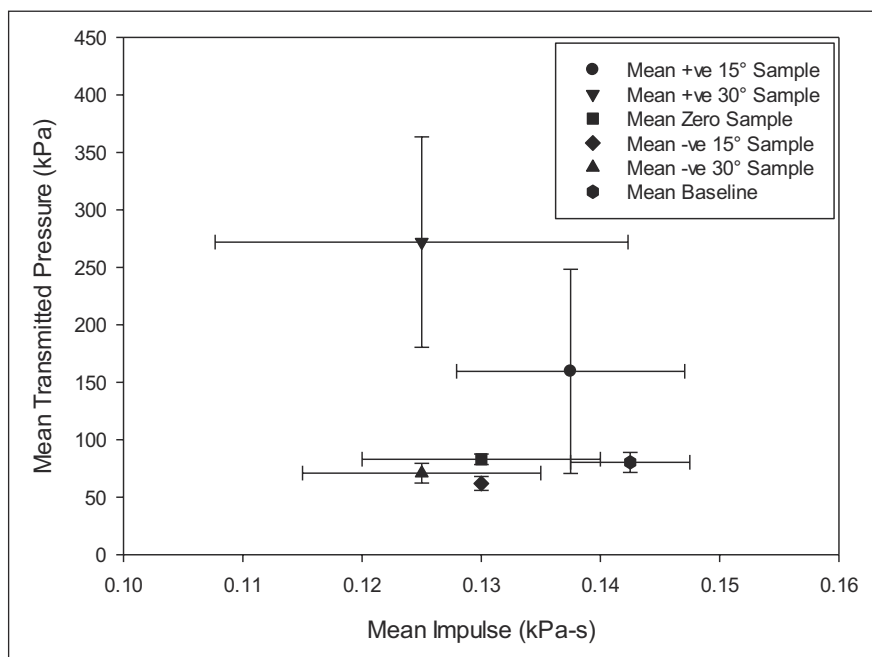
Figure 8. Mean peak transmitted pressure versus impulse response of tested structures with error provided by standard deviation.
