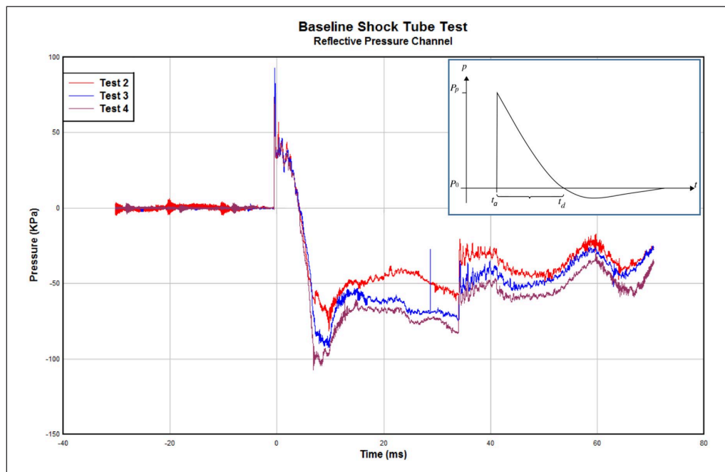
Figure 6. Raw Pressure-time measurements of baseline data where the sample response is similar in the positive phase. Test 1 omitted due to translation in the Y-axis due to sensor movement. Example of Friedlander curve provided for reference of typical behaviour.
