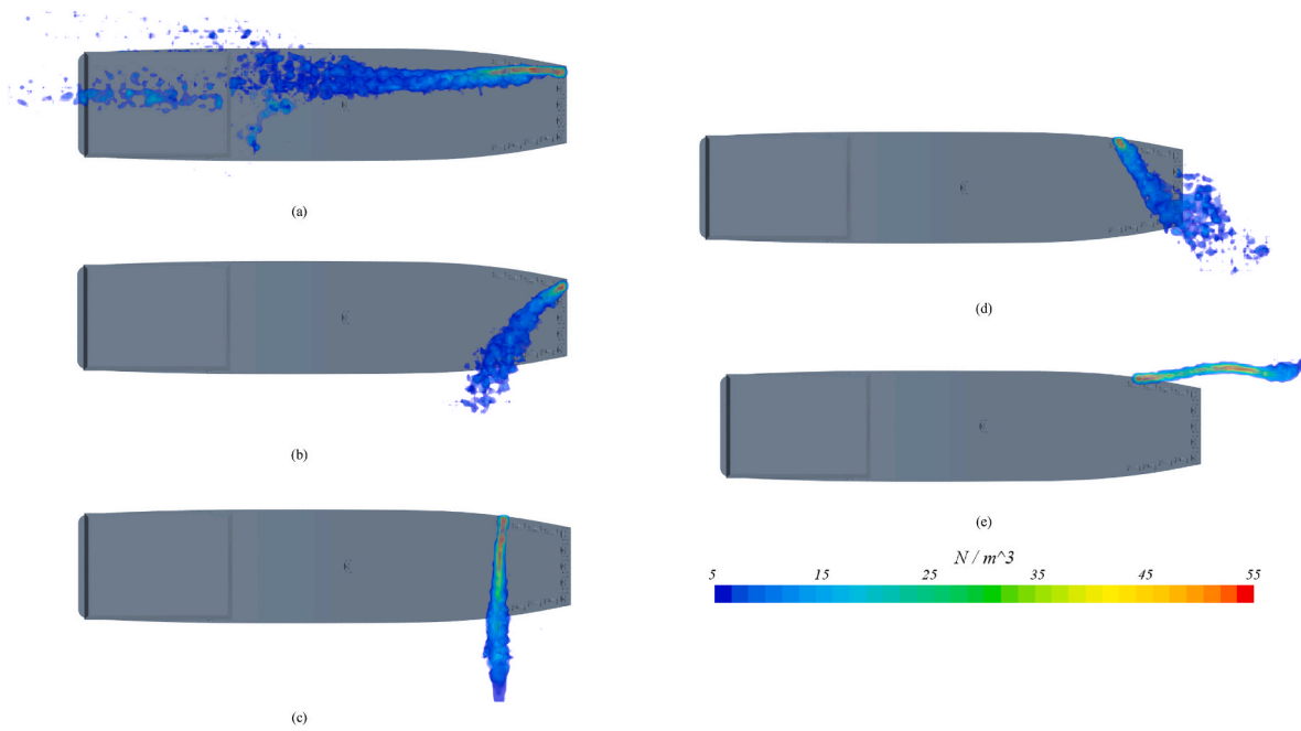
Fig. 12. Comparison of virus distribution with different wind directions; plan view and V = 1 m/s: (a) \theta = 0^\circ , (b) \theta = 45^\circ , (c) \theta = 90^\circ , (d) \theta = 135^\circ , (e) \theta = 180^\circ .
