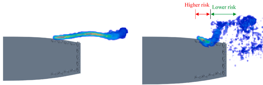
Fig. 20. Comparison of virus transmission without (Left Panel) and with (Right Panel) motions in following seas.
