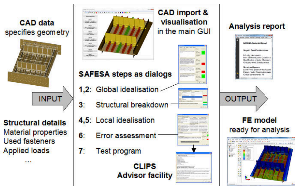
Figure 3 FE idealisation using the SAFESA advisory system
