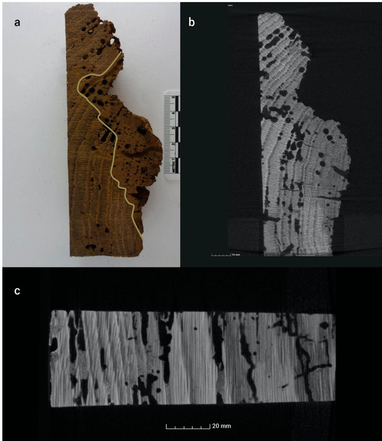
Figure 6. Images of Block 1b (surface photograph and CT slices). In Figure 6(a), the boundary has been drawn on (by eye), distinguishing (i) the area of degrading wood, lacking some structure (here, the right-hand side of the block) from (ii) the better condition, sound wood (here, the left-hand side of the block). Note that Figure 6(b) is a 'slice' from within Block 1b, and hence the holes are not identical to those observed in the surface image.
